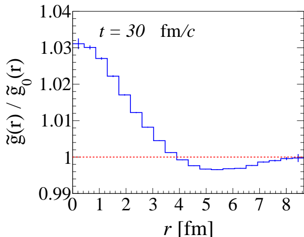
FIG. 13. (Color online) Pair correlation function at t = 30 fm/c for a system initialized inside the “quark-hadron” spinodal region (at baryon number density n_B = 3.0 n_0 and temperature T = 1 MeV), calculated within the parallel ensembles method; the results are averaged over N_{\text{ev}}^{(\text{parallel})} = N_T \times N_{\text{ev}} = 25,000 events. Spontaneous spinodal decomposition leads to a formation of two coexisting phases: a “less dense” and a “more dense” nuclear liquid. The increased relative concentration of particles in the “more dense” phase results in an elevated normalized pair correlation at small distances. The correlation is exactly the same as shown on the rightmost panel in Fig. 9. See text for more details.
