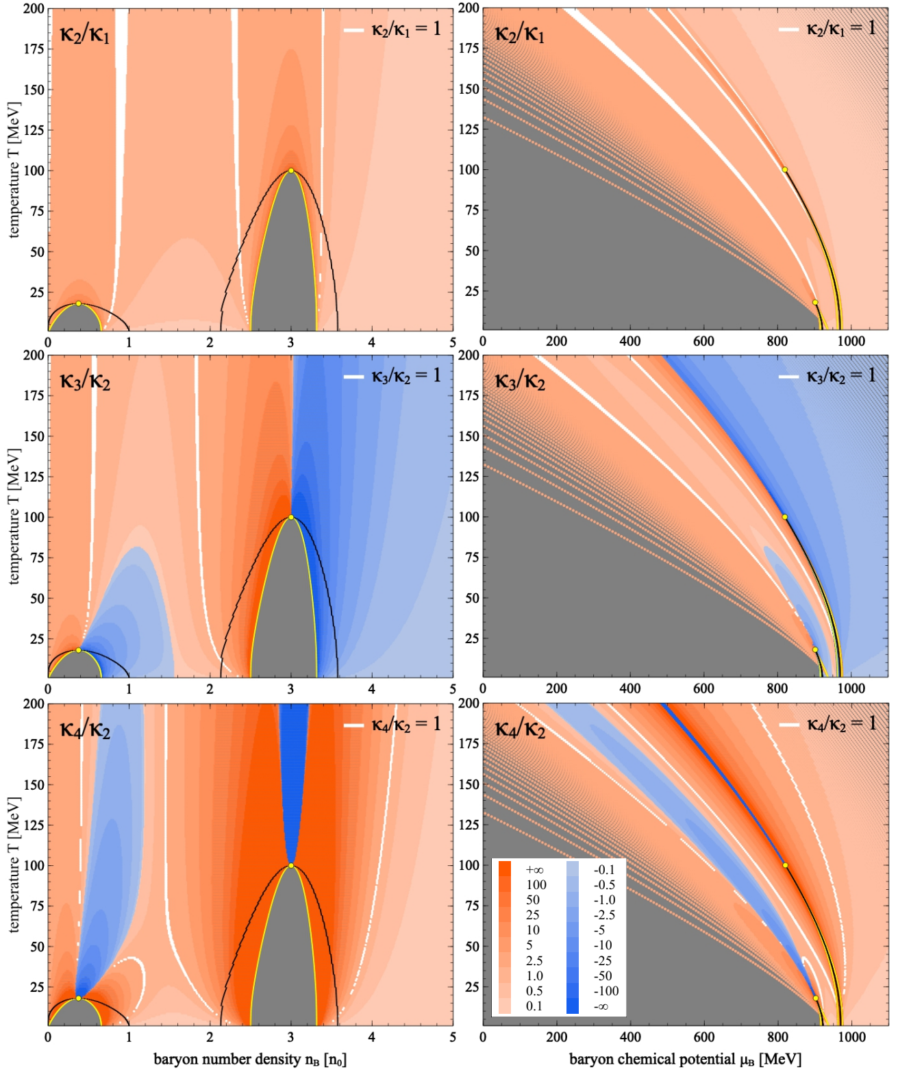
FIG. 5. Contour plots of cumulant ratios \kappa_2/\kappa_1 (upper row), \kappa_3/\kappa_2 (middle row), and \kappa_4/\kappa_2 (lower row) in both T - n_B and T - \mu_B plane (left and right column, respectively), for the EOS identified by the fourth (IV) set of characteristics listed in Table I. Black lines denote coexistence regions, while yellow lines denote spinodal regions; critical points are indicated with yellow dots. White regions correspond to values of cumulant ratios close to the Poissonian limit, \kappa_i/\kappa_j = 1 \pm 0.03 . Grey color signifies regions of the phase diagram in which either the cumulant calculation is invalid (left column: inside the spinodal region, which is unstable), or where data has not been produced (right column: regions with extremely small values of the baryon number density n_B ). The legend entries denote upper (lower) boundaries of ranges of positive (negative) values of cumulant ratios.
