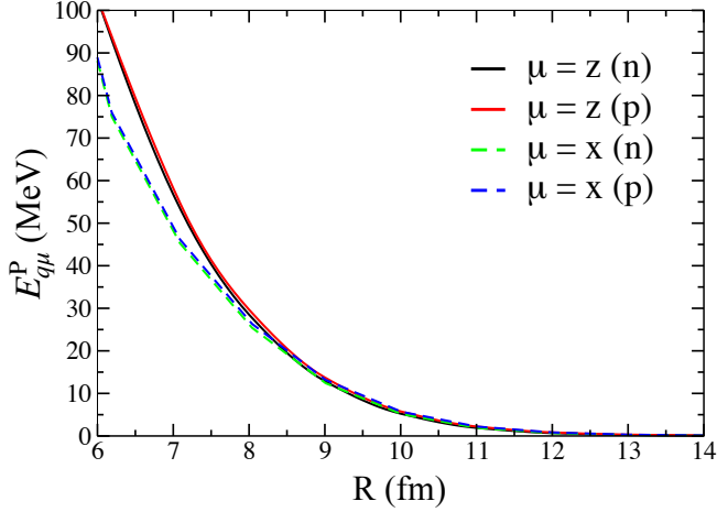
FIG. 4. Proton and neutron Pauli energy in ^{40}\text{Ca}+^{40}\text{Ca} computed from DCFHF using Eq. (12) and summing over spin, E_{q\mu}^P = \sum_{s_\mu} E_{qs_\mu}^P . The solid and dashed lines are obtained with the quantization axis \mu = z and x , respectively.
