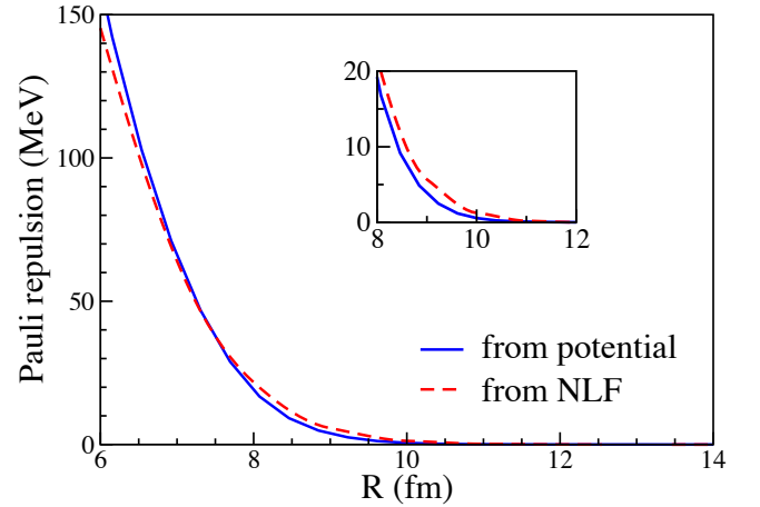
FIG. 5. Pauli repulsion in ^{40}\text{Ca}+^{40}\text{Ca} . The solid line is obtained from the potential difference V^{\text{DCFHF}} - V^{\text{FHF}} . The dashed line is the sum of neutron and proton net PKE from Eq. (13) with \mu = z spin quantization axis. The inset shows the same quantities in the barrier region.
