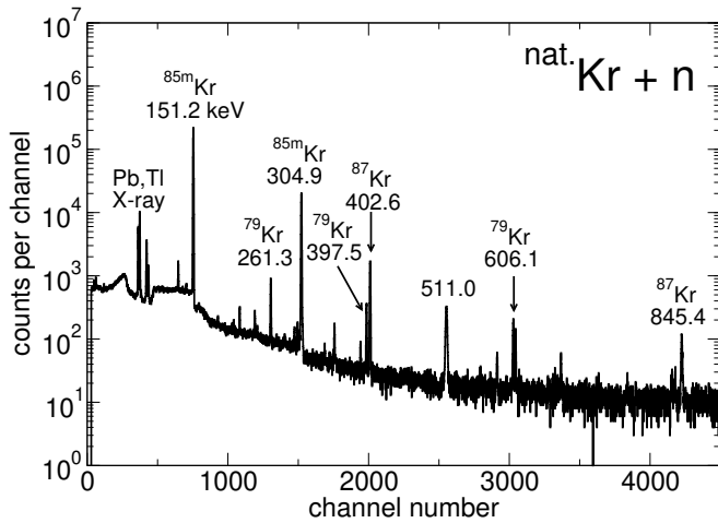
FIG. 8. \gamma -ray spectrum obtained by counting sphere #43 activity for 1872 s, starting 9007 s after end of irradiation A with an unshielded HPGe detector. The photo-peaks from the decay of the activated \text{Kr}(n, \gamma) isotopes are labeled in keV.
