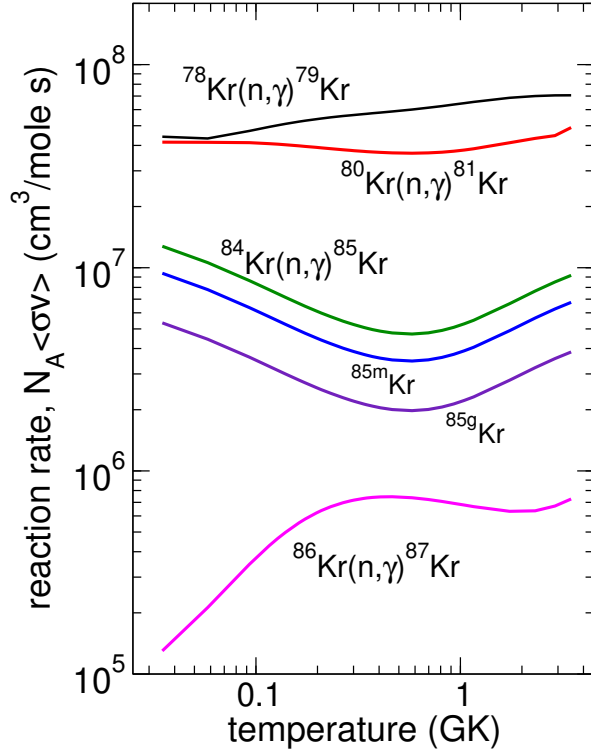
FIG. 17. Astrophysical reaction rates for (n, \gamma) reactions on Kr isotopes calculated with the MACS's of Table XII.
