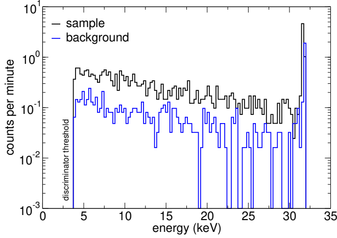
FIG. 14. Sample (upper histogram) and background (lower) \beta -spectra for measurement 1. Only a fraction of the particle decay energy (687 keV) is released within the counter before they reach its wall. Events with energies greater than 33 keV are recorded as saturated events in the last MCA channels and are included in the ^{85}\text{Kr} activity analysis.
