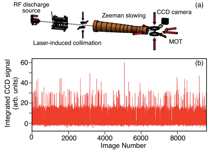
FIG. 13. (a) Schematic of the ATTA atomic beamline. Atoms (dotted line) travel from left to right, starting at the radio-frequency discharge source, passing through laser-induced collimation and Zeeman slowing stages, and ending in the MOT where they are imaged by a CCD camera. (b) Integrated CCD camera signal (divided by 1000) over a region of interest during the ^{81}\text{Kr} trapping cycles over the course of measuring the Kr gas sample (irradiation B) displayed vs. time. Zero-, one- and two- ^{81}\text{Kr} atom trapping events are observed.
