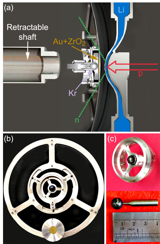
FIG. 3. (a) Diagram of the Liquid-Lithium Target (LiLiT) and activation target assembly. The ( \approx 1.5 mA, \approx 9 mm full width) proton beam (open red arrow) impinges on the free-surface lithium film (blue) (see [24] for details). The Kr-filled sphere (see text) and Au foil are positioned in the outgoing neutron cone (green dotted lines) in a vacuum chamber separated from the LiLiT chamber. The retractable shaft (at left) is used to load and unload rapidly the target assembly. (b) Photograph of the Kr gas sphere mounted in an aluminum circular frame on the center line of the chamber. A 0.5 mm thick pure Al plate (displaced to the bottom of the photograph to unveil the sphere) holding the Au monitors and a ZrO 2 thin (parasitic) target covers the Kr gas sphere. (c) Ti sphere (see [33] for details) used to contain the pressurized Kr gas for irradiation and the sphere holder for irradiation at SARAF-LiLiT.
