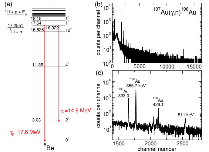
FIG. 5. (a) Part of the ^8\text{Be} energy level scheme. The two high energy gammas at 14.6 and 17.6 MeV are shown in red. See [23] for more details. (b) Spectrum of the ^{196}\text{Au} decay from the ^{197}\text{Au}(\gamma,n)^{196}\text{Au} reaction in a Au monitor foil for the under threshold run (irradiation B). (c) Zoom in on the relevant photo-peaks in the spectrum.
