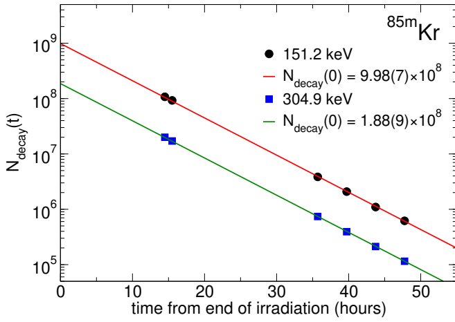
FIG. 11. The number of ^{85m}\text{Kr} decaying via \beta^- calculated from the \gamma photo-peak at 151.2 keV (75.2(5)% intensity), and via IT calculated from the \gamma photo-peak at 304.9 keV (14.0(3)% intensity). The measured ratio is 0.188(9) in good agreement with the intensity ratio 0.186(4) in [49] (see table II).
