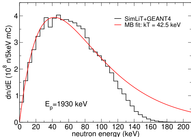
FIG. 6. Simulated neutron spectrum (black histogram) impinging on the Kr, \frac{dn_{sim}}{dE_n} . Also shown is a fit to Maxwell-Boltzmann (MB) distribution (red curve) E_n e^{-\frac{E_n}{kT}} at 42.5 keV in the range of 0-120 keV.
