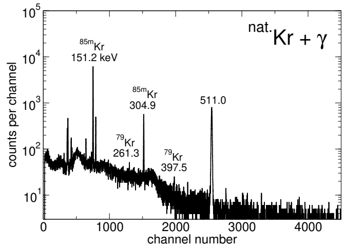
FIG. 9. \gamma -ray spectrum obtained by counting sphere #59 activity for 7208 s, starting 2844 s after end of irradiation B with a shielded HPGe detector. The photo-peaks from the decay of the activated \text{Kr}(\gamma, n) isotopes are labeled in keV.
