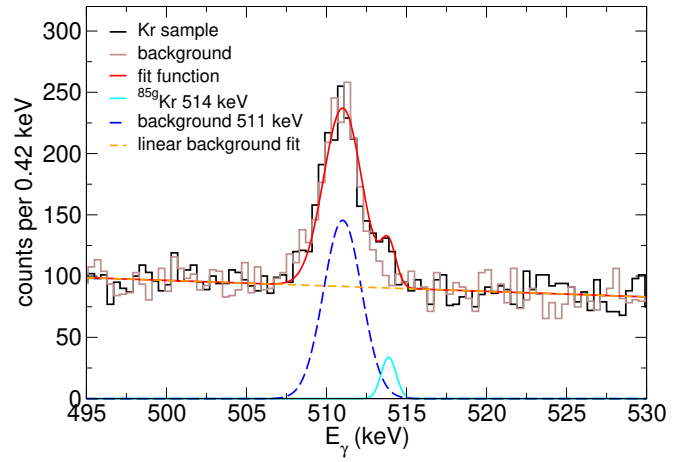
FIG. 15. 514 keV photo-peak next to the 511 keV photo-peak for the irradiation above neutron production threshold. This region in the spectrum was fitted to 2 Gaussians and a linear background. The amount of ^{85g}\text{Kr} produced during the irradiation was determined from this fit (see table V).
