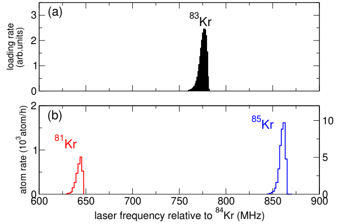
FIG. 12. Typical spectrum of the trap capture rate of ^{81,83,85}\text{Kr} versus laser frequency shift (relative to a reference transition in stable ^{84}\text{Kr} ) measured for an atmospheric Kr sample ( ^{81}\text{Kr}/\text{Kr} = 9.3 \times 10^{-13} [39]). Figure adapted from [52], see text.
