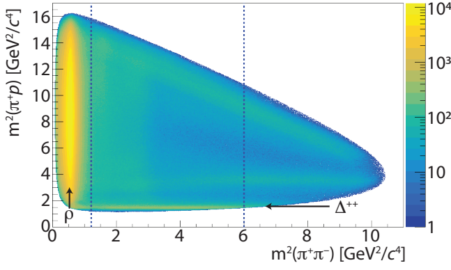
Figure 2. Dalitz plot of products of the reaction \gamma p \rightarrow \pi^+ \pi^- p . Candidates between dashed lines are selected. Data shown are not efficiency corrected.
