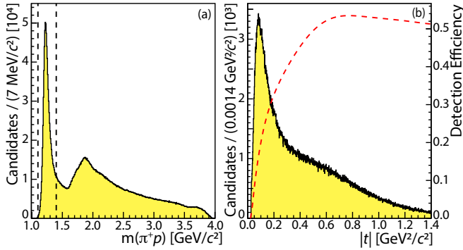
Figure 3. (a) The \pi^+ p invariant mass distribution of events satisfying all selection criteria. In addition to the \Delta^{++} , excited states around 1.9 GeV/c 2 are visible. (b) The distribution of |t| for candidates between the dashed lines in panel (a) and the detection efficiency as a function of |t| . Data plotted are not efficiency corrected.
