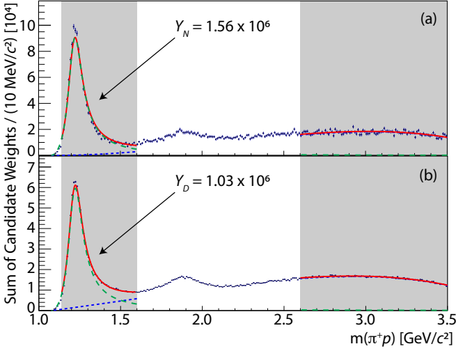
Figure 4. (color online) Fit to (a) numerator N and (b) denominator D defined in Eqs. 5b and 5a, in the extended range 0.4 \text{ (GeV}/c^2) < |t| < 1.4 \text{ (GeV}/c^2) . The \Delta^{++} component is shown in green (dashed), polynomial background in blue (dotted), and total fit in red. Data are fit in the shaded regions only, the integral of the green (dashed) curve in the lower shaded region is used to determine the yields Y_N and Y_D .
