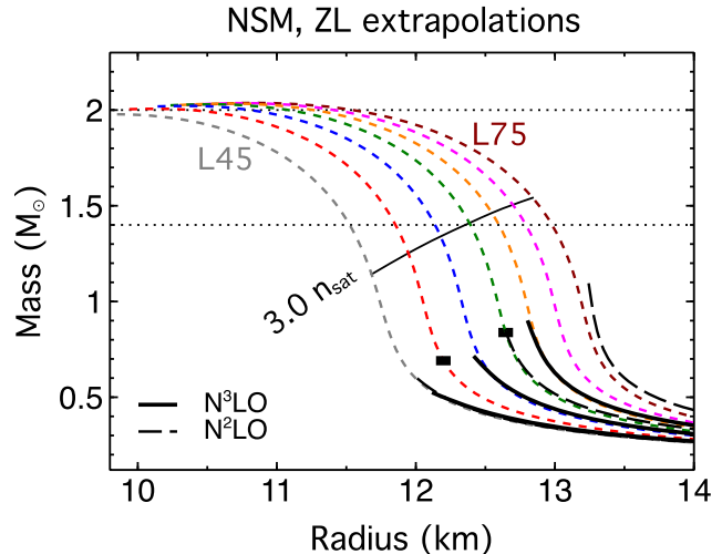
FIG. 5. M-R relations for NSM EOSs extrapolated to n_B \geq 2.0 n_{\text{sat}} beyond the \chi\text{EFT} calculations using the ZL parametrization [60]; the thin black line indicates where the NS central densities are 3.0 n_{\text{sat}} . From left to right, the colored dotted curves represent L = 45 MeV to L = 75 MeV in increments of 5 MeV, and the black-solid (black-dashed) curves refer to \chi\text{EFT-N}^3\text{LO} ( \text{N}^2\text{LO} ) with \pm 1\sigma uncertainties. The L = 50 MeV (red) and L = 60 MeV (green) ZL EOSs are used in Fig. 11 because they best represent \pm 1\sigma bounds.
