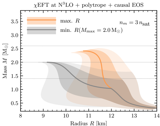
FIG. 4. Similar to Fig. 3 but obtained using the polytropic extrapolation of the \chi\text{EFT} EOS up to n_m = 3.0 n_{\text{sat}} .
