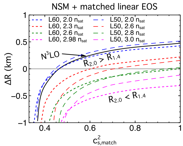
FIG. 13. Radius differences \Delta R = R_{2.0} - R_{1.4} using the ZL extrapolations with L = 50 \text{ MeV} and L = 60 \text{ MeV} joined continuously to linear EOSs at n_m between 2.0 n_{\text{sat}} and 3.0 n_{\text{sat}} .
