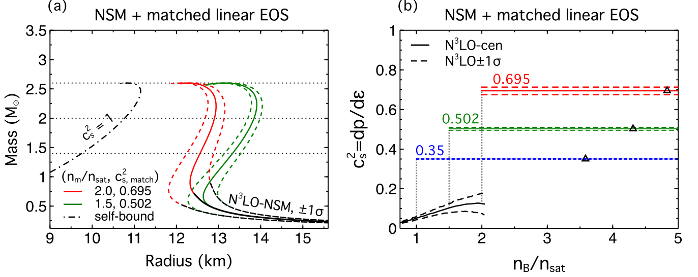
FIG. 14. Panel (a): M - R diagram for matched linear EOSs that give rise to M_{\max} = 2.6 M_{\odot} with N^3\text{LO-NSM} ( \pm 1\sigma ) applied for low densities \leq 2.0 n_{\text{sat}} . Corresponding values of n_m and c_{s,\text{match}}^2 are indicated (see also Fig. 11 (a)). Panel (b): sound speed profiles c_s^2(n_B) for N^3\text{LO-NSM} only (black-solid for the central value and black-dashed for \pm 1\sigma uncertainties), and matched linear EOSs with different values of c_{s,\text{match}}^2 associated with M_{\max} = 2.6 M_{\odot} in panel (a) (colored horizontal lines). The open triangles mark the central densities of the maximum-mass stars M_{\max} = 2.6 M_{\odot} .
