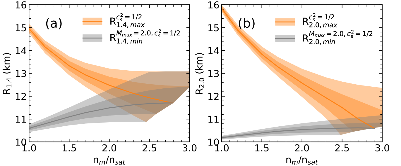
FIG. 9. Similar to Fig. 8, but assuming c_s^2 \leq 1/2 above n_B = n_m .
