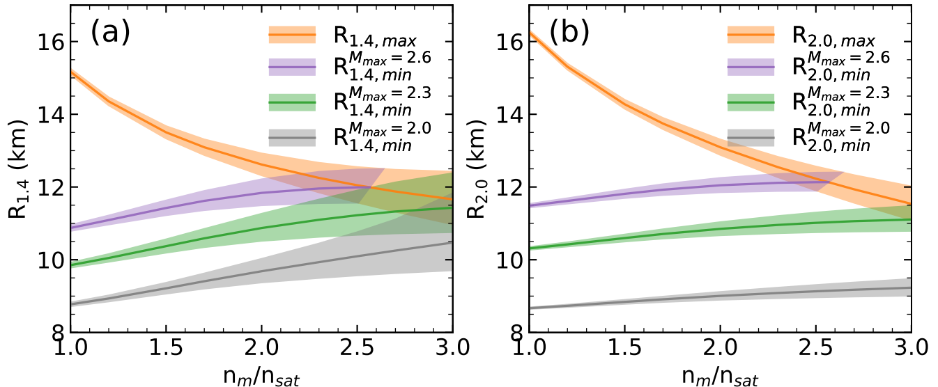
FIG. 6. Similar to Figs. 3 and 4, but displaying the minimum and maximum radii of 1.4 M_{\odot} (panel (a)) and 2.0 M_{\odot} (panel (b)) stars as a function of the matching density n_m = 1.0 - 3.0 n_{\text{sat}} . Additionally, R_{\text{min}} contours and uncertainty bands for the case M_{\text{max}} = 2.3 M_{\odot} are shown.
