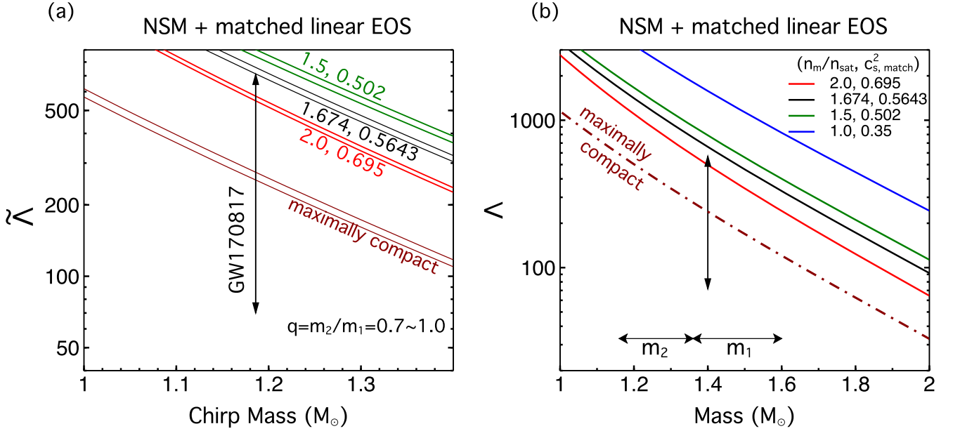
FIG. 15. \tilde{\Lambda} - M and \Lambda - M relations confronted with constraints from GW170817 [6, 7] (vertical lines with arrows), with fixed M_{\max} = 2.6 M_{\odot} as an example. Parameters for matched EOSs are the same as in Fig. 14, except for the special case with n_m = 1.674 n_{\text{sat}} (with c_{s,\text{match}}^2 = 0.5643 ), which refers to the minimum matching density that survives \tilde{\Lambda}(M = 1.186 M_{\odot}) \leq 720 .
