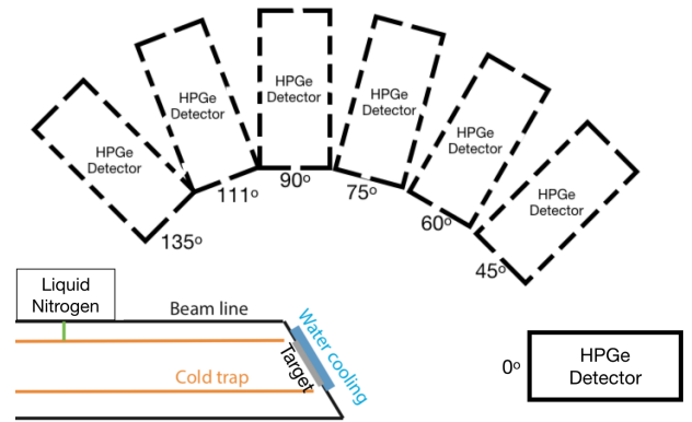
FIG. 2: Schematic of the experimental setup. It is important to note that the same HPGe detector was set on a rotating table and set to each of the angles, not seven different detectors.
