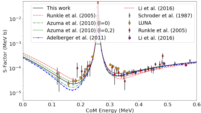
FIG. 13: R -matrix fits comparing our best fit to those performed in previous works. Our fit used a lifetime value for the 6.79 MeV excited state in ^{15}\text{O} within our measured range, \Gamma = 2.75 where the fits to the data provide good agreement with data above and below the 278 keV resonance. This plot is limited to the low energy region. The Schröder et al. data are from [8], while the LUNA data represents the measurements of [10, 13, 33, 34], the Runkle et al. data are from [14], and the Li et al. data are from [16]. Of these, the data used from Li et al. [16] are differential and were treated as such in the fitting but scaled up by 4\pi for plotting purposes. The fits from previous works come from Refs. [14–16, 31].
