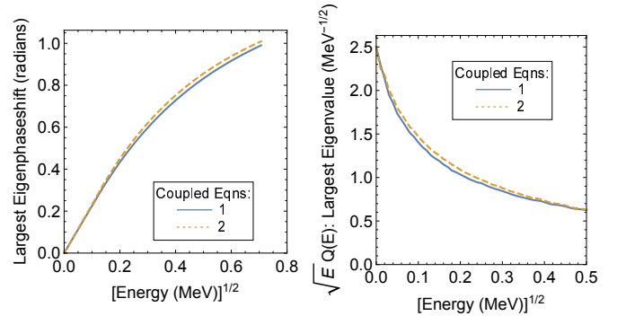
Figure 13. The largest 3n eigenphaseshift (left) and time delay (right) with the inclusion of 1 and 2 channels from a multi-channel calculation to show the effects on the low-energy behavior from non-adiabatic coupling. These results use a single Gaussian model for the nn two-body interaction with the HH basis.
