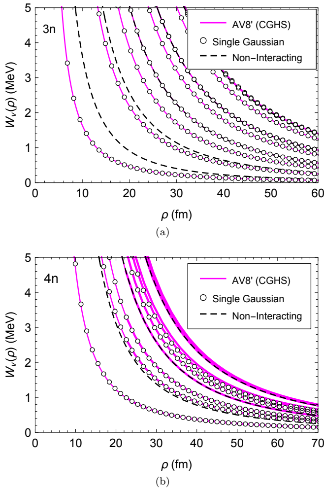
Figure 1. The lowest few adiabatic potentials for the 3n (a) and 4n (b) systems using the AV8' two-body interaction are presented with the ordering of states from bottom to top, with the lowest curve representing \nu=1 . The diagonal second-derivative non-adiabatic couplings are included. The non-interacting potentials (dashed lines) are shown to provide a qualitative picture of the amount of attraction in these systems. Also, the adiabatic potentials are compared to a single-Gaussian model (open circles) with L=0 and L=1 natural parity states for the 4n and 3n systems, respectively.
