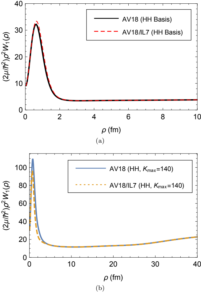
Figure 4. A comparison of the lowest adiabatic potential using the AV18 two-body interaction with and without the IL7 3N force for the 3n (a) and 4n (b) systems. There is only a significant difference for \rho < 5 fm.
