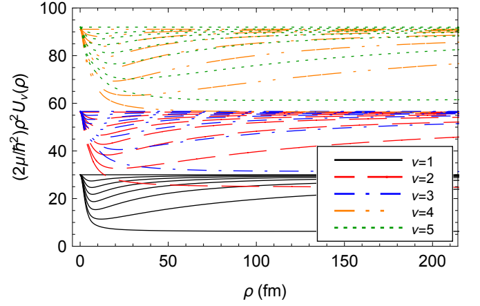
Figure 10. The lowest 5 adiabatic potentials ( \nu=1-5 ) for the 4n system for the J^\pi = 0^+ symmetry with L = 0 using a single-Gaussian potential with r_0 = 1.78 fm. The strength V_0 is tuned to give different scattering lengths from 0 to infinity with no two-body bound state. Each set of potentials represent a different s -wave scattering length in this range.
