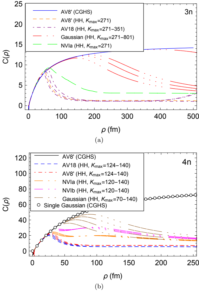
Figure 2. Plots of the dimensionless function C_\nu(\rho) \equiv (\rho/a)[\rho^2 W_1(\rho) 2\mu/\hbar^2 - l_{\text{eff}}(l_{\text{eff}} + 1)] for the 3n (a) and 4n (b) systems with \nu = 1 . According to Eq. (10), we should obtain C_\nu(\rho \rightarrow \infty) = C_\nu , where C_\nu is the coefficient listed in Table II. We observe the slow convergence for large \rho of the adiabatic potentials calculated using the HH basis, with increasing values of K_{\text{max}} indicated as higher curves for each nuclear model that tends towards the most converged CGHS calculation. However, it has to be noted that where the convergence is achieved, the functions C_\nu(\rho) obtained for the different interactions used in this work almost collapse onto a single curve. Noticeably, this happens already for fairly small values of \rho , showing that the adiabatic potentials are already universal at moderate values of the hyperradius. In fact, the limit C_\nu(\rho) = C_\nu is reached only for \rho > 500 fm.
