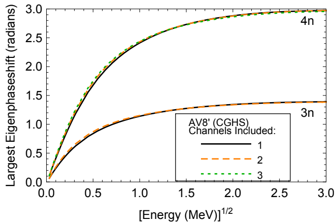
Figure 15. Largest eigenphaseshift for the 3n and 4n systems for the inclusion of up to 3 channels using the AV8' interaction with the CGHS basis. The lowest curve is the single-channel results while the second lowest and highest curves are the resultant eigenphaseshifts from a multichannel calculation for 2 and 3 channels, respectively. The eigenphaseshift is only slightly modified for energies less than 1 MeV, providing further support the adiabatic approximation is sufficient in describing the low-energy behavior.
