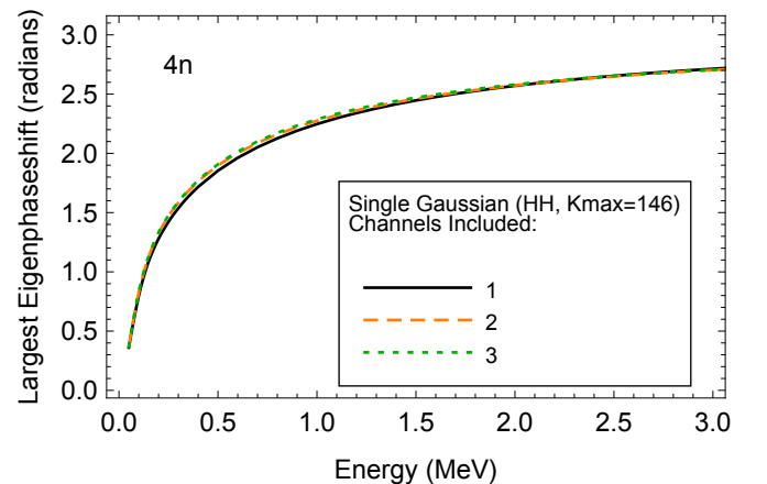
Figure 14. The 4n phaseshift in the lowest adiabatic potential with the inclusion of multiple channels an a multi-channel calculation to show the effects on the low-energy behavior from channel coupling. These results use a single Gaussian model for the nn two-body interaction with the HH basis.
