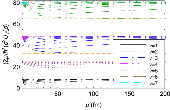
Figure 9. The lowest 7 adiabatic potentials ( \nu=1-7 ) for the 3n system for the J^\pi = \frac{3}{2}^- symmetry with L = 1 using a single-Gaussian potential with r_0 = 1.78 fm. The strength V_0 is tuned to give different scattering lengths from 0 to infinity with no two-body bound state. Each set of potentials represent a different s -wave scattering length in this range with limits shown by the horizontal dashed lines representing the non-interacting limit (upper-dashed) and unitarity limit (lower-dashed). The unitarity limits are given in Table II. The set of potentials labeled by \nu=1, 2, 3 and 5 represent the potentials with the \rho^{-3} behavior as they approach the non-interacting limit and the curves labeled by \nu=4, 6 and 7 represent those that fall off faster than \rho^{-3} .
