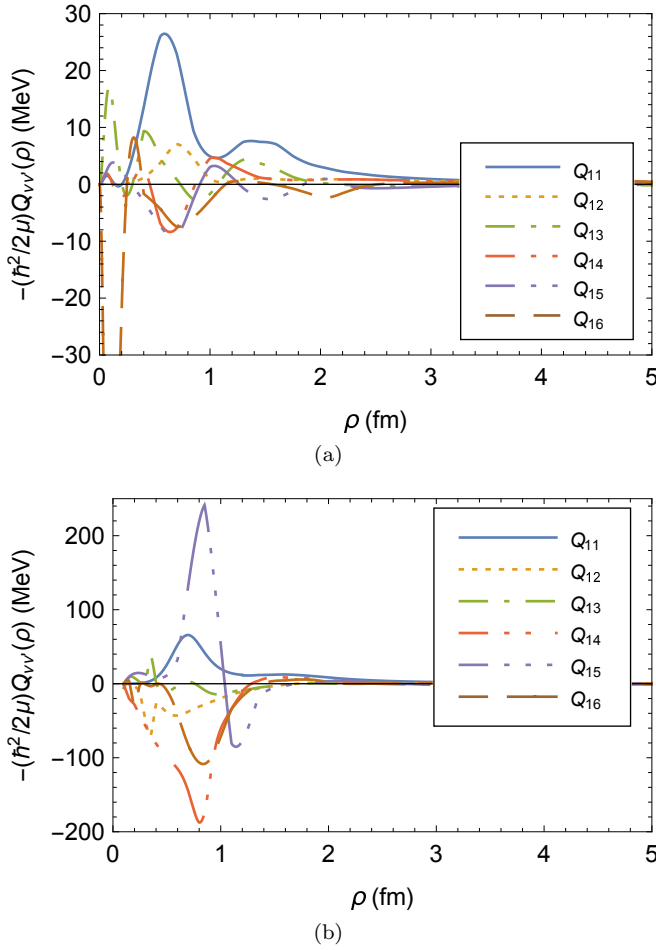
Figure 6. The second-derivative coupling matrix elements Q_{1\nu} in the lowest channel for the 3n (a) and 4n (b) systems with \nu = 1 - 6 . The coupling matrix elements are scaled by \hbar^2/2\mu .
