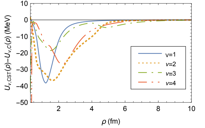
Figure 3. Difference in the lowest few 4n hyperradial potentials for L = 0 states ( \nu = 1 - 4 ) with and without the spin-orbit and tensor interactions. The differences suggest that the tensor and spin-orbit interactions provide attraction to the system at hyperradii around 0 < \rho < 5 fm.
