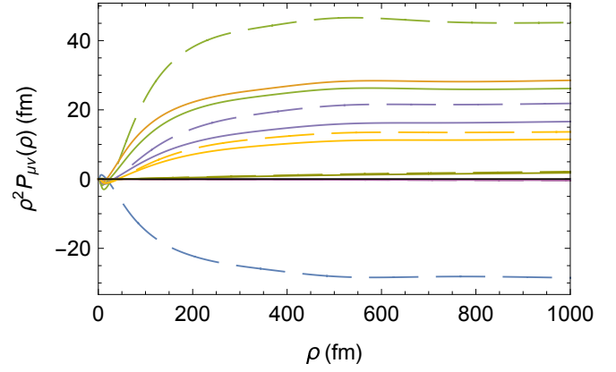
Figure 7. The first-derivative non-adiabatic matrix elements for the lowest few 3n channels are shown multiplied by \rho^2 to emphasize the long-range behavior. The solid lines are the coupling matrices to the first channel and the dashed lines are coupling matrices to the second channel (i.e. P_{1\nu} and P_{2\nu} with \nu = 1, \dots, 6 ).
