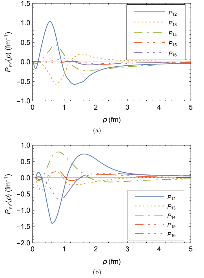
Figure 5. The first-derivative coupling matrix elements P_{1\nu}(\rho) in the lowest channel for the 3n (a) and 4n (b) systems with \nu = 2 - 6 (from Eq. (5) P_{11}(\rho) = 0 ).
