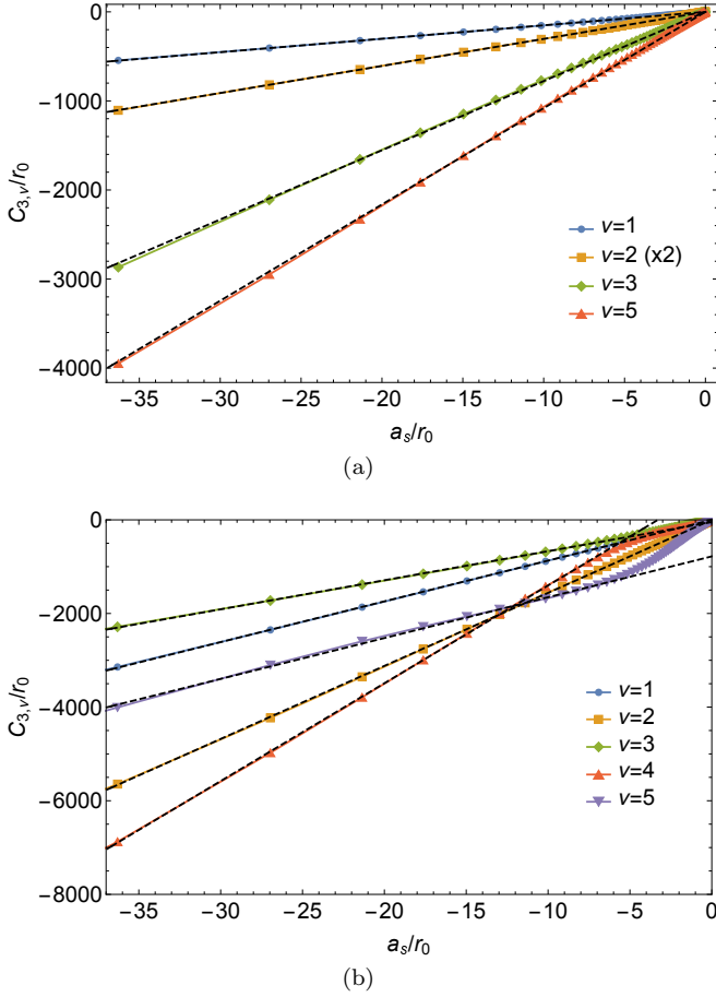
Figure 11. The scattering length dependence of the 3-body and 4-body C_{3,\nu} coefficient scaled by the range of the potential, r_0 for the lowest few potentials. In (a), the re-scaled C_{3,\nu} coefficient is shown for the 3-body case for the (\frac{1}{2})_{\frac{3}{2}}^- symmetry. The circle, square, diamond and triangle symbols represent the channels \nu = 1, 2, 3 , and 5 , respectively. The data for \nu = 2 is multiplied by a factor of 2, denoted by the label (\times 2) , in order to differentiate between the data for \nu = 1 and \nu = 2 . In (b), the re-scaled C_{3,\nu} coefficient is shown for the 4-body case for the (00)0^+ symmetry. The circle, square, diamond, upright triangle, and downward triangle symbols represent the channels \nu = 1, 2, 3, 4 , and 5 , respectively. The dashed lines are linear fits performed over the range -36 < a_s/r_0 < -10 .
