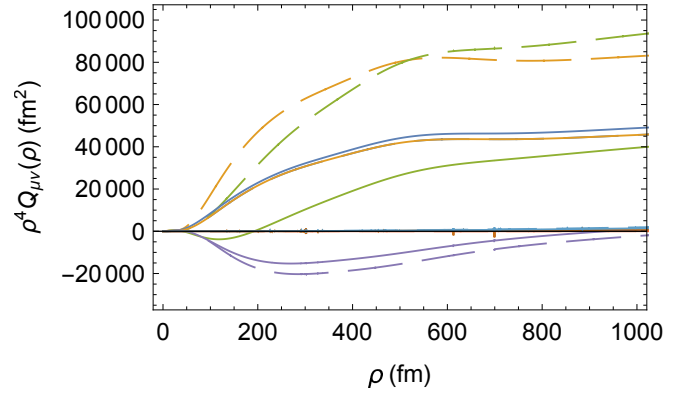
Figure 8. The second-derivative non-adiabatic matrix elements for the lowest few 3n channels are shown multiplied by \rho^4 to emphasize the long-range behavior. The solid lines are the coupling matrices to the first channel and the dashed lines are coupling matrices to the second channel (i.e. Q_{1\nu} and Q_{2\nu} with \nu = 1, \dots, 6 ).
