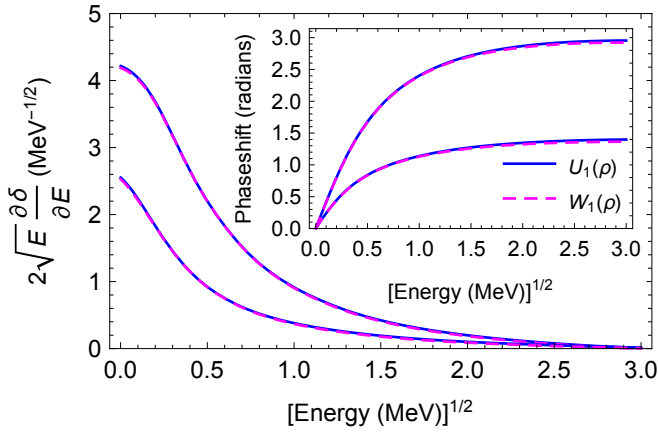
Figure 12. The elastic phaseshift(inset) and re-scaled Wigner-Smith time delay in the lowest adiabatic potential for the 3n and 4n systems with and without the diagonal second-derivative coupling term shown as dashed and solid lines, respectively. The upper curves are for the 4n system and the lower curves are for the 3n system.
