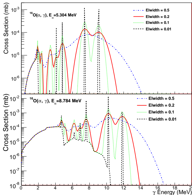
Figure 2. (Color online). Plot of ^{16}\text{O}(\alpha, \gamma) cross section versus \gamma -ray energy for two \alpha energies of 5.304 MeV and 8.784 MeV with different values of “elwidth”.
