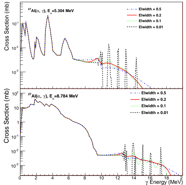
Figure 1. (Color online). Plot of ^{27}\text{Al}(\alpha, \gamma) cross section versus \gamma -ray energy for two \alpha energies of 5.304 MeV and 8.784 MeV with different values of “elwidth”.
