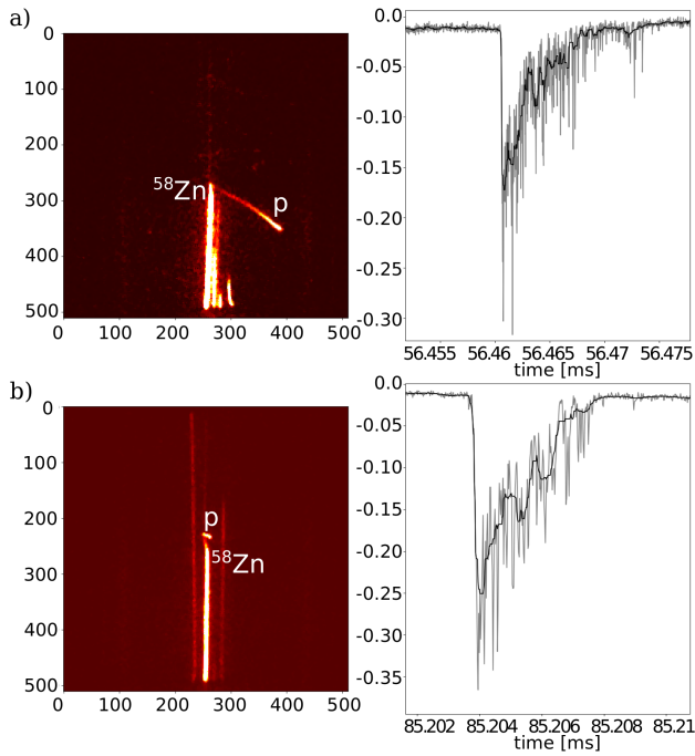
FIG. 4. (Color online) a) and b) Example CCD pictures (left) and respective fragments of the PMT signal corresponding to the proton track (right) collected during the experiment. The grey histogram shows the raw PMT signal, while the black curve is the same signal processed through a median filter. The decision on whether a proton is stopped inside the chamber or not is based on the observation of the Bragg peak in the CCD image rather than in the PMT signal because of the noise levels in the latter. See text for details.
