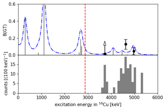
FIG. 6. (Color online) (Upper panel) B(GT) values for decay of ^{58}\text{Zn} from experiment for E_x > S_p (full circles with error bars, this work) and from QRPA calculations (see text for details) up to 6 MeV excitation energy. The grey bars show the B(GT) calculations, while the dash-dotted blue line represents the calculated B(GT) folded with 0.2 MeV-wide Breit-Wigner distributions to account for the energy resolution. The vertical dashed line shows the S_p value in ^{58}\text{Cu} . (Lower panel) Energy spectrum of \beta p from ^{58}\text{Zn} decay reported on the excitation-energy scale for comparison with the calculations. The spectrum has been corrected for the efficiency (see Fig. 5).
