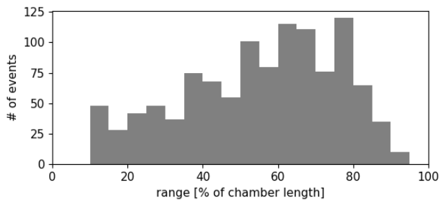
FIG. 3. Implantation profile of identified ^{58}\text{Zn} ions (events in which only a single ion entered the chamber – \sim 3\% of the total statistics). The abscissa shows the depth into the chamber along the beam direction. Only ions implanted within 10 and 90% of the chamber length were considered further in the analysis.
