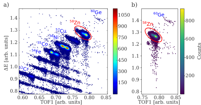
FIG. 2. (Color online) ID-plot of a) all fragments identified during the experiment and b) triggering ions. Both plots refer to the ion-optics setting optimised for ^{60}\text{Ge} . See text for details.
