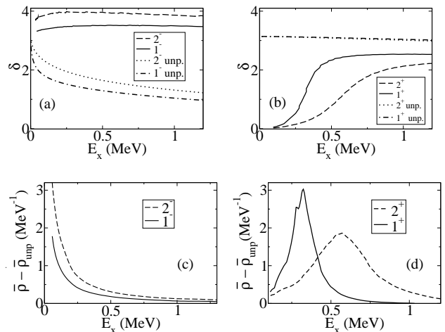
FIG. 2. Upper panels: Phase shifts associated with the renormalized and the unperturbed single-particle states of negative (a) and positive (b) parity in ^{10}\text{Li} . Lower panels: differences between the spectral functions of the renormalized low-lying negative (c) and positive (d) parity states and the spectral functions of the corresponding unperturbed single-particle states.
