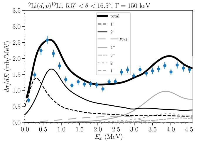
FIG. 5. Theoretical prediction (continuous solid curve) of the ^{10}\text{Li} strength function for the d(^9\text{Li},p)^{10}\text{Li} reaction at 100 MeV incident energy and \theta_{CM} = [5.5^\circ, 16.5^\circ] in comparison with the experimental data (solid dots with errors) [62] (see also Fig. 3(a)).
