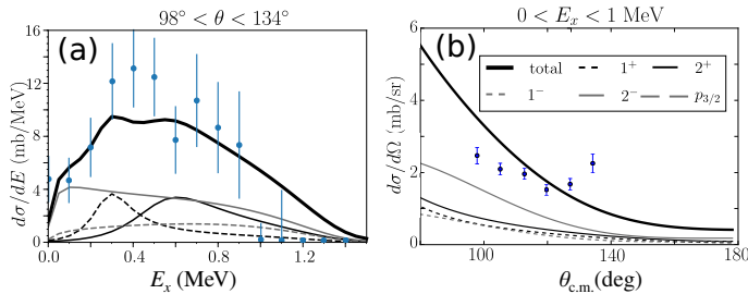
FIG. 4. (Color online) (a) Theoretical prediction (continuous solid curve) of the ^{10}\text{Li} strength function for the d(^9\text{Li},p)^{10}\text{Li} reaction at 21.4 MeV incident energy and \theta_{CM} = [98^\circ, 134^\circ] in comparison with the experimental data. (solid dots with errors) [26]. The data expressed as counts/MeV in [26] have been converted into mb/MeV using the appropriate acceptance function (A.M. Moro, private communication). (b) Corresponding angular distributions associated with the states in the energy interval 0–1 MeV in comparison with the experimental data.
