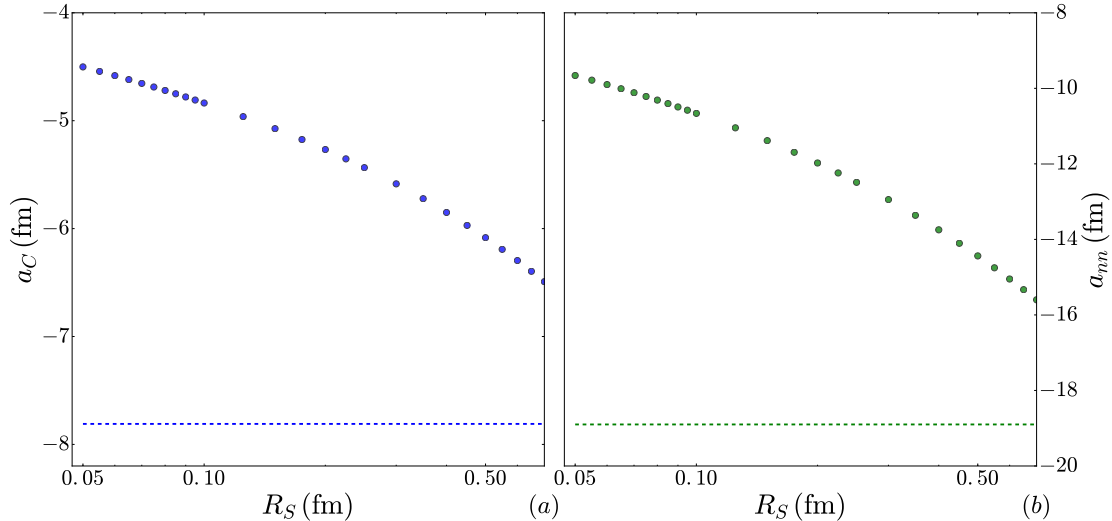
FIG. 12. Proton-proton scattering length a_C (left panel a) and neutron-neutron scattering length a_{nn} (right panel b), as a function of the coordinate-space cutoff R_S . The points are computed with the long-range potentials V_{pp} and V_{nn} defined in Eq. (145), and with a charge-independent short-range potential with LEC C = C_{np} fitted to the np scattering length in the ^1S_0 channel, a_{np} . The dashed lines indicate the experimental values of a_C and a_{nn} .
