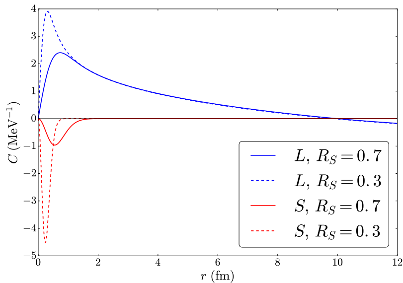
FIG. 14. Matrix-element densities for the nn \rightarrow ppe^-e^- transition as a function of the radial coordinate. Curves are shown for the long- (blue) and short-range (red) components of the 0\nu\beta\beta transition operator for two choices of the cutoff R_S , 0.7 (solid) and 0.3 (dashed) fm.
