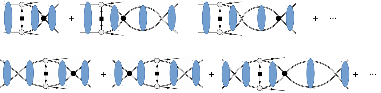
FIG. 3. Diagrammatic representation of LO and NLO contributions to nn \rightarrow pp e^- e^- induced by long-range neutrino exchange. Double, dashed, and plain lines denote nucleons, pions, and leptons, respectively. Gray circles denote the nucleon axial and vector currents, and the black square an insertion of m_{\beta\beta} . The blue ellipse represents iteration of V_\pi , while an unmarked contact interaction stands for C . In the NLO diagrams, the black circle denotes an insertion of C_2 . Diagrams analogous to those in the second and fourth rows, but with contact interactions to the left of neutrino exchange, are not shown. The diagrams for \not\chi EFT are obtained by neglecting pion exchange in the blue ellipse.
