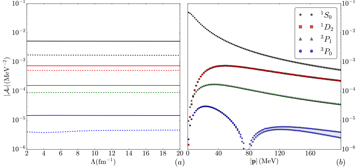
FIG. 9. Left panel (a): absolute value of neutrino amplitude \mathcal{A}_\nu for the ^1S_0 (black), ^1D_2 (red), ^3P_1 (green), and ^3P_0 (blue) channels as a function of momentum-space cutoff \Lambda . Solid (dashed) lines correspond to |\mathbf{p}| = 50 MeV ( |\mathbf{p}| = 100 MeV). Right panel (b): absolute value of neutrino amplitude \mathcal{A}_\nu in the ^1S_0 (black stars), ^1D_2 (red squares), ^3P_1 (green triangles), and ^3P_0 (blue dots) as functions of the neutron center-of-mass momentum |\mathbf{p}| . The bands (all except blue are nearly invisible) represent cutoff variation in the range 2 to 20 \text{fm}^{-1} .
