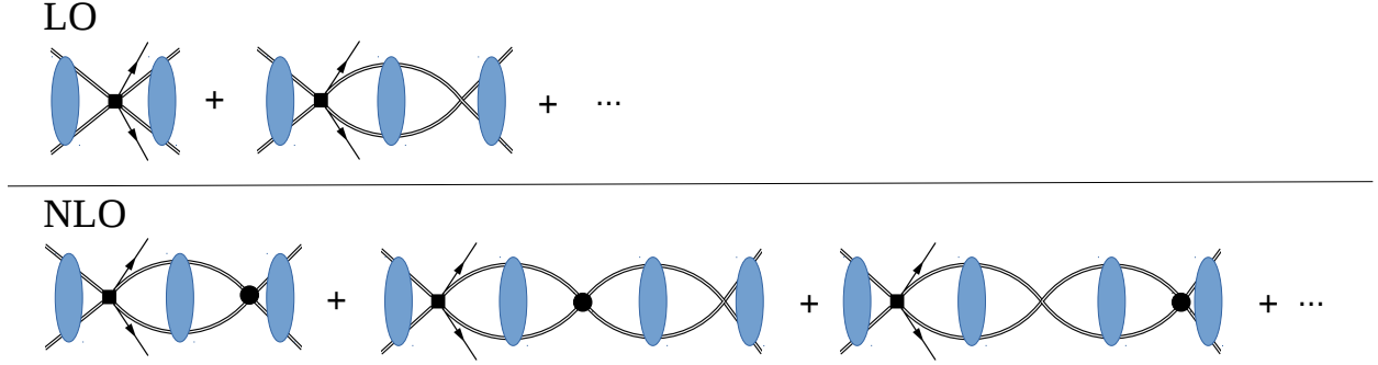
FIG. 4. Diagrammatic representation of LO and NLO contributions to nn \rightarrow pp e^- e^- induced by the short-range operator g_\nu^{\text{NN}} . The notation is as in Fig. 3. The diagrams for \not\pi EFT are obtained by neglecting pion exchange in the blue ellipse.
