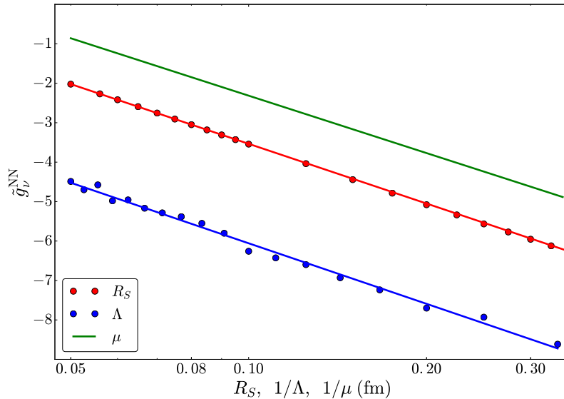
FIG. 6. Dimensionless counterterm \tilde{g}_\nu^{\text{NN}} in \chi\text{EFT} as a function of the coordinate- and momentum-space cutoffs R_S (red) and \Lambda (blue), and of the dimensional-regularization scale \mu (green). Red and blue points denote the results of numerical calculations, while the corresponding lines are logarithmic fits, as explained in the text. The counterterm is determined by imposing the (arbitrary) condition \mathcal{A}_\nu \exp(-i(\delta_{1S_0}(E) + \delta_{1S_0}(E'))) = -0.05 \text{ MeV}^{-2} at |\mathbf{p}| = 1 \text{ MeV} .
