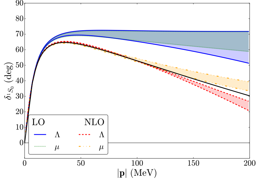
FIG. 5. Phase shifts for np scattering in the ^1S_0 channel, computed in \chi EFT with a momentum space ( \Lambda ) cutoff and in dimensional regularization ( \mu ), as function of the center-of-mass momentum |\mathbf{p}| . The solid blue and dashed red lines denote the momentum-cutoff results at LO and NLO, respectively. The bands are obtained by varying \Lambda between 2 and 20 \text{fm}^{-1} . The dotted green and dash-dotted orange lines are the LO and NLO results in dimensional regularization. The bands in the \overline{\text{MS}} scheme are obtained by varying the regulator of the intermediate scheme, as discussed in App. B, between 1/\lambda = 0.05 \text{ fm} and 1/\lambda = 0.7 \text{ fm} . C is fit to the scattering length, and C_2 to the phase shift at |\mathbf{p}| = 30 \text{ MeV} . The black line shows the Nijmegen partial-wave analysis [93].
