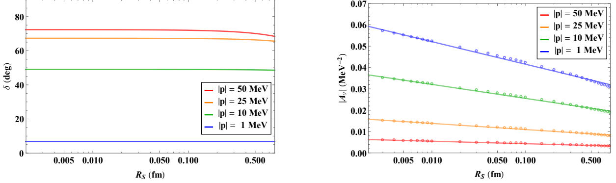
FIG. 2. The left panel shows the phase shifts in the ^1S_0 channel for several momenta |\mathbf{p}| as functions of the cutoff, R_S . The right panel shows the 0\nu\beta\beta amplitude of Eq. (8). The dots result from explicitly evaluating Eq. (8), while the straight lines are due to a fit of the form \mathcal{A}_\nu = a + b \ln R_S .
