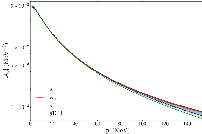
FIG. 7. Magnitude of the LNV scattering amplitude \mathcal{A}_\nu as a function of the neutron center-of-mass momentum |\mathbf{p}| at LO. The red, blue, and green lines represent the results in \chi EFT with coordinate-space, momentum-space, and dimensional regularization, respectively, using g_\nu^{\text{NN}} from Fig. 6. The bands indicate residual regulator dependence, and are obtained by varying R_S between 0.05 and 0.7 fm, \Lambda between 2 and 20 \text{fm}^{-1} , and 1/\lambda between 0.05 fm and 0.7 fm. The dashed black line is the result in \not\chi EFT with dimensional regularization. Since the \not\chi EFT amplitude can be made exactly \mu -independent at this order, there is no band associated with the \mu variations.
