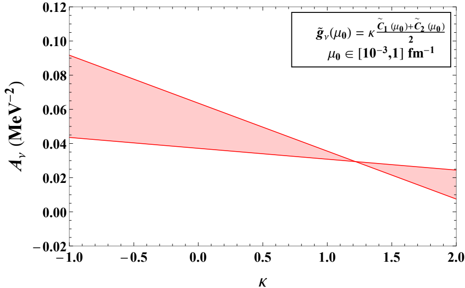
FIG. 15. Dependence of the sum of the short- and long-range nn \rightarrow pp e^- e^- amplitudes at \mathbf{p} = 1 MeV, on the parameter \kappa that parametrizes the relation between \tilde{g}_\nu and the CIB counterterms \tilde{\mathcal{C}}_1 + \tilde{\mathcal{C}}_2 at a given scale \mu_0 . The bands are obtained by varying \mu_0 between 10^{-3} and 1 fm ^{-1} .
