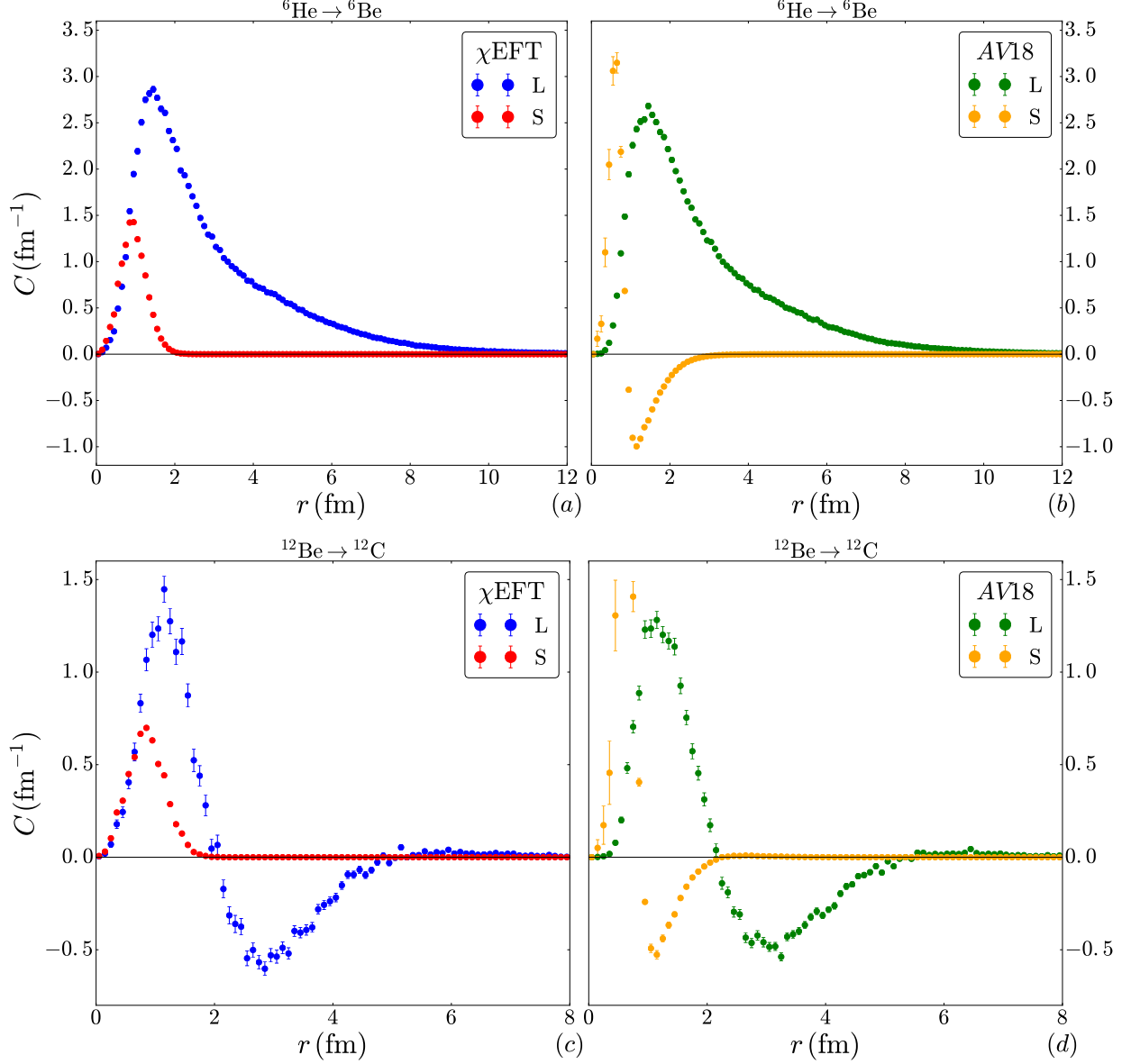
FIG. 17. VMC calculations of the long- (L) and short- (S) range transition densities C(r) for {}^6\text{He}\rightarrow{}^6\text{Be} (upper panels a and b) and {}^{12}\text{Be}\rightarrow{}^{12}\text{C} (bottom panels c and d) decays with two potentials, labeled \chi\text{EFT} (left panels a and c) and AV18 (right panels b and d).
