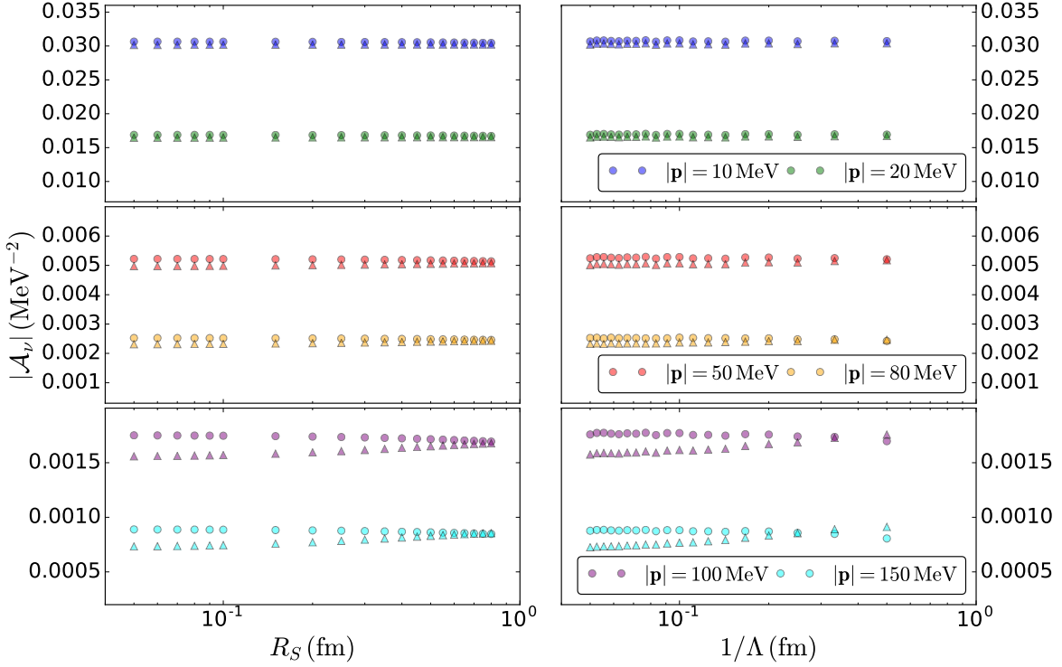
FIG. 10. Magnitude of the LNV matrix element \mathcal{A}_\nu at various values of the neutron center-of-mass momentum: |\mathbf{p}| = 10, 20, 50, 80, 100, and 150 MeV. Left and right panels show \mathcal{A}_\nu as function of coordinate- and momentum-space regulators, respectively. Circles and triangles denote results at, respectively, LO and NLO. For the purpose of illustration, the LNV counterterm is determined by imposing the (arbitrary) condition |\mathcal{A}_\nu| = 0.05 \text{ MeV}^{-2} at |\mathbf{p}| = 1 \text{ MeV} .
