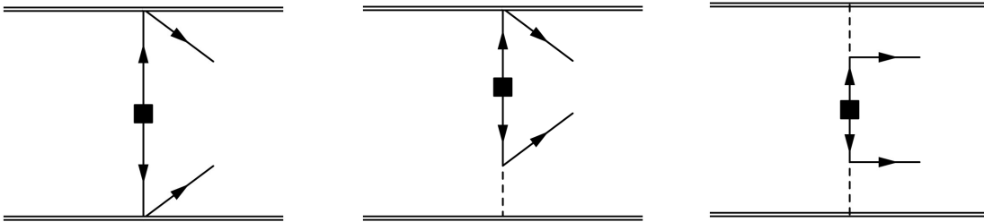
FIG. 1. Long-range contributions to the neutrino potential. Double and dashed lines denote, respectively, nucleons and pions. Single lines denote electrons and neutrinos, and a square an insertion of m_{\beta\beta} .
