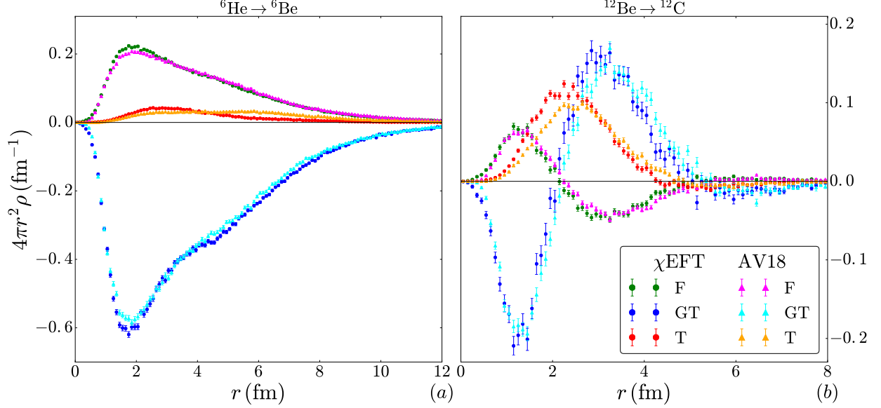
FIG. 16. VMC calculations of the Fermi (F), Gamow-Teller (GT), and tensor (T) densities \rho(r) for {}^6\text{He} \rightarrow {}^6\text{Be} (left panel a) and {}^{12}\text{Be} \rightarrow {}^{12}\text{C} (right panel b) decays with two potentials, labeled AV18 and \chi\text{EFT} .
