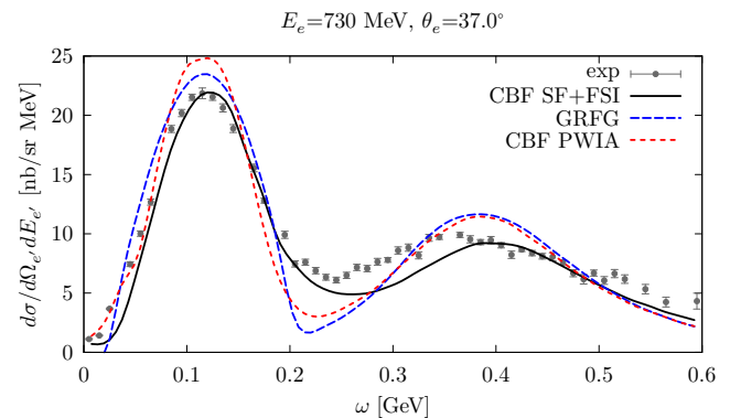
FIG. 10. Electron- ^{12}\text{C} double-differential cross section. The dashed (blue) line has been obtained within the GRFG model. The short-dashed (red) and solid (black) curves have been obtained using the SF of Ref. [39] within the PWIA and IA with FSI corrections, respectively.
