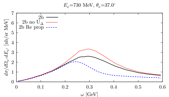
FIG. 8. Two-body current contribution to the double-differential electron- ^{12}\text{C} cross section for E_e = 730 MeV and \theta_e = 37^\circ . The solid (black) line corresponds to results in which the in-medium corrections to the \Delta -decay are included, while the short-dashed (red) line is obtained neglecting this contribution. The dashed (blue) line displays the two-body current contribution in which only the real part of the \Delta propagator is retained.
