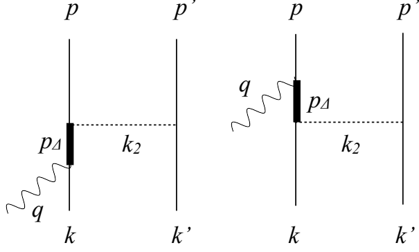
FIG. 2. Feynman diagrams describing two-body currents contributions associated to delta excitations processes. Solid, thick, and dashed lines correspond to nucleons, deltas, pions, respectively. The wavy line represents the vector boson.
