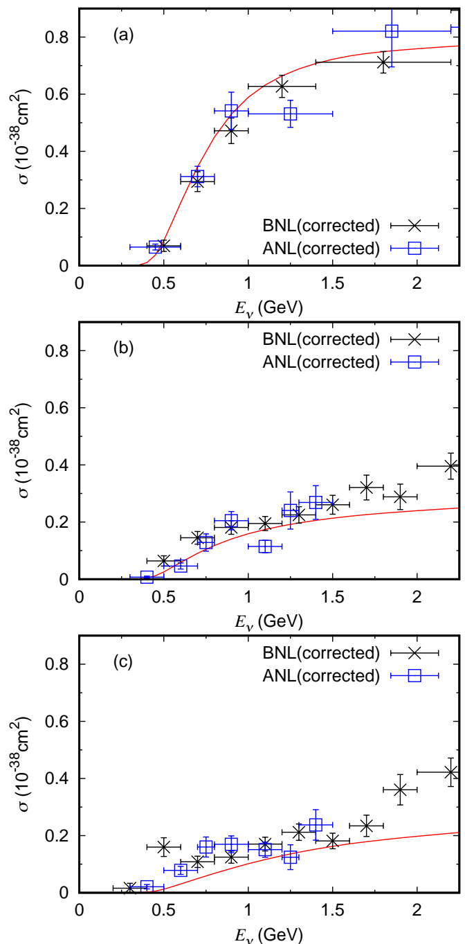
FIG. 6. Total cross sections of (a) \nu_\mu p \rightarrow \mu^- \pi^+ p ; (b) \nu_\mu n \rightarrow \mu^- \pi^0 p ; (c) \nu_\mu n \rightarrow \mu^- \pi^+ n . The solid red curves are from the DCC model. The data are from ANL [95] and BNL [96].
