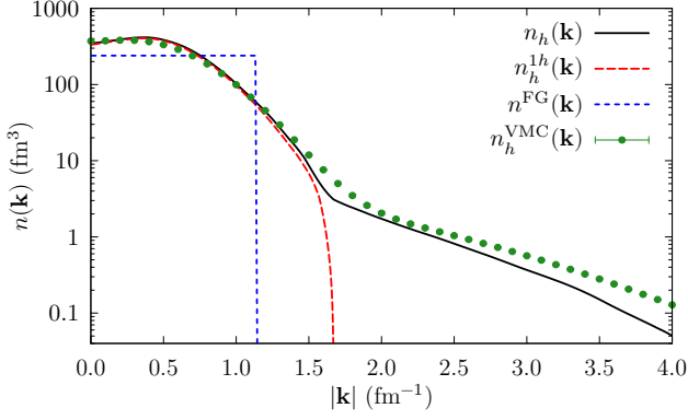
FIG. 1. Momentum distributions associated with the hole SF ( n_h(\mathbf{k}) ), the mean-field component of the hole SF ( n_h^{1h}(\mathbf{k}) ), the free Fermi gas at k_F = 225 MeV ( n^{\text{FG}}(\mathbf{k}) ), and the VMC results of [66] ( n_h^{\text{VMC}}(\mathbf{k}) ).
