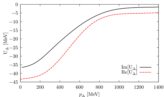
FIG. 3. Real and imaginary part of the \Delta potential in nuclear matter at saturation density \rho = 0.16 \text{ fm}^{-3} .
