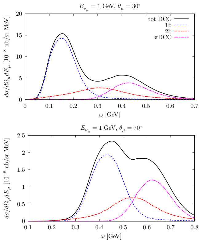
FIG. 12. Double-differential cross section for the \nu_\mu + {}^{12}\text{C} \rightarrow \mu^- + \text{X} process at E_\nu = 1 GeV, \theta_\mu = 30^\circ (upper panel), and E_\nu = 1 GeV, \theta_\mu = 70^\circ (lower panel). The different curves are the same as in Fig. 11.
