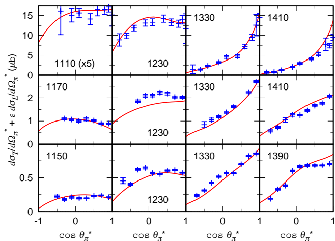
FIG. 5. Same as Fig. 4 but for the p(e, e'\pi^+)n reaction. Experimental data are from Ref. [90–92].
