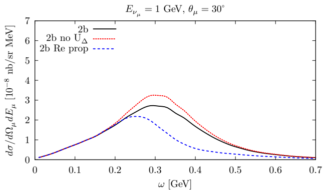
FIG. 9. Same as Fig. 8 but for CC \nu_\mu - ^{12}\text{C} scattering at E_{\nu_\mu} = 1 GeV and \theta_\mu = 30^\circ .
