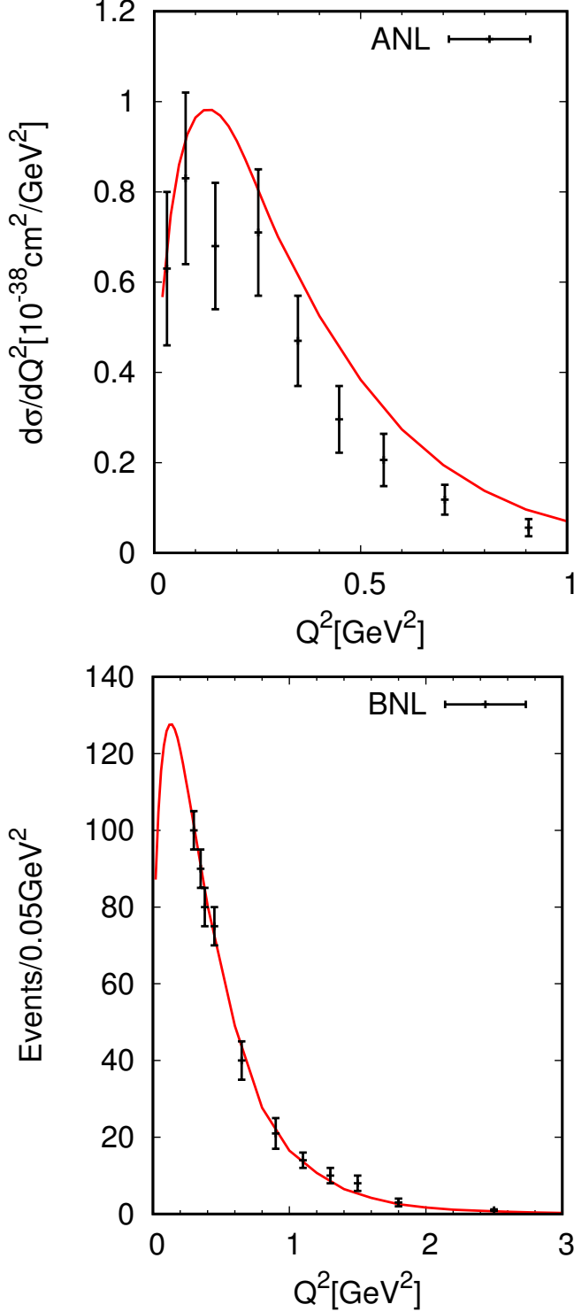
FIG. 7. Flux-averaged ( 0.5 \text{ GeV} \leq E_\nu \leq 6 \text{ GeV} ) d\sigma/dQ^2 for \nu_\mu p \rightarrow \mu^- \pi^+ p . The solid red curves are from the DCC model. The data are from ANL [95] and BNL [96].
