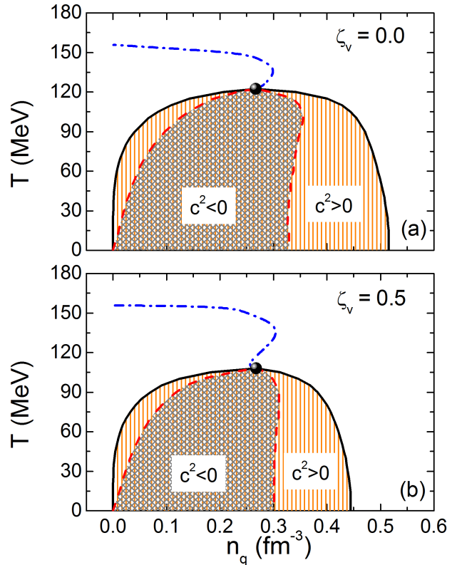
FIG. 3. (Color online) Temperature, T , versus quark number density, n_q , for 3-flavor quark matter without (a) and with (b) vector interactions. The crossover and the first order phase transitions are shown by the dot-dashed blue and solid black lines, respectively. The critical endpoint (CEP) is marked with a solid black dot. Unstable ( c_s^2 < 0 ) and metastable ( c_s^2 > 0 ) regions are highlighted.
