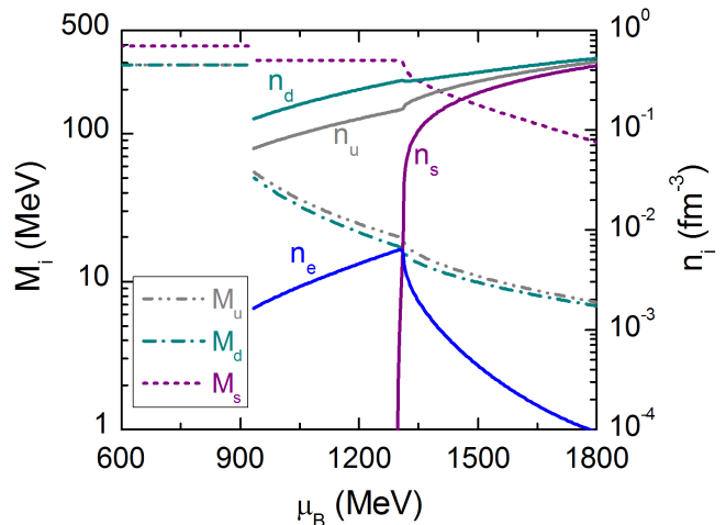
FIG. 8. (Color online) Dynamical masses, M_i , and number densities, n_i , of up , down and strange quarks as a function of baryon chemical potential. n_e denotes the number density of electrons.
