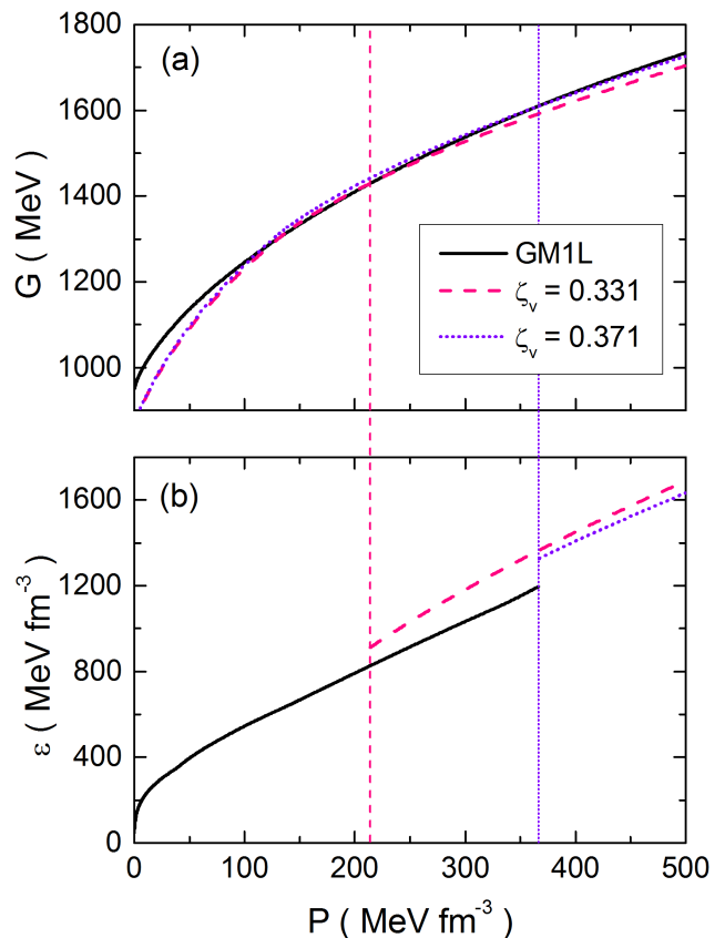
FIG. 6. (Color online) Panel (a) shows the construction of the EoS (at T = 0 ) from the Gibbs free energy (per particle), G , for the hybrid GM1L-3nPNJL parametrization. The solid black line represents the hadronic (GM1L) EoS and the red dashed and blue dotted lines are the EoSs of the quark (3nPNJL) phase for two values of the vector coupling constant, \zeta_v . Panel (b) shows the energy density, \epsilon , as function of pressure, P , for the two values of \zeta_v , discussed in the text.
