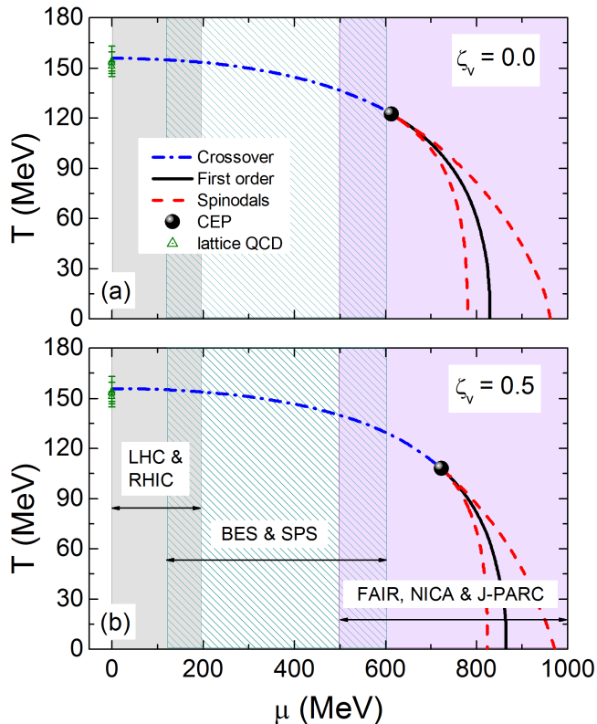
FIG. 2. (Color online) Temperature, T , versus baryon chemical potential, \mu , for 3-flavor quark matter without (a) and with (b) vector interactions. LQCD results [44–46] are marked. The crossover phase transition is shown by the dot-dashed blue line. The dashed red line shows the spinodals, the solid black lines marks the first-order phase transition. The location of the critical endpoint (CEP) is shown by the solid dot.
