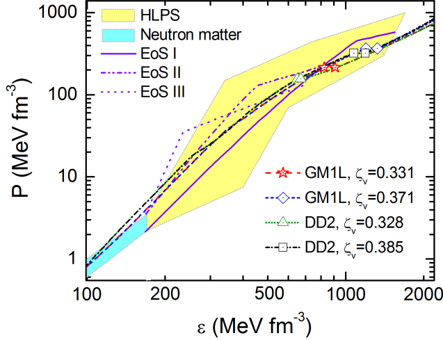
FIG. 9. (Color online) Comparison of the zero-temperature quark-hybrid EoSs of this work (GM1L, DD2) with models (HLPS, Neutron EoS I, EoS II, EoS III) from the literature [73–75]. The solid dots mark the beginning and the end of the quark-hadron phase for our EoSs. The symbol \zeta_v denotes the vector interaction strengths.
