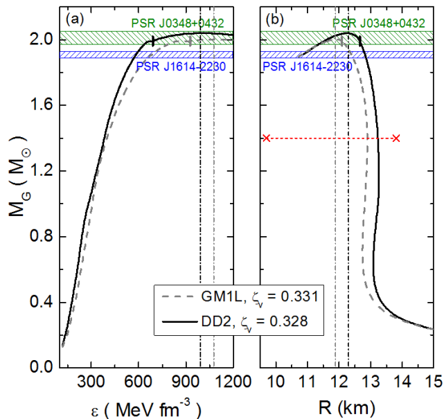
FIG. 11. (Color online) (a) Gravitational mass as a function of central energy density, and (b) gravitational mass as a function of stellar radius, for T = 0 MeV. The vertical bars show the onset of the transition of hadronic matter to quark matter. The vertical dash-dotted lines mark the location of the maximum-mass star for each EoS. The dashed horizontal line shows the estimate of a 1.40M_{\odot} neutron-star radius derived from GW170817 [30–34].
