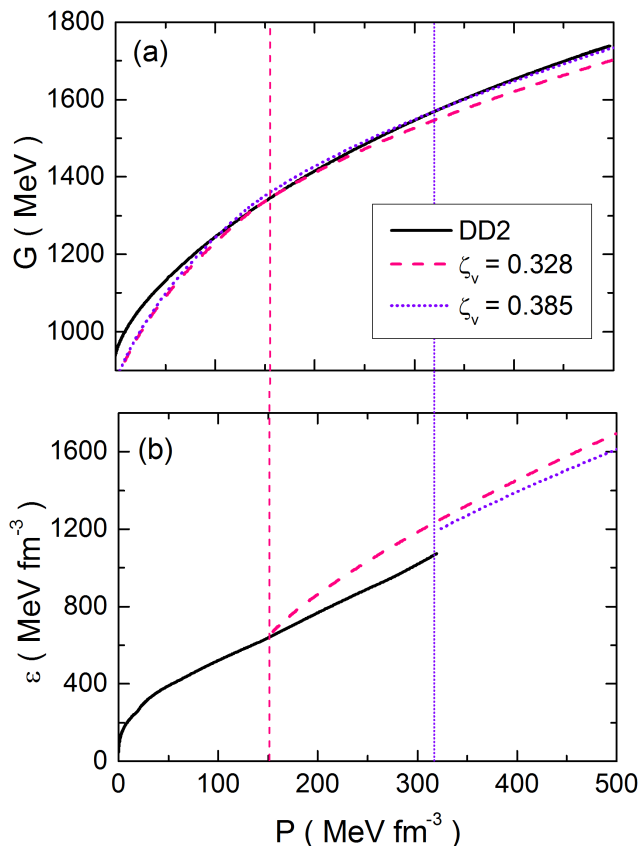
FIG. 7. (Color online) Panel (a) shows the construction of the EoS (at T = 0 ) from the Gibbs free energy (per baryon) G for hybrid DD2-3nPNJL parametrization. The solid black line represents the hadronic (DD2) EoS and the red dashed and blue dotted lines are the EoSs for the quark (3nPNJL) phase for two values of the vector coupling constant, \zeta_v . Panel (b) shows the energy density, \epsilon , as function of pressure, P , for the two values of \zeta_v , discussed in the text.
