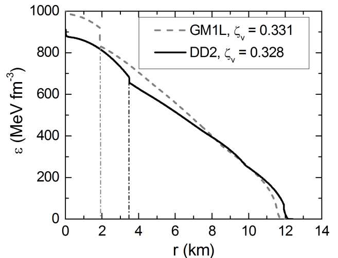
FIG. 12. (Color online). Energy density as a function of radius for the maximum-mass neutron stars shown in Fig. 11. The density discontinuities at around 2 and 3.5 km (dash-dotted vertical lines) are caused by the quark-hadron phase transition in these stars.
