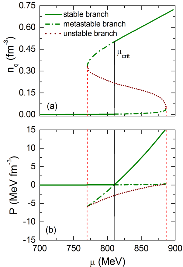
FIG. 4. (Color online) (a) Quark number density, n_q , and (b) pressure, P , as a function of baryon chemical potential, \mu , at T = 50 MeV. The dotted, solid and dot-dashed lines show unstable, stable, and metastable equilibrium, respectively.
