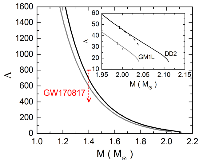
FIG. 17. (Color online) Tidal deformability versus gravitational mass of pure hadronic stars (solid lines). Hybrid branches are indicated by dashed lines. The small vertical bars on each curve mark the onset of the phase transition from hadronic to quark matter. Each line terminates at the maximum-mass star. The red arrow shows the constraint on \Lambda imposed by the analysis of the data of GW170817.
