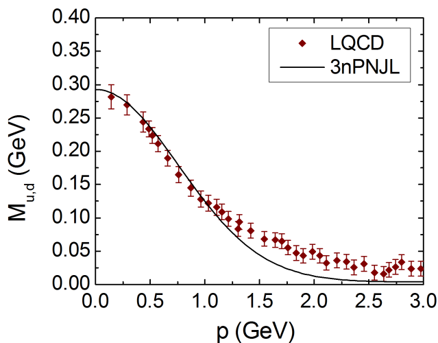
FIG. 1. (Color online) Dependence of the dynamical masses of light ( u and d ) quarks on momentum p for the parametrization used in this work. (solid line). The diamond shaped symbols show the results of LQCD calculations for N_f = 2 + 1 quark flavors extracted from [43].
