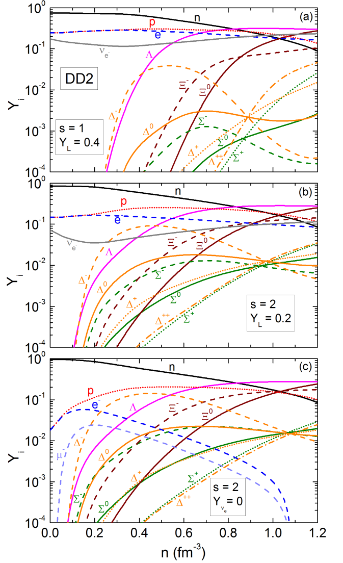
FIG. 15. (Color online) Same as Fig. 14, but for the DD2 parametrization.
