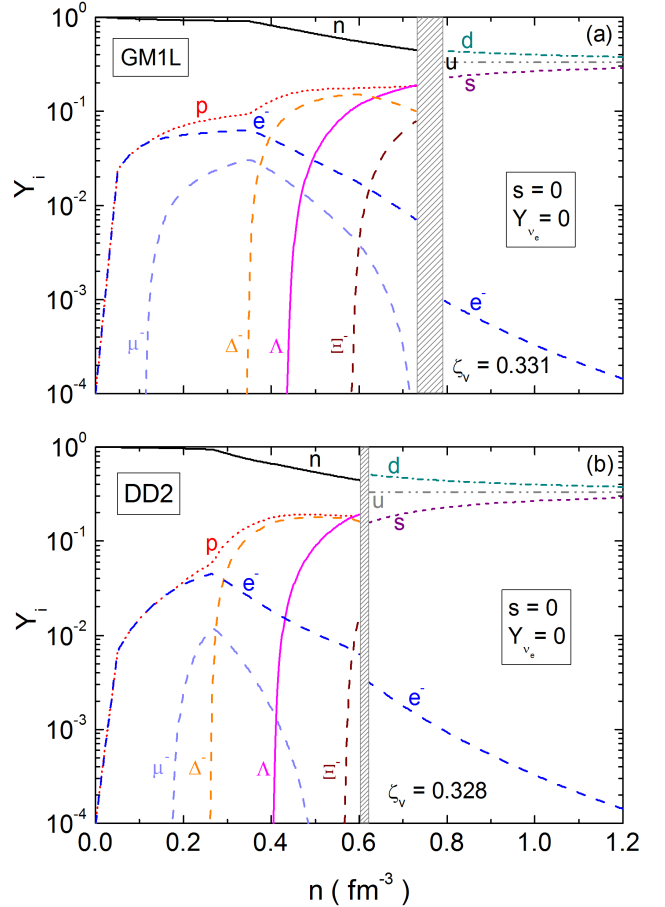
FIG. 10. (Color online) Particle population of stellar quark-hybrid matter at zero temperature as a function of baryonic number density. The populations are computed for GM1L-3nPNJL and DD2-3nPNJL (see text). \zeta_v denotes the strength of the vector repulsion among quarks.
