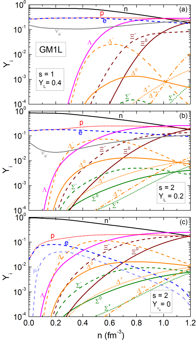
FIG. 14. (Color online) Particle populations of proto-neutron star matter for the GM1L parametrization. The compositions correspond to matter in the cores of proto-neutron stars at different evolutionary stages characterized by entropy per baryon, s , and lepton number, Y_L .
