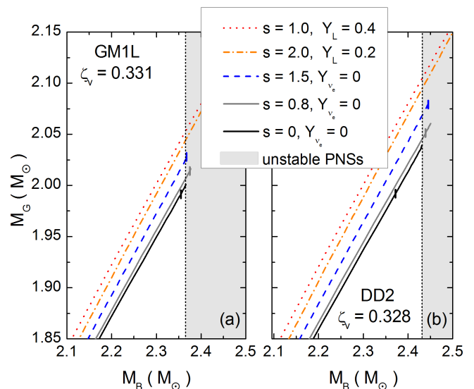
FIG. 16. (Color online) Gravitational mass versus baryonic mass of selected stages (characterized by entropy and lepton number) in the evolution of EOSs of this paper. Each line terminates at the maximum-mass star of each stage. The small vertical bars close to the maximum-masses mark the onset of the hadron-quark phase transition. Only the most massive members of the cold neutron-star sequence are found to have pure quark matter in their cores. Stars in the shaded region are gravitationally unstable.
