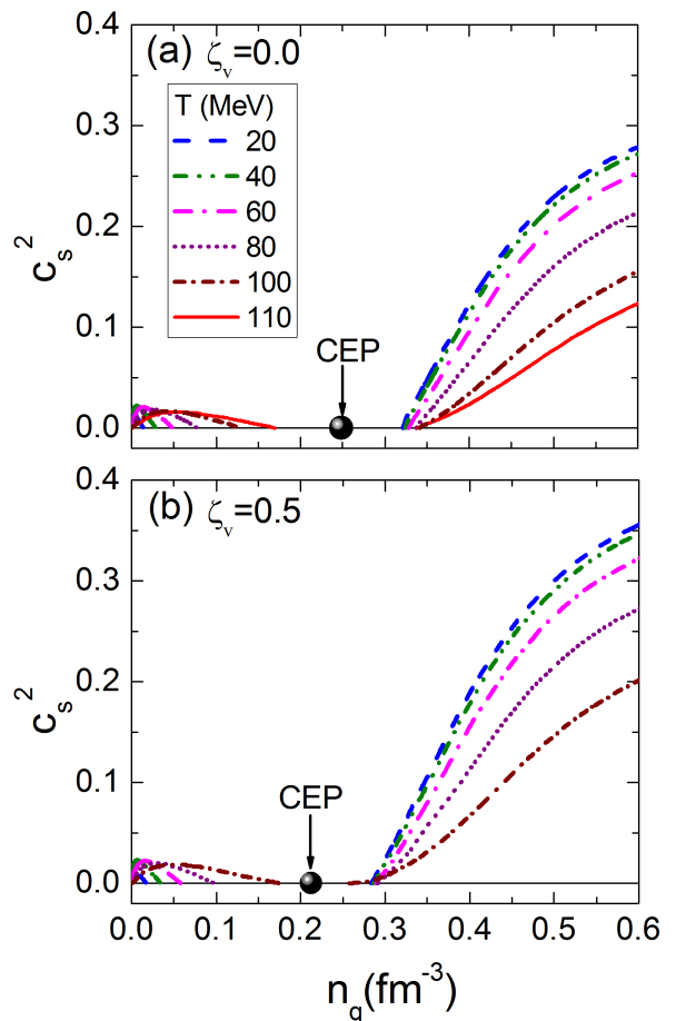
FIG. 5. (Color online) Isotherms of the square of the speed of sound, c_s^2 , as a function of quark number density, n_q without (a), and with (b) vector interactions among quarks. The solid dots indicate the location of the critical endpoints (CEP).
