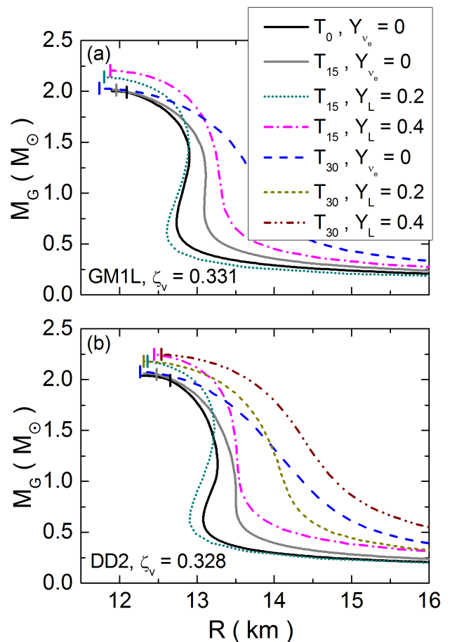
FIG. 13. (Color online) Gravitational mass, M_G , as a function of radius, R , for quark-hybrid stars at different transition temperatures, T_{\text{trans}} , of the quark-hadron phase transition. Y_L denotes the lepton fraction and Y_{\nu_e} the neutrino fraction. The vertical bars mark the onset of quark deconfinement. With the exception of the neutrino-less ( Y_{\nu_e} = 0 ) stars with T_{\text{trans}} = 0 ( T_0 ) and T_{\text{trans}} = 15 MeV ( T_{15} ), this transition happens at the maximum-mass peak.
