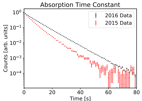
FIG. 4: Neutron counted by the in-situ detector as a function of time after the detector insertion. Note that the same detector shows different time constants for two subsequent years of operation. (color online)
