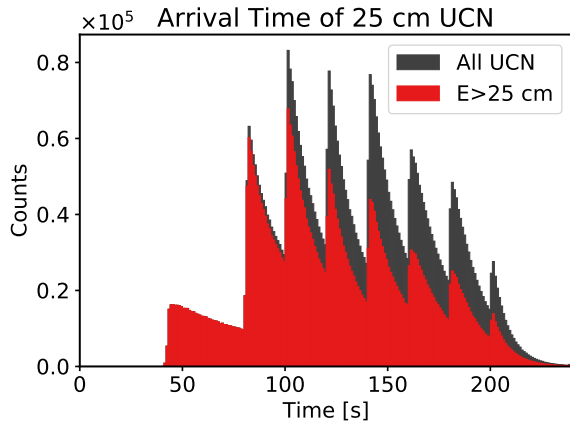
FIG. 15: The detection of neutrons (all energies) in the 9-step detection (the dark gray histogram) is compared to the detection of high-energy neutrons, E/m_{ng} > 25 cm (the red (gray) histogram). The first peak has no counts due to the high efficiency of the cleaner. The second peak measures neutrons with E/m_{ng} > 25 cm. Note that the subsequent peaks at increasingly lower height contains sizable population of the same high energy neutrons with E/m_{ng} > 25 cm. The extrapolated sum of P2 counts only 30% of the total UCN with E/m_{ng} > 25 cm. (color online)
