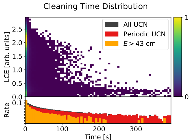
FIG. 11: The distribution of LCE and the arrival time on the cleaner. The bottom figure shows the count rate by integrating the neutrons over the full range of the UCN energy (dark gray), and over neutrons with LCE < 0.75 with quasi-periodic trajectories (red/gray), and over neutrons with E/m_n g > 43 cm (orange/light gray). (color online)
