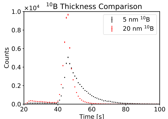
FIG. 5: Detector response (for a 3-step measurement) with two different thicknesses of the boron layer. The one with a thicker boron layer counts the neutrons in the MG trap faster. (color online)
