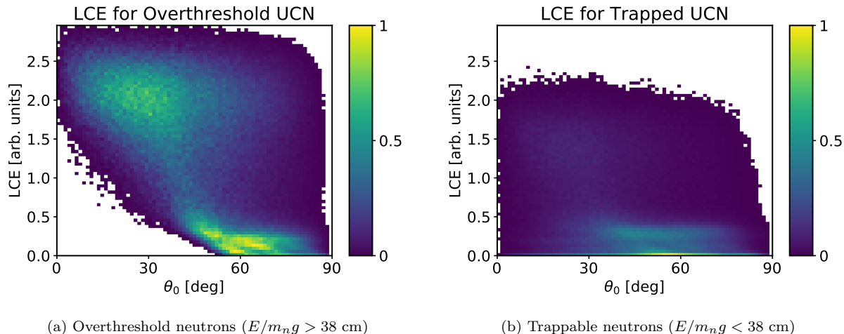
FIG. 12: Distribution of the initial polar angle and the Lyapunov exponent for (a) overthreshold neutrons and (b) trappable neutrons. (color online)
