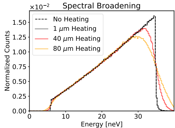
FIG. 16: The spectrum of detected neutrons in the simulation with vibration of microphonic frequencies. Scenarios of no vibration, 1 \mu\text{m} , 40 \mu\text{m} , and 80 \mu\text{m} are shown. The neutron spectrum broadens with increasing amplitude of vibration. (color online)
