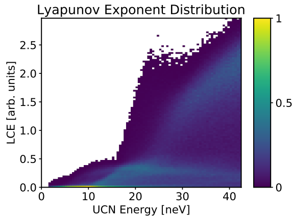
FIG. 10: The distribution of LCE of neutron trajectories and the corresponding neutron energy. (color online)
