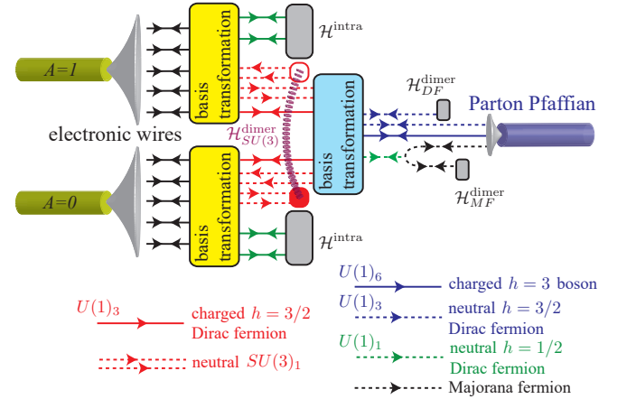
FIG. 8. Emergence of parton Pfaffian from ten electronic wires. Each of the pair of basis transformations in the yellow boxes is defined in (78) and (79). The second basis transformation in the blue box is the product of (106) and (110). \mathcal{H}^{intra} , \mathcal{H}_{SU(3)}^{dimer} , \mathcal{H}_{DF}^{dimer} and \mathcal{H}_{MF}^{dimer} are defined in (84), (105), (116) and (117) respectively.
