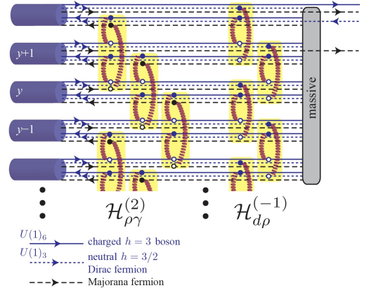
FIG. 10. Coupled wire model and its gapless edge modes of the \nu = 1/6 parton Pfaffian state \mathfrak{P}_{2,-1} in (128). \mathcal{H}_{\rho\gamma}^{(2)} and \mathcal{H}_{d\rho}^{(-1)} are defined in (132) and (133).
