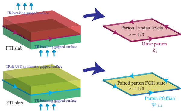
FIG. 1. Correspondence between thin FTI slabs with gapped surfaces and parton fractional quantum Hall states.
