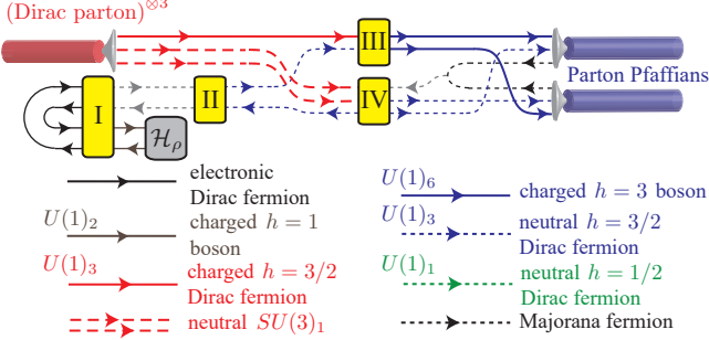
FIG. 3. Splitting of a chiral Dirac triplet channel into a pair of parton Pfaffian channels. The basis transformations (I), (II), (III) and (IV) are defined in (58), (61), (64) and (66) respectively. The backscattering Hamiltonian is defined in (60).
