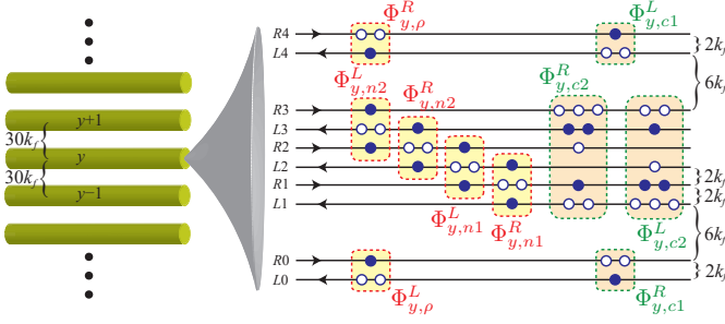
FIG. 4. Bundle arrangement and basis transformation for the \nu = 1/3 parton FQH state. The momentum displacement between channels (directed lines) and bundles (green cylinders) are shown in nk_f , where 2k_f is the displacement between R and L -movers on same wire at Fermi level. Dashed boxes represent products of electronic operators that correspond to (78) and (79). \bullet and \circ represents electron creation and annihilation operators respectively.
