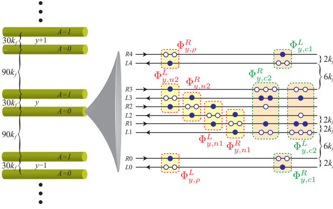
FIG. 7. Bundle arrangement and basis transformation for the \nu = 1/6 Pf* FQH state. The momentum displacement between channels (directed lines) and bundles (green cylinders) are shown in nk_f , where 2k_f is the displacement between R and L -movers on same wire at Fermi level. Dashed boxes represent products of electronic operators. \bullet and \circ represents electron creation and annihilation operators respectively.
