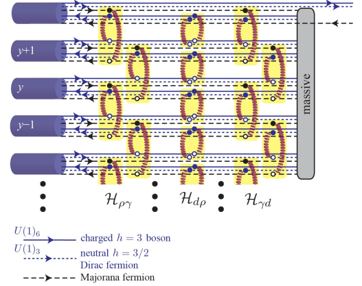
FIG. 9. Coupled wire model and its gapless edge modes of the \nu = 1/6 parton Pfaffian state. \mathcal{H}_{\rho\gamma} , \mathcal{H}_{d\rho} and \mathcal{H}_{\gamma d} are defined in (118), (119) and (120).
