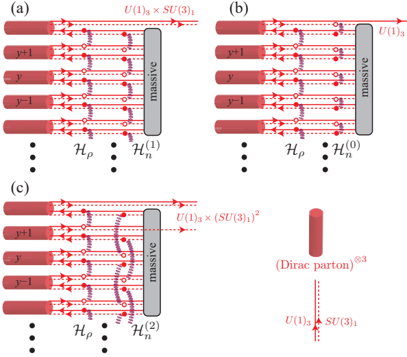
FIG. 6. Coupled wire models and gapless edge modes of (a) the parton state \mathcal{L}_1 = U(1)_3 \times SU(3)_1 with c = 3/2 , (b) the Laughlin state \mathcal{L}_0 = U(1)_3 with c = 1 , and (c) the \mathcal{L}_2 = U(1)_3 \times (SU(3)_1)^2 state with c = 5 . \mathcal{H}_\rho and \mathcal{H}_n^{(q)} are defined (91) and (92) respectively.
