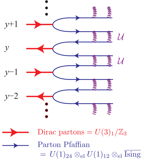
FIG. 11. Coupled wire model of the \mathcal{T} -Pf* surface state of a fractional topological insulator. The energy gap is introduced by the many-body electron backscattering \mathcal{U} defined in (142).
