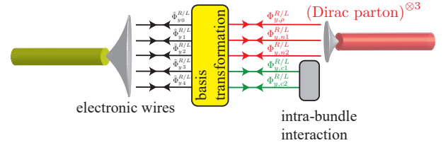
FIG. 5. Emergence of Dirac partons from five electronic wires. The basis transformation is defined in (78) and (79). The intra-bundle interaction is defined in (84).
