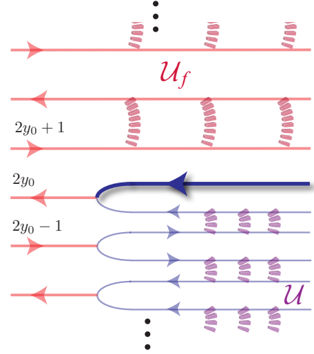
FIG. 12. A parton Pfaffian CFT (highlighted blue line) at the domain wall separating two gapped regions with symmetry-preserving interaction \mathcal{U} and AFTR symmetry breaking interaction \mathcal{U}_f .
