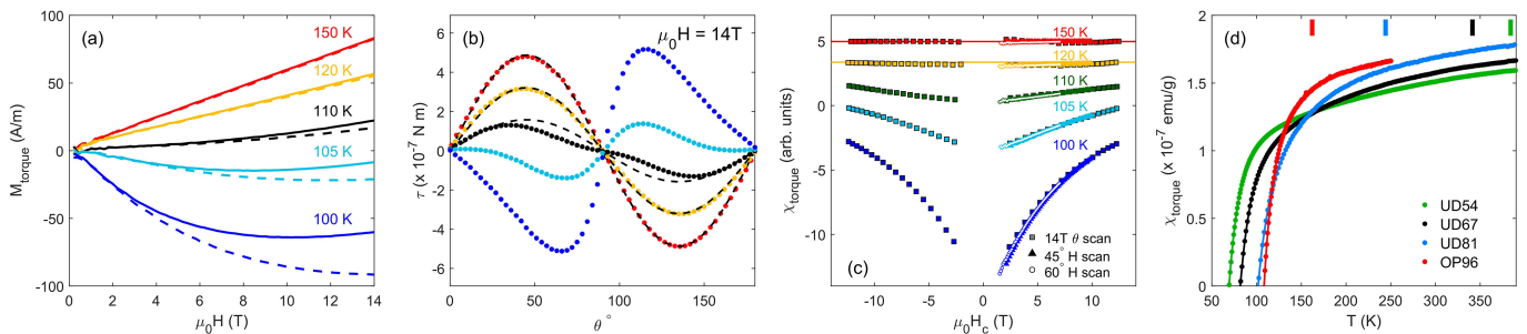
FIG. 1. Data for Hg1201. (a) Field dependence of the effective magnetic moment M_{torque} \equiv \chi_{torque}H at \theta = 45^\circ (solid lines) and 60^\circ (dashed lines) for a nearly optimally doped sample OP96 ( T_c \approx 96 K). M_{torque} equals the effective magnetic moment M_{eff} \equiv \tau/(\mu_0 V H \sin(\theta)) defined in [4, 5] divided by \cos(\theta) . M_{eff} = M_c - M_a H_c / H_a approximates the c -axis magnetization M_c when the in-plane magnetization M_a is negligible. Unlike M_{eff} , M_{torque} is independent of angle \theta for linear magnetism. Therefore, discrepancy of M_{torque} between two different angles at temperatures below 120 K is a clear indication of the appearance of nonlinear magnetism. (b) Angular dependence of the torque for OP96. The temperature is indicated by the same colors as in (a). The deviation from the \sin(2\theta) dependence occurs below the same temperature as the onset of the nonlinear component of M_{eff} in (a). Dashed black lines are fits to \sin(2\theta) for 150, 120 and 110 K. (c) \chi_{torque} as a function of H_c for OP96, calculated from the field dependence in (a) (triangles: \theta = 45^\circ ; circles: \theta = 60^\circ ) and from the angular dependence in (b) (squares: \mu_0 H = 14 T). The two methods agree remarkably well, which indicates that the result is hardly affected by H_a . The contribution from the in-plane response thus is negligible, and \chi_c dominates the nonlinear diamagnetic signal in this temperature range. Horizontal lines at 120 K and 150 K indicate the field-independent paramagnetic contributions. (d) \chi_{torque} over a wide temperature range above T_c for OP96 and three underdoped samples UD54, UD67 and UD81 ( T_c \approx 54, 67, 81 K). \chi_{torque} is obtained with an external magnetic field \mu_0 H = 14 T at \theta = 45^\circ . At high temperature, in the normal state, M_{torque} is independent of \theta , and \chi_{torque} (now equal to \chi_c - \chi_a ) is independent of \theta and H up to at least 14 T with very good accuracy. The vertical bars indicate the pseudogap temperature T^* estimated from neutron scattering [28, 29] and planar dc resistivity measurements [30]. Non-trivial temperature dependences of \chi_{torque} (and d\chi_{torque}/dT ) are observed up to 400 K. Similar behavior as in (a)-(d) is observed for the other cuprates [31].
