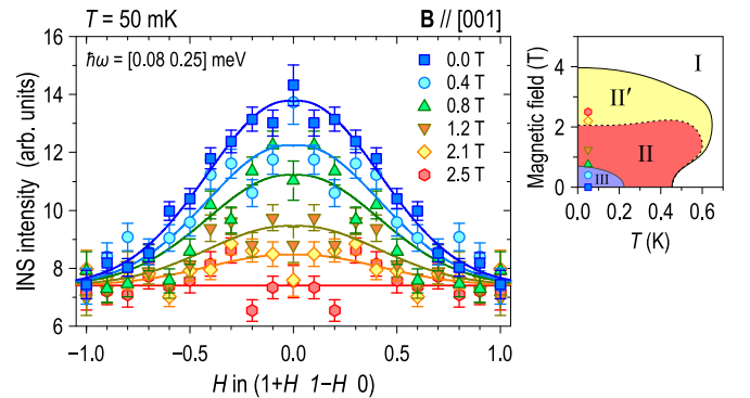
Fig. 3. Magnetic-field dependence of the diffuse INS peak at the (110) wave vector, which represents the tail of the two broad (111) and (1\bar{1}\bar{1}) peaks located above and below the (HK0) scattering plane. The data are symmetrized with respect to the mirror plane of the cubic Brillouin zone. Solid lines are Gaussian fits, showing the suppression of intensity towards the boundary of phases II and II'. A schematic field-temperature phase diagram with the positions of the measured data points is shown to the right.
