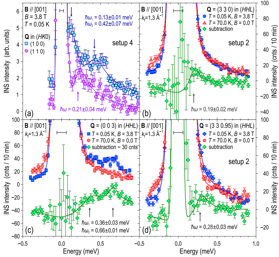
Fig. 8. (a) Constant- Q cuts through the TOF data at B = 3.8 T (setup 4), taken at the (100) and (110) points. The (100) dataset is shifted upwards by 1 unit for clarity. (b–d) The low-temperature TAS spectra at B = 3.8 T (setup 2), reference background spectra ( T = 70 K, B = 0 ), and their corresponding subtractions at three different wave vectors: (330) , (003) , and near (331) , respectively. The subtracted data in panel (b) are shifted down by 30 units for clarity. Arrows mark fitted peak positions. Black horizontal bars indicate energy resolution defined as the full width at half maximum of the elastic line.
