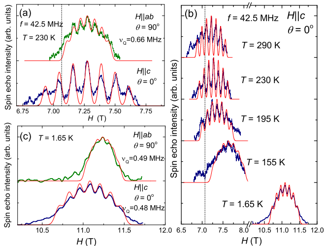
FIG. 2: (a) Typical field-swept ^{139}\text{La} -NMR spectra of \text{LaCrGe}_3 in the PM state at f = 42.5 MHz and T = 230 K for H||c and H||ab . (b) Temperature dependence of ^{139}\text{La} -NMR spectrum for H||c . (c) Field-swept ^{139}\text{La} -NMR spectra in the FM state ( T = 1.65 K) for H||c and H||ab . Blue and green curves represent spectra for H||c and H||ab , respectively, and the red curves are the calculated spectra with \nu_Q = 0.66 MHz for the PM state and \nu_Q \sim 0.49 MHz for the FM state. The vertical dashed black lines in (a) and (b) represent the zero-shift position ( K = 0 ).
