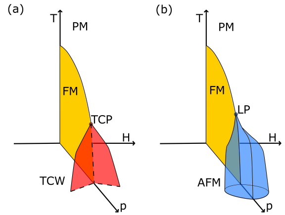
FIG. 1: Generic temperature-pressure-magnetic field ( T - p - H ) phase diagrams for clean itinerant ferromagnets. (a) Schematic T - p - H phase diagram with a tricritical wing (TCW) structure. The second order phase transition (solid line) becomes first order (dashed line) at a tricritical point (TCP). Under magnetic field, the TCW structure shown in red emerge from the TCP. (b) Schematic T - p - H phase diagram with an antiferromagnetic (AFM) phase in blue. The AFM phase emerges from the Lifshitz point (LP) that is suppressed under H .
