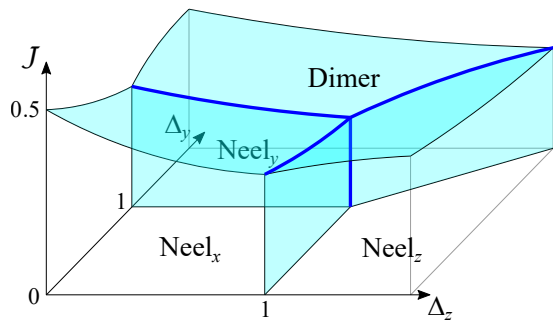
FIG. 2. (Color online) Qualitative phase diagram of the quantum spin-1/2 antiferromagnetic J_1 - J_2 XYZ model in the three-dimensional parameter space (\Delta_z, \Delta_y, \mathcal{J}) . The three Neel phases and the dimer phase are separated by six planes of phase boundaries, each of which realizes Gaussian criticality with U(1) \times U(1) symmetry. These six planes join at the four solid blue lines, along which the fixed-point theory is the Gaussian model with SU(2) symmetry. The dimer phase exists for \mathcal{J} > \mathcal{J}_c(\Delta_y, \Delta_z) . The three Neel _\alpha phases with \alpha = x, y, z are located below the phase boundaries of the Gaussian criticality, \mathcal{J} < \mathcal{J}_c(\Delta_y, \Delta_z) . The pair of Neel _\alpha and Neel _\beta phases with \alpha < \beta = x, y, z are separated by the phase boundary at \Delta_\alpha = \Delta_\beta of the Gaussian criticality ( \Delta_x \equiv 1 ). We have omitted other phases (such as the UDD Ising ordered phase) that can exist for \mathcal{J} > 1/2 .
