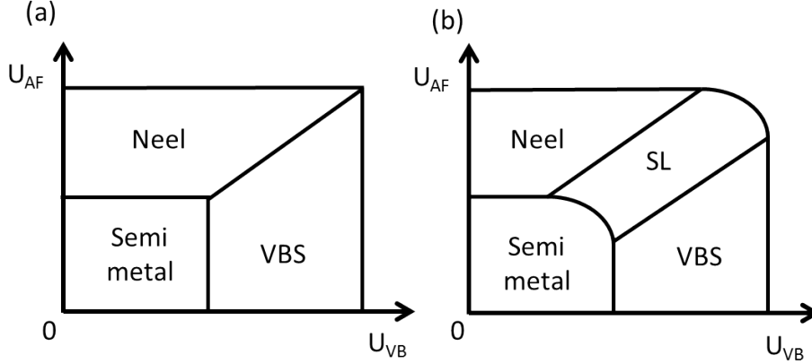
FIG. 11. Two possible phase diagrams for interacting fermionic tight-binding models at half-filling with an O(3)\times O(3) symmetry that realize the \pi -flux phase on the cubic lattice in the noninteracting limit. (a) There exists a phase boundary between the Neel and dimer (valence bond solid) phases that is governed by a continuous quantum critical point at which the dual point defects of either phases have simultaneously proliferated. (b) The Neel and dimer (valence bond solid) phases do not touch. They are separated by a gapless spin liquid (SL) phase characterized by the dual point defects of either phases being simultaneously deconfined.
