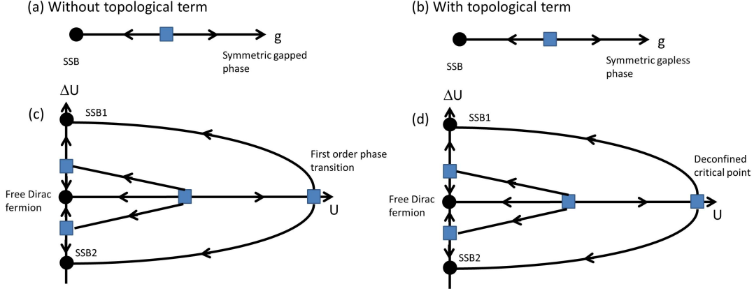
FIG. 10. (Color online) Renormalization-group (RG) flows for the NLSM with O(6) symmetry in (3+1) -dimensional spacetime (a) without any topological term and (b) with a Wess-Zumino term. Panels (c) and (d) show RG flows for Dirac fermions perturbed by O(3)\times O(3) symmetric interactions in (3+1) -dimensional spacetime, assuming that bosonization in their Mott insulating phases delivers the RG flows in panel (a) and (b), respectively, when the interactions are fine-tuned to an O(6) symmetric interaction.
