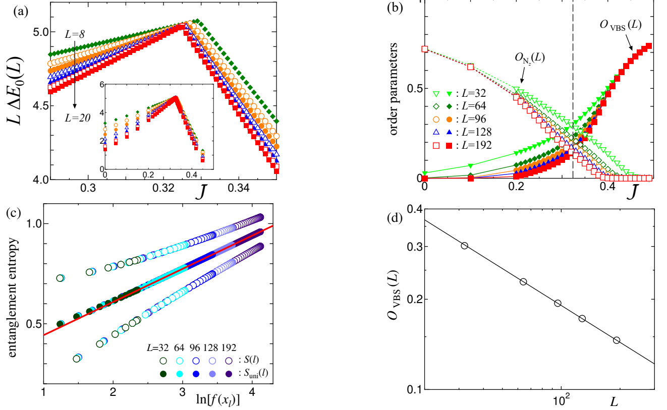
FIG. 14. (Color online) Panels (a), (b), (c), and (d) are the counterparts to Figs. 5(a), 13, 6(b), and 7(a), respectively, when \Delta_z = 3.0 and \Delta_y = 2.0 . The central charge c obtained in (c) (using the data for L = 192 ) is c = 0.994 , and the exponent \eta obtained in (d) is \eta = 1.22 .
