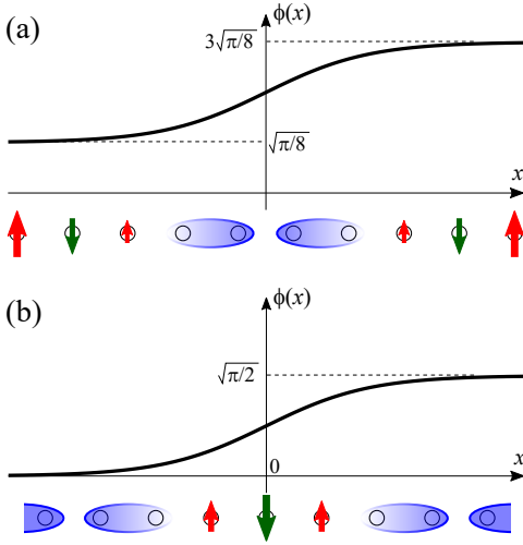
FIG. 8. (Color online) Schematic picture of a domain wall in (a) the Neel z phase and (b) the VBS (dimer) phase.
