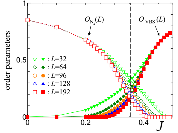
FIG. 13. (Color online) Order parameters O_{N_z}(L) (unfilled symbols) and O_{\text{VBS}}(L) (filled symbols) for \Delta_z = 2.0 and \Delta_y = 0.5 as functions of \mathcal{J} .
