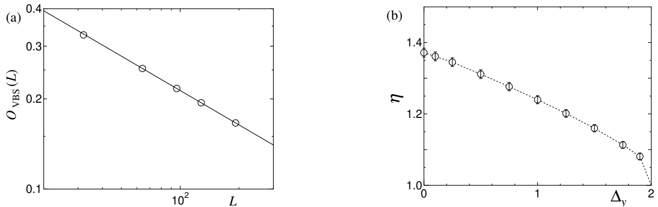
FIG. 7. (a) Log-log plot of the dependence of O_{\text{VBS}}(L) defined in Eq. (2.48) on L at the critical point \mathcal{J} = \mathcal{J}_c for \Delta_z = 2.0 and \Delta_y = 0.5 . (b) Exponent \eta at the Neel z -dimer transition for \Delta_z = 2.0 as a function of \Delta_y .
