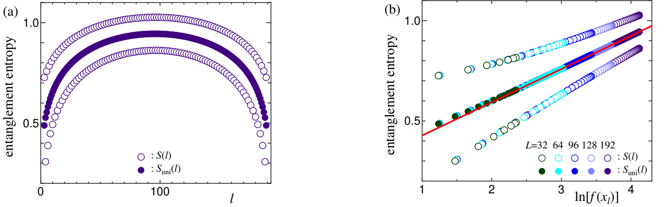
FIG. 6. (Color online) Entanglement entropy \mathcal{S}(l) (open circles) and its uniform part \mathcal{S}_{\text{uni}}(l) (filled circles) at the quantum critical point \mathcal{J} = \mathcal{J}_c for \Delta_z = 2.0 and \Delta_y = 0.5 . (a) \mathcal{S}(l) and \mathcal{S}_{\text{uni}}(l) for L = 192 are plotted as a function of l . Successive open circles are either above or below the curve defined by the filled circles. This effect originates from choosing open boundary conditions. (b) \mathcal{S}(l) and \mathcal{S}_{\text{uni}}(l) for L = 32, 64, 96, 128, 192 are plotted as a function of \ln[f(x_l)] with x_l := l + \frac{1}{2} .
