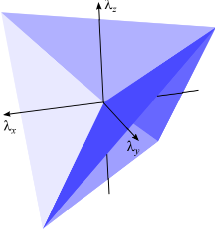
FIG. 4. (Color online) Six critical planes separating four gapped phases in the three-dimensional parameter space (\lambda_x, \lambda_y, \lambda_z) .
