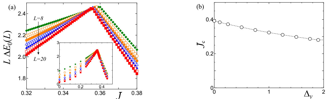
FIG. 5. (Color online) (a) Dependence on \mathcal{J} \equiv J_2/J_1 of the scaled finite-size gap L \Delta E_0(L) with \Delta E_0(L) defined in Eq. (2.44) for \Delta_y = 0.5 , \Delta_z = 2.0 and L = 8 to L = 20 . The position of the cusp defines \mathcal{J}_c(L) . The inset shows the data for the range 0 \leq \mathcal{J} < 1/2 , while the main panel limits the range of data to the vicinity of the cusp singularity. (b) Critical coupling \mathcal{J}_c = \lim_{L \rightarrow \infty} \mathcal{J}_c(L) at which a continuous quantum phase transition separates the Neel z from the dimer phase for \Delta_z = 2.0 as a function of 0 \leq \Delta_y < 2.0 .
