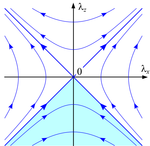
FIG. 3. (Color online) Renormalization-group flow diagram of Eq. (2.38) on the \lambda_x = \lambda_y plane. The shaded region corresponds to the critical phase in Fig. 1.
