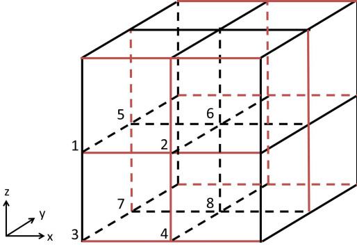
FIG. 9. (Color online) We define the \pi -flux model on the three-dimensional cubic lattice by the following rules. Only nearest-neighbor hopping amplitudes are allowed. All nearest-neighbor hopping amplitudes have the magnitude t/2 > 0 and are real valued. The sign of the nearest-neighbor hopping amplitudes is +1 ( -1 ) when the nearest-neighbor is colored in black (red).
