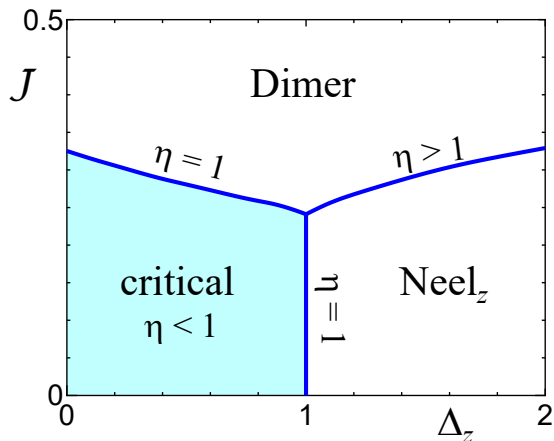
FIG. 1. (Color online) Ground-state phase diagram of the quantum spin-1/2 antiferromagnetic J_1 - J_2 XXZ Hamiltonian (2.4c) with the Ising exchange anisotropy \Delta_z and the exchange ratio \mathcal{J} = J_2/J_1 . The phase boundaries are taken from Ref. 39. When 0 \leq \Delta_z < 1 and 0 \leq \mathcal{J} < \mathcal{J}_c(\Delta_z) , the system is in the critical phase with in-plane spin-correlation exponent \eta < 1 ( \eta = 1 on the boundary of the critical phase). The Umklapp coupling vanishes along the phase boundary with \eta > 1 separating the gapped dimer (VBS) and Neel _z phases that break different \mathbb{Z}_2 symmetries.
