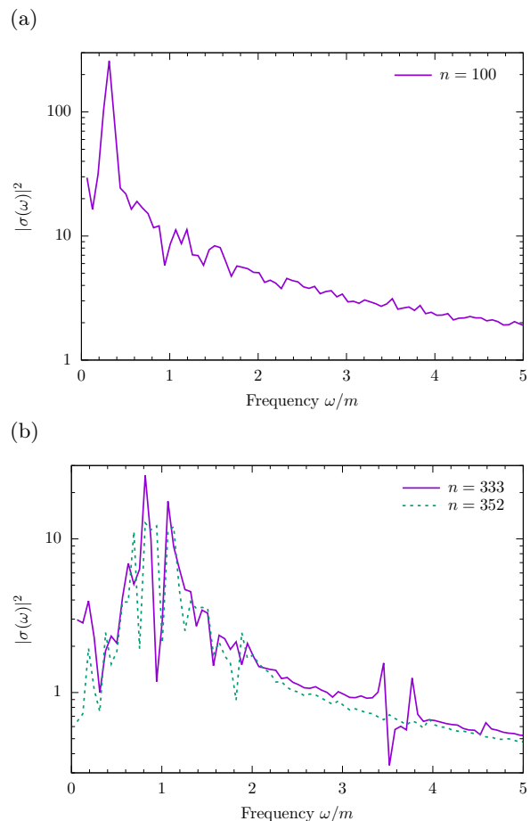
FIG. 16. Power spectrum |\sigma(\omega)|^2 for: (a) the n = 100 rare state; (b) the n = 333, 352 thermalizing states as computed from data in Fig. 15.
