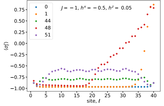
FIG. 18. The spin expectation value \langle \sigma_\ell^z \rangle , on each site \ell = 1, 2, \dots, 40 , for the 0th (ground), 1st, 44th, 48th and 51st states in the spectrum as found using DMRG. These states are marked in Fig. 17(c). The 1st and 48th states are examples of mesons localized on the boundary.
