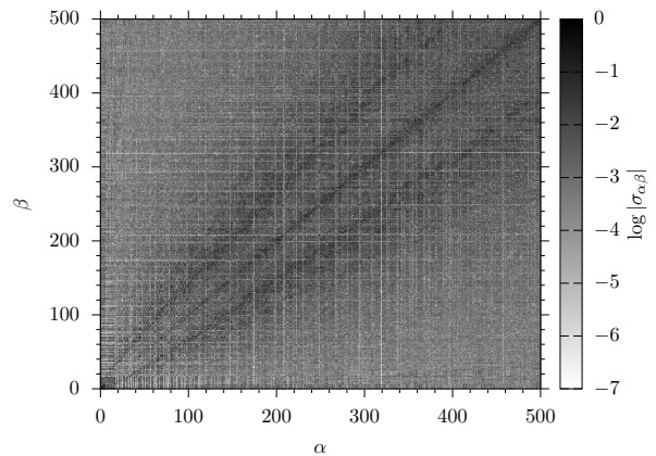
FIG. 4. Off-diagonal matrix elements of the local spin operator |\langle E_\beta | \sigma(0) | E_\alpha \rangle| ( \alpha \neq \beta ) between the first 500 eigenstates constructed with the TSM for m = 1, g = 0.1 and R = 35 , cf. Fig. 2(b). Parameters are m = 1, g = 0.1 . Matrix elements satisfying |\sigma_{\alpha\beta}| < 10^{-7} are plotted as white. Note the visible vertical/horizontal lines are not remnants of the plotting, but show eigenstates that are only coupled very weakly to other states by the spin operator \sigma(0) .
