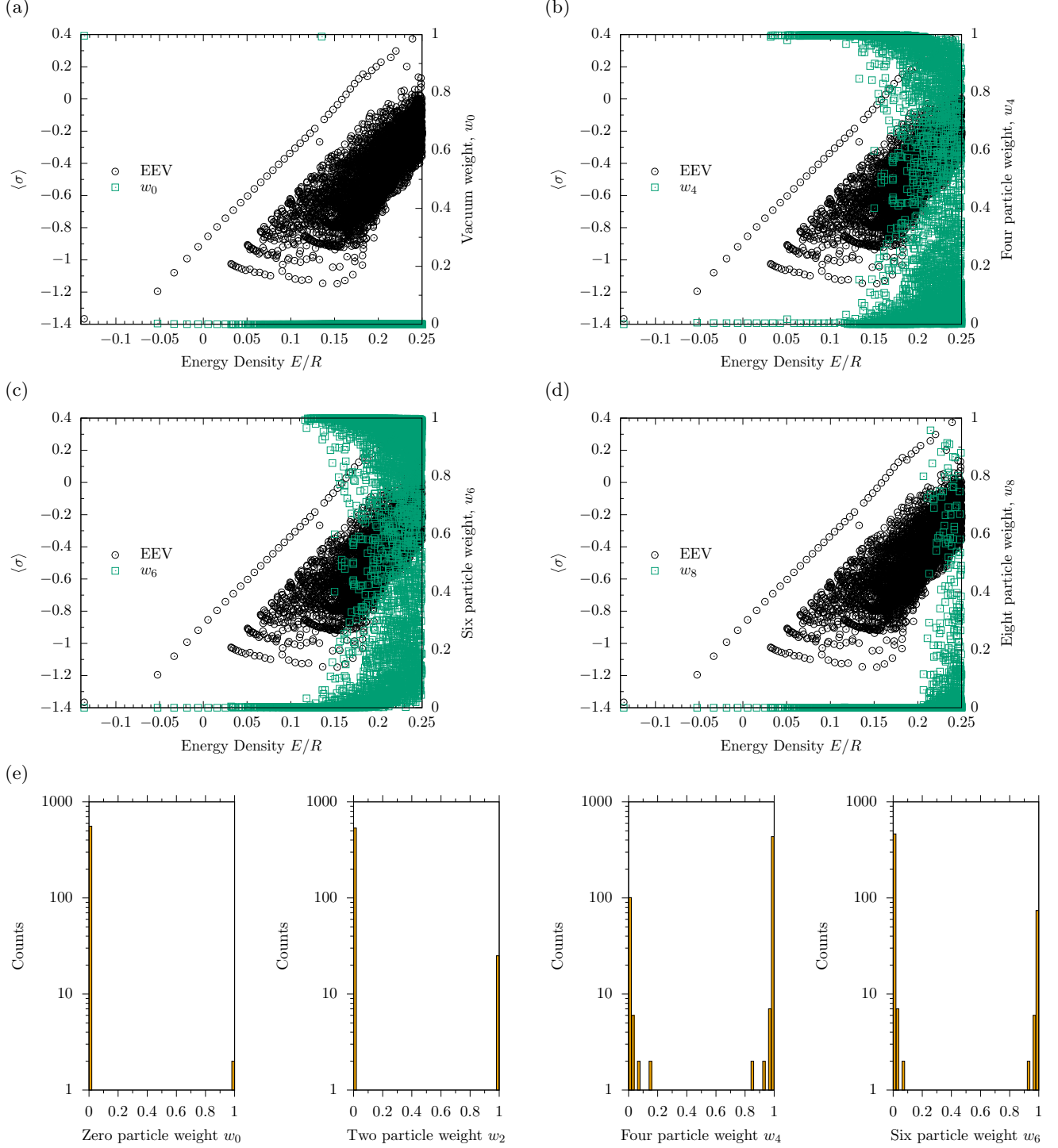
FIG. 25. The weights (a) w_0 ; (b) w_4 ; (c) w_6 ; (d) w_8 . Eigenstates were constructed with the TSM on the length R = 35 chain with m = 1 , g = 0.1 and an energy cutoff E_\Lambda = 10.5 , with up to 10 free fermions in the basis states. These plots illustrate the approximate low-energy U(1) symmetry discussed in the main text: below an energy density of E/R \sim 0.15 , the weight for each state are either w_N \approx 1 or w_N \approx 0 . This is emphasized in (e), where we show the distribution of the weights for eigenstates with energy density E/R < 0.15 , where bins are of width \Delta w_N = 0.02 . We see almost all states have weights close to zero or close to one, with the histograms being bimodal (note the logarithmic y -axis scale). The issue of where this approximate U(1) symmetry breaks is tough to address, with cutoff effects dominating results at higher energies.
