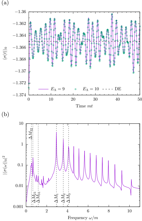
FIG. 13. (a) Time evolution of the local magnetization \langle\sigma(t)\rangle_0 following the quench (m = 1, g = 0.2) \rightarrow (m = 1, g = 0.1) in (2) with R = 25 . Time evolution is computed via TSM+CHEB with cutoff E_\Lambda = 9, 10 and the expansion evaluated to order 2000. The magnetization is oscillating about its diagonal ensemble (DE) value, computed via the TSM, which also coincides with the microcanonical ensemble prediction. (b) The power spectrum of the time evolution. We note a few prominent frequencies in terms of the post-quench confined state energies: \Delta M_{ij} = M_i - M_j and \Delta M_j = M_j .
