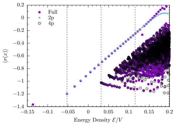
FIG. 11. We compare the results of a full TSM procedure with E_\Lambda = 10.5 (for a system with g = 0.1 , m = 1 of size R = 35 ) to an approximate block diagonalization by fermion number. Two particle states (2p) are considered up to cutoff E_\Lambda = 200 ; four particle states (4p) are considered up to cutoff E_\Lambda = 16 . Dashed lines show the threshold energies for eigenstates containing 1 – 3 mesons (i.e. up to 6 fermions).
