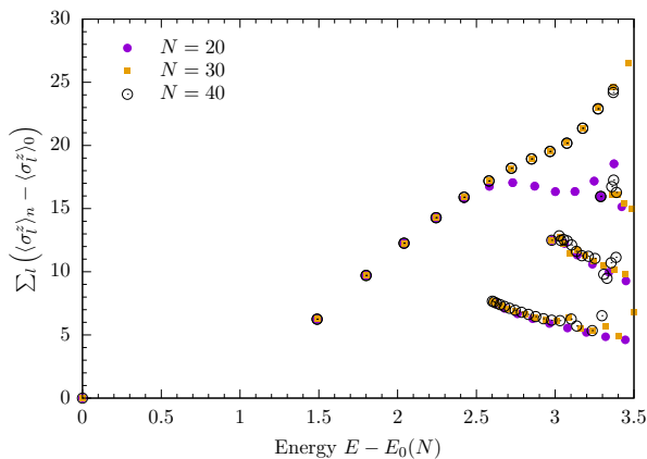
FIG. 19. The EEV spectrum obtained by DMRG on the finite lattice of N sites for the Hamiltonian (33) with J = -1 , h^x = -0.5 and h^z = 0.05 . Here we consider the total magnetization of the eigenstates relative to the ground state, as a function of energy (relative to the ground state energy E_0 ). See Fig. 17 for further details.
