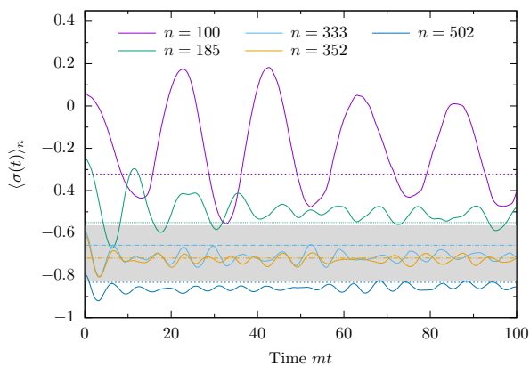
FIG. 15. Time evolution of the local spin operator \sigma(0) following a quench H_i = H(1, 0.1) \rightarrow H_f = H(1, 0.2) computed via TSM+CHEB. Each data set starts from a different eigenstate n of the initial Hamiltonian. Dashed lines denote the diagonal ensemble prediction for the long time limit, whilst the shaded region shows the thermal result from the microcanonical ensemble (with the uncertainty representing the standard deviation of the data averaged over).
