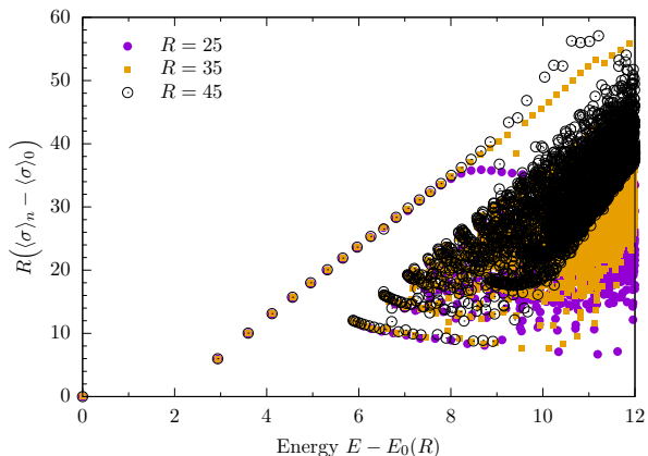
FIG. 20. The EEV spectrum for m = 1 , g = 0.1 in systems of sizes R = 25 - 45 (see Figs. 2 for details). Here we plot the total magnetization (relative to the ground state) as a function of energy (relative to the ground state). We see that the meson states are well converged as a function of system size R , while the thermal continuum is qualitatively converged (in the sense that the features are correct, but the density of state increases with increasing R ). Note the striking similarity to Fig. 19.
