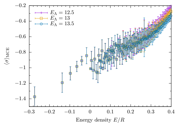
FIG. 24. The MCE prediction for \langle \sigma(0) \rangle at a given energy density in the field theory (2) with m = 1 , g = 0.2 and R = 25 . Error bars denote the standard deviation of the averaged data for the window \Delta E = 0.1 .
