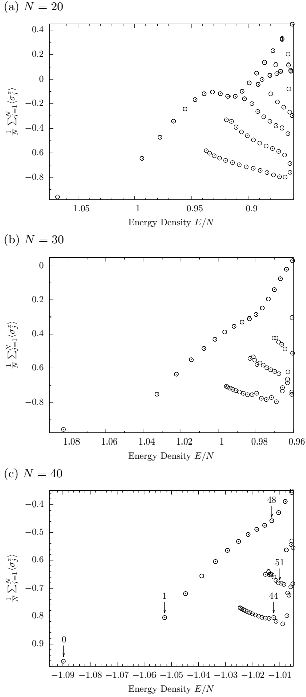
FIG. 17. The eigenstate expectation values for the chain-averaged magnetization \frac{1}{N} \sum_{i=1}^N \langle \sigma_i^z \rangle in the lowest \sim 150 states of the lattice model, Eq. (33), with J = -1 , h^x = -0.5 and h^z = 0.05 . Eigenstates were computed with DMRG for a chain of (a) N = 20 ; (b) N = 30 ; (c) N = 40 sites. We encourage the reader to compare this to the analogous plot in the scaling limit, Fig. 2, and note the striking similarity. In plotting (a), (b), we exclude the false vacuum state. The labels in (c) indicate the states shown in Fig. 18.
