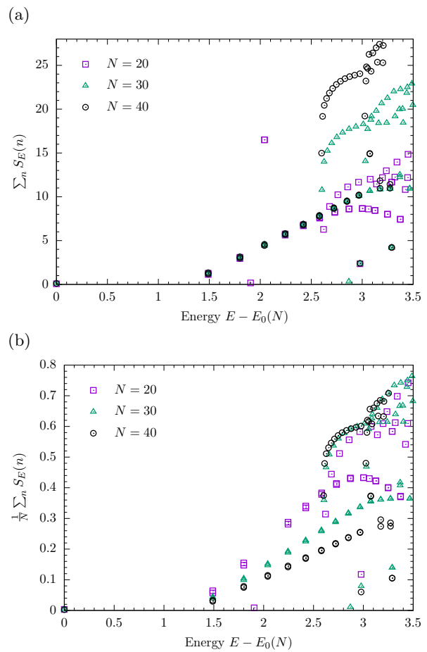
FIG. 21. (a) The entanglement entropy averaged over bipartitions of the system, \sum_n S_E(n) , in each eigenstate of energy E relative to the ground state, for the lattice model (33) with J = -1 , h^x = -0.5 and h^z = 0.05 . Data is presented for three different system sizes N . We see that there are two classes of states: those that have N -independent entanglement (i.e. area law states) and those with volume law entanglement (linear in N ). The presence of volume law entanglement states is shown more clearly in (b), where we scale the bipartition averaged entanglement by dividing through by the volume N . The nonthermal states have area law entanglement, while the thermal states have volume law.
