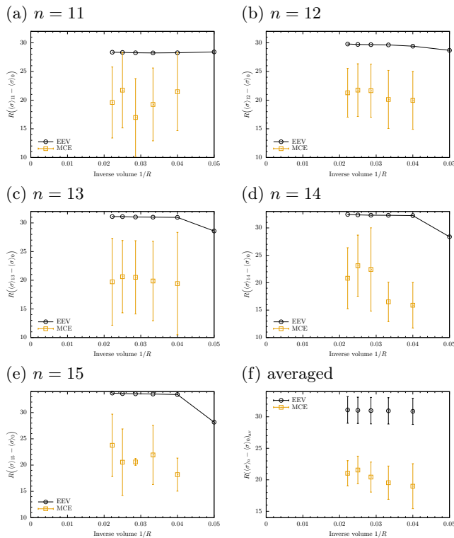
FIG. 3. (a)–(e) The finite size scaling the total magnetization R\langle\sigma\rangle of the n = 11 - 15 rare states (EEV), compared to the MCE prediction. (f) The average magnetization of the n = 11 - 15 rare states compared to that predicted by the average of the MCE results. Clearly the rare states and their proximate thermal states have different magnetization, and this persists to the R \rightarrow \infty limit. In all cases, error bars show the standard deviation of the data averaged over. Note that R(\langle\sigma\rangle_n - \langle\sigma\rangle_0) measures the number of overturned spins in the n th meson as compared to the (ordered) ground state.
