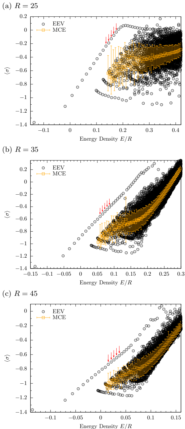
FIG. 2. Comparison of the eigenstate expectation values (EEV, black) of the local magnetization \sigma with the microcanonical ensemble prediction (MCE, orange) for eigenstates at energy density E/R in the Ising field theory (2) with m = 1 , g = 0.1 on the ring of size (a) R = 25 ; (b) R = 35 ; (c) R = 45 . Eigenstates are constructed via the TSM with an energy cut-off of (a) E_\Lambda = 13.5 ; (b) E_\Lambda = 10.5 ; (c) E_\Lambda = 9 . States containing up to ten particles are considered in the truncated Hilbert space. The MCE is constructed by uniformly averaging over an energy window of size \Delta E = 0.1 , with error bars denoting the standard deviation. The red arrows highlight the nonthermal states considered further in Fig. 3.
