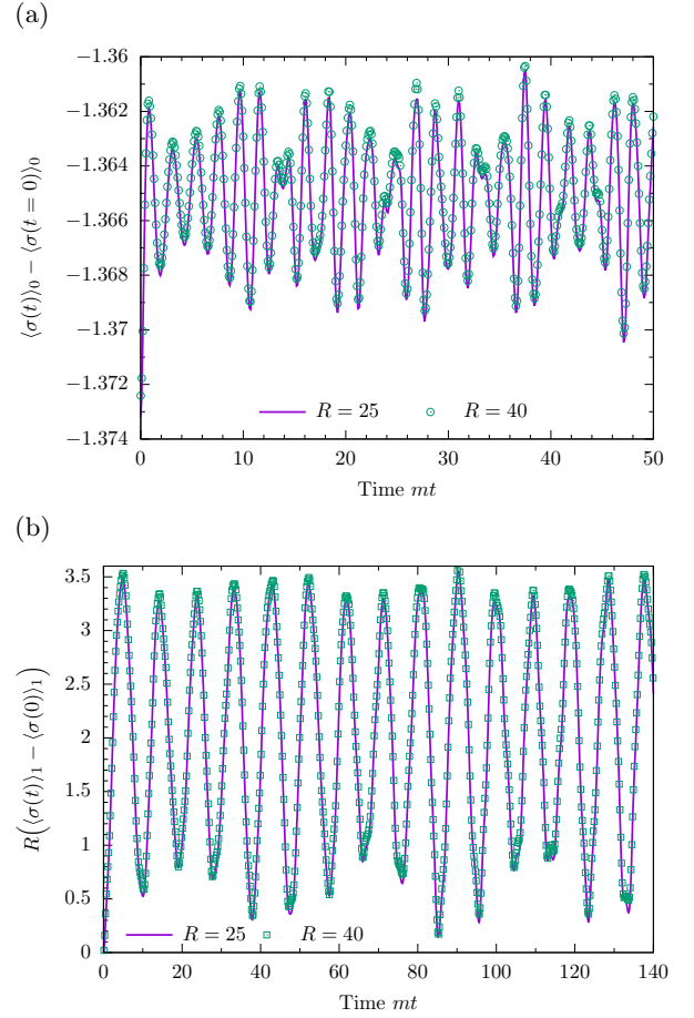
FIG. 27. Time evolution via the N_{\max} = 2000 -order Chebyshev expansion for the quantum quench (m, g) = (1, 0.1) \rightarrow (1, 0.2) of (2) for R = 25, 40 . We start from the (a) ground state; (b) first excited state of the initial Hamiltonian, computed via the TSM with an energy cutoff E_\Lambda = 9 . Good agreement of the results is seen until t \sim 145 (not shown in (a)), where the finite order of the Chebyshev expansion causes the results for the large system size to breakdown.
