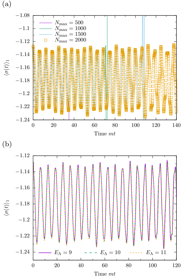
FIG. 26. (a) Time evolution via the N_{\max} -order Chebyshev expansion for the quantum quench (m, g) = (1, 0.1) \rightarrow (1, 0.2) of (2) for R = 25 . We start from the first excited state of the initial Hamiltonian, computed via the TSM with an energy cutoff E_\Lambda = 9 . The breakdown time t_{\text{br}} is seen by the divergence of the result from higher order predictions, see the purple line at mt \sim 35 , the green line at mt \sim 70 and the cyan line at mt \sim 110 . (b) Time evolution shown for three values of E_\Lambda with N_{\max} = 2000 . We see that the energy cutoff plays only a small role in the convergence of the presented results.
