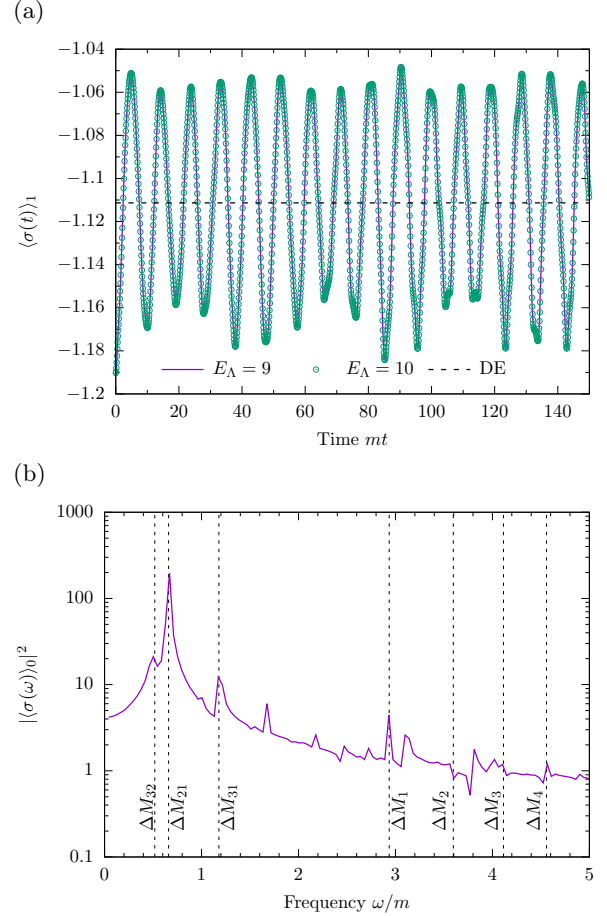
FIG. 14. (a) Time evolution of the local magnetization \langle\sigma(t)\rangle_1 when starting from the first excited state of (2) for the same quench described in Fig. 13. (b) The associated power spectrum. We note a few prominent frequencies in terms of the post-quench confined state energies: \Delta M_{ij} = M_i - M_j and \Delta M_j = M_j .
