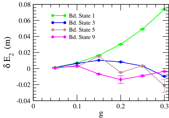
FIG. 9. The second order correction to the energy (measured relative to the ground state) as a function of longitudinal field strength g for four mesons (the first, third, fifth and ninth ordered by energy) arising from mixing with zero and four domain wall fermion states. Error bars denote uncertainties in extrapolating to the infinite volume.
