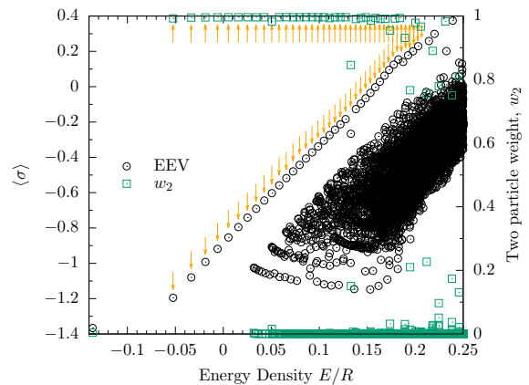
FIG. 6. The two particle weight w_2 (20) and the eigenstate expectation values of the local magnetization operator \langle\sigma\rangle in the field theory (2) with m = 1 , g = 0.1 on the ring of size R = 35 . Eigenstates are constructed with the TSM for an energy cutoff of E_\Lambda = 10.5 and a maximum of ten particles in the basis states. Arrows (upper and lower) are drawn at the energies of the first forty confined states, M_n , as computed in Appendix C. Higher particle weights, as well as histograms of their distributions, are provided in Appendix B.
