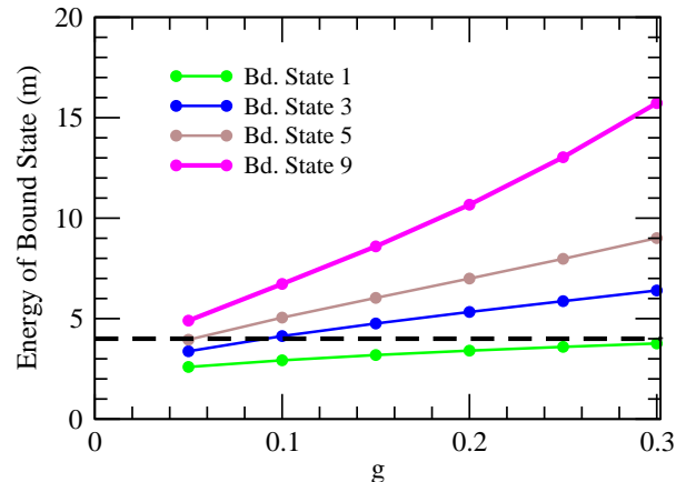
FIG. 10. The energies as a function of longitudinal field strength g for four mesons (the first, third, fifth and ninth ordered by energy) whose energy corrections are given in Fig. 9. The dashed line marks the 4m threshold. Once the energy of the meson crosses this threshold, we no longer expect the energy of hybridization with the vacuum and four particle states to increase monotonically with increasing g .
