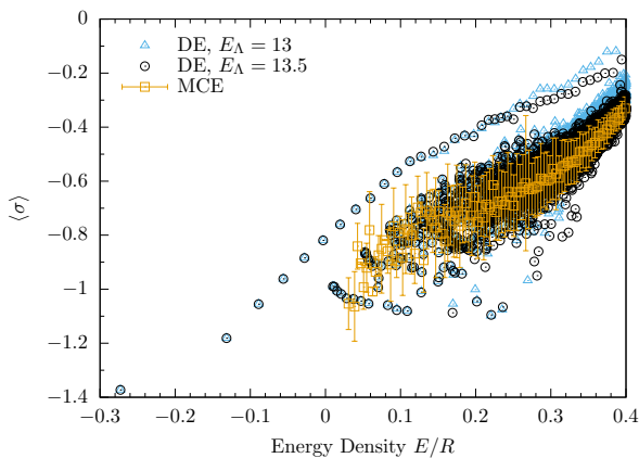
FIG. 12. The diagonal ensemble (DE) result for long-time expectation values and the microcanonical ensemble (MCE) prediction following the sudden quench ( m = 1, g = 0.1 ) \rightarrow ( m = 1, g = 0.2 ) in the field theory (2). Each data point corresponds to starting from a different low energy eigenstate of the initial Hamiltonian, m = 1, g = 0.1 . In all cases, results are on a system of size R = 25 and with energy cutoff E_\Lambda . We note that E_\Lambda = 13 ( E_\Lambda = 13.5 ) corresponds to 23, 238 (32, 149) computational basis states. The MCE is computed by averaging an energy window of size \Delta E = 0.1 , and error bars denote the standard deviation of data averaged over.
