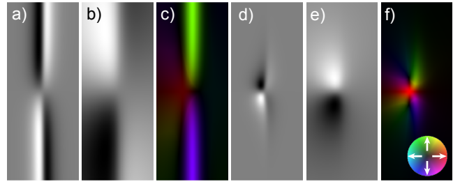
FIG. 4: a & d) Fresnel mode LTEM, b & e) phase map, and c & f) in-plane magnetic induction map of a a - c) vertical Bloch line ( D = 0 \text{mJ/m}^2 ) and d - f) DW Skyrmion ( D = 0.5 \text{mJ/m}^2 ) calculated from the micromagnetic output of figures 2f and 2i.
