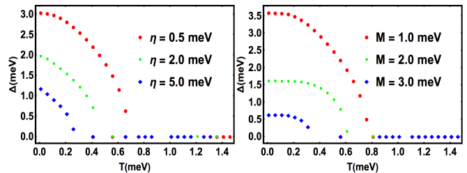
FIG. 3. Temperature dependence of the superconducting gap for \lambda = 5 meV. (Left) as a function of the dissipation parameter \eta and M = 1 meV. (Right) As a function of the mass parameter M and \eta = 0.1 meV. The BCS ratio \frac{\Delta(0)}{T_c} increases (decreases) with the dissipation (mass) parameter.
