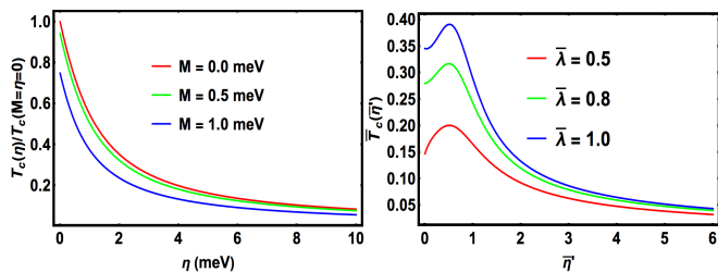
FIG. 2. (Left) Superconducting critical temperature T_c (normalized to its value at M = \eta = 0 ) as a function of the dissipation parameter \eta for different masses M when the mediator is local. The coupling constant \lambda is chosen to be equal to 1 meV. (Right) The case when the mediator is non-local for M = 0 : plot of the dimensionless \bar{T}_c = T_c/\kappa as a function of \bar{\eta}' = \eta'/\kappa for different dimensionless coupling strengths \bar{\lambda} = \lambda/\kappa^2 . The peak in T_c is set by \kappa , the energy scale associated with bosonic velocity.
