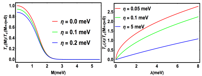
FIG. 1. Effect of a local dissipative mediator: (Left) Superconducting critical temperature T_c (normalized to its value at M = \eta = 0 ) as a function of the mass parameter M . The coupling constant \lambda is chosen to be equal to 1 meV. (Right) Same quantity now plotted as a function of the coupling constant \lambda for M = 0.1 meV. A crossover from T_c \sim \sqrt{\lambda} to T_c \sim \lambda occurs as a function of \eta .
