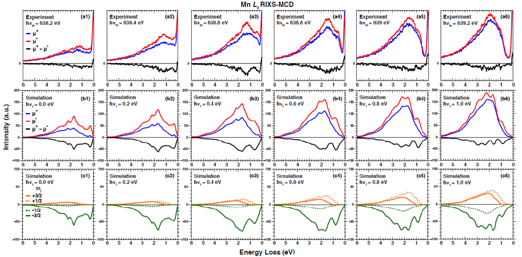
FIG. 4 RIXS and RIXS-MCD spectra for Mn L_3 -edges. Figures (a1)-(a6) show the experimental RIXS results for the \mu^+ and \mu^- configurations and their MCD spectra for the Mn L_3 -edge as a function of the energy loss. Theoretically calculated RIXS and RIXS-MCD spectra based on DFT calculation are in (b1)-(b6). The definition of h\nu_1 is given in the text. Figures (c1)-(c6) show m_j resolved RIXS-MCD spectra for Mn L_3 -edge, and the summation of the whole components of these spectra corresponds to the RIXS-MCD spectra in Figs. (b1)-(b6).
