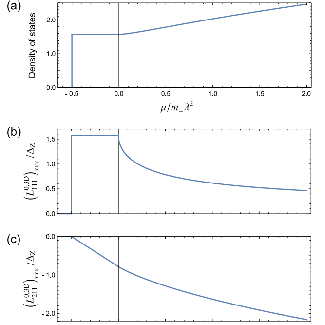
FIG. 2. For BiTeX( X=I,Br ), (a) the density of states in unit of \sqrt{m_{\perp}^3 m_{\parallel}}\lambda/\pi^2 , (b) the three-dimensional nonlinear electric conductivity (L_{111}^{0,3D})_{xxx}/\Delta_Z (proportional to the thermoelectric conductivity (L_{122}^{3D})_{xxx}/\Delta_Z ) in unit of 3e^3\tau^2\sqrt{m_{\parallel}/m_{\perp}}/16\pi^2(1+i\omega\tau) , and (c) the three-dimensional nonlinear thermoelectric conductivity (L_{211}^{0,3D})_{xxx}/\Delta_Z (proportional to the thermal conductivity (L_{222}^{3D})_{xxx}/\Delta_Z ) in unit of 3e^2\tau^2\lambda^2\sqrt{m_{\perp}m_{\parallel}}/8\pi^2(1+i\omega\tau) are plotted as functions of the chemical potential \mu in unit of m_{\perp}\lambda^2 . All quantities are estimated in the limit of the vanishing magnetic field ( \Delta_Z \rightarrow 0 ).
