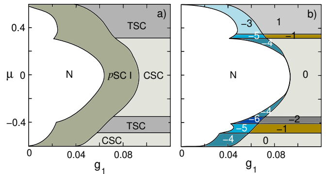
Figure 3. (Color online) Mean field phase diagram as a function of the chemical potential \mu and intra-orbital pairing coupling g_1 , both in eV units. The phase diagram does not depend on g_2 for g_2 \lesssim 0.1 eV (see Fig 2). a) Normal phase (N), p_x superconducting phase ( p SC I), chiral p + ip state (CSC) and topological p + ip phase (TSC). b) Possible topological phases in the chiral p + ip channel. The integers indicate the corresponding BdG Chern number \mathcal{N} . For fixed g_1 , the system has a sequence of topological phase transitions near the van-Hove singularities of the band, where the topology of the Fermi surface changes. The blue regions correspond to the weak coupling gapped p + ip phases, which are topological. Gray and maroon regions: strong coupling phases. In mean field, the gapped p + ip state wins over the non-chiral p state in the strong coupling sector.
