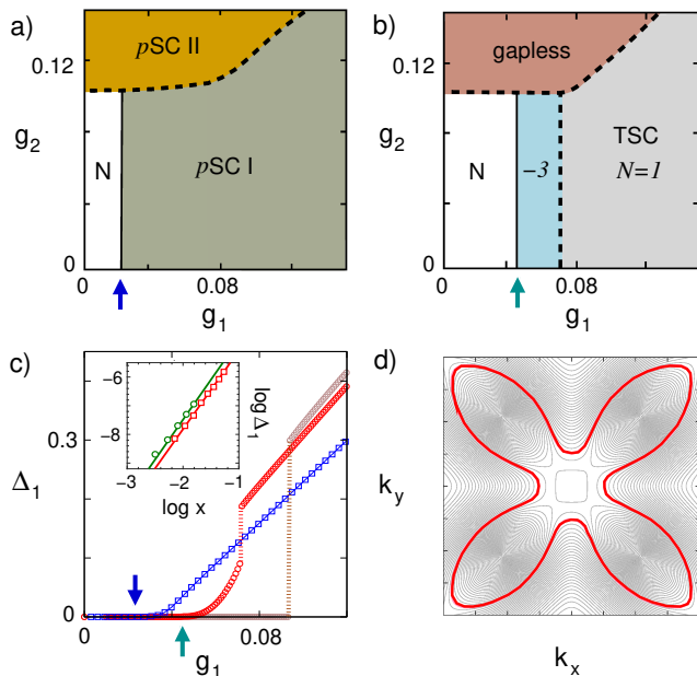
Figure 2. (Color online) Phase diagram for a) p -wave and b) p + ip state for intra-orbital ( g_1 ) and inter-orbital ( g_2 ) couplings at \mu = 4t/3 = 0.4 eV. g_1 and g_2 in eV units. Green area: intra-orbital p -wave ( p SC I) for g > \tilde{g}_{1c}(\mu) . Yellow: inter-orbital p -wave ( p SC II). Gray area: strong coupling topological phase (TSC) with Chern number \mathcal{N} = 1 ; Light blue: gapped weak coupling one ( \tilde{g}_{1c} < g < g_{1c} ) with \mathcal{N} = -3 (see Fig. 3b). Light red: gapless p + ip , which is topologically trivial. Dashed lines: first order phase transitions. Solid black lines: second order transition (blue and green arrows). c) Scaling of \Delta_1^C vs g_1 . Red and brown circles: p + ip for \mu = 0.4 , and 0, respectively. Blue square: p -wave for \mu = 0.4 eV. Green and blue arrows: critical coupling \tilde{g}_{1c} \approx t/7 = 0.045 eV and \tilde{g}_{1c} \approx t/12 = 0.025 eV respectively for \mu = 0.4 eV. Inset: \Delta_1^C vs \log x , with x = (1 - \tilde{g}_{1c}/g) , showing power law scaling in the chiral phase near \tilde{g}_{1c}(\mu) . Green dots: \mu = 0.3 eV. Red: \mu = 0.4 eV. d) Brillouin zone. Red line: anisotropic Fermi surface at \mu = 0.33 eV.
