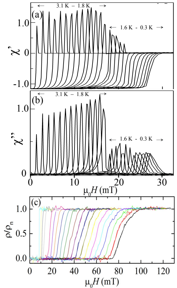
FIG. 8. Real component, \chi' (a), and imaginary component, \chi'' (b) of the magnetic susceptibility of a polycrystalline bar of AuBe plotted against H for a series of constant temperatures in the range 3.1 \text{ K} \geq T \geq 0.3 \text{ K} . Field sweeps in the temperature range 0.3 - 1.6 \text{ K} were done in the ^3\text{He} cryostat, while those in the range 1.8 - 3.1 \text{ K} employed the MPMS. The jump in peak magnitudes between 1.6 K and 1.8 K is caused by a difference in drive amplitude. (c) Isothermal resistivity data, shown as resistivity, \rho , divided by the low-temperature normal-state resistivity, \rho_n , versus magnetic field H . The data were recorded at a series of approximately equally spaced temperatures covering the range 3.0 \text{ K} \geq T \geq 0.3 \text{ K} .
