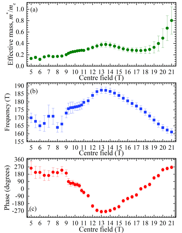
FIG. 5. Magnetic-field dependence of parameters describing the F \approx 170 T series of dHvA oscillations: (a) effective mass m^* , (b) frequency F and (c) phase \mathfrak{N} (see Equation 7) of the oscillations. The field dependences of these parameters are derived from Fourier analysis of dM/dH data using inverse field windows of \frac{1}{24} \text{T}^{-1} width symmetrically disposed (in inverse field) about the centre field ( B_m ) values given on the lower axis.
