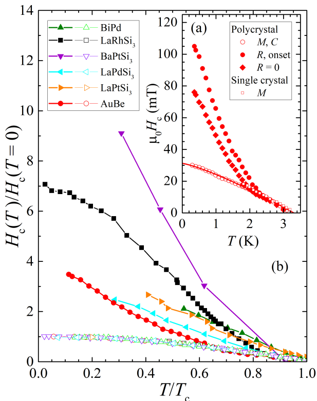
FIG. 9. (a) [inset] Critical fields versus temperature for AuBe. The solid symbols are critical fields measured using resistivity [circles = onset of resistive transition, diamonds = highest field at which zero resistance occurs], whilst the hollow symbols represent critical fields derived from thermodynamic probes (magnetization, susceptibility and heat capacity). Data from the magnetization of a small single crystal are shown as hollow squares. (b) Analogous phase diagram for a representative collection of NCSs, presented in reduced units H_c/H_c(T=0) , T/T_c . Here, H_c(T=0) is derived from standard BCS fits to critical fields derived from thermodynamic probes. As in (a), open symbols represent thermodynamic critical fields and filled points are resistive critical fields. Data for the various NCSs are from the following sources: AuBe (this work), BiPd [66], LaRhSi 3 [60], BaPtSi 3 [61], LaPdSi 3 [56], LaPtSi 3 [56].
