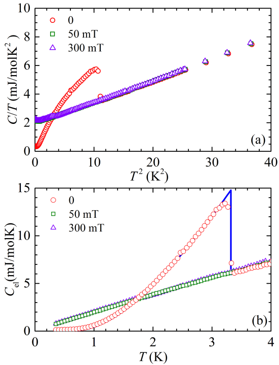
FIG. 6. (a) Heat capacity C of AuBe, divided by temperature T , plotted as a function of T^2 at fields \mu_0 H = 0, 50 , and 300 mT. The transition to the superconducting state is marked by the near-vertical jump close to T^2 = 10 K 2 in the H = 0 data set. (b) The low-temperature electronic component of the heat capacity versus T at fields of \mu_0 H = 0, 50 , and 300 mT. The curve is a fit to the standard BCS model for an isotropic, fully-gapped superconductor in the weak-coupling limit 44 .
