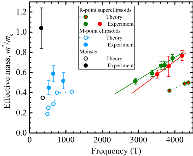
FIG. 4. Solid points represent effective masses derived using Equation 4 versus corresponding experimental dHvA frequencies. The error bars are the uncertainties given by the Simplex fitting routine and the different coloured points and guide lines are explained in the text. Masses and frequencies corresponding to a selection of predicted extremal orbits from the bandstructure calculations (including spin-orbit interactions) are shown as hollow points. The hollow light-blue points (calculated for \mathbf{H}||[100] ; dotted line is a guide to the eye) correspond to the hole ellipsoids centred on the zone-edge M-points [Figure 3(b)]. The hollow green, red-filled points (calculated for \mathbf{H}||[100] ) are from the two electron approximate superellipsoids centred on the zone-corner R-points [Figure 3(c, e)]. The black, hollow point corresponds to a possible “monster” extremal orbit [Figure 3(d)].
