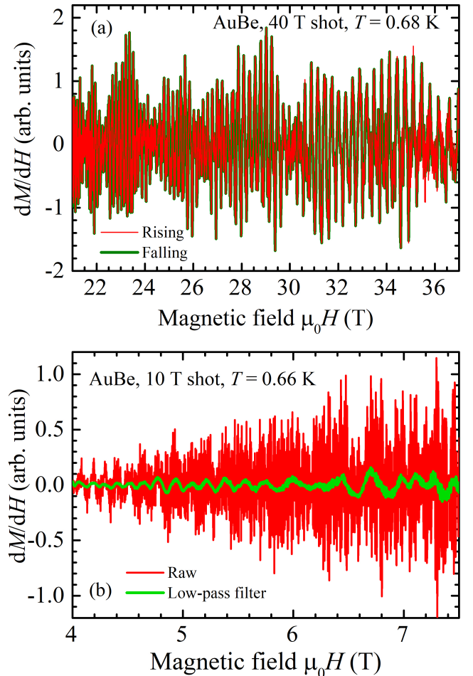
FIG. 1. (a) The differential susceptibility, dM/dH , plotted versus magnetic field \mu_0 H for a polycrystalline AuBe rod at T = 0.68 \text{ K} , recorded during a 40 T pulsed-magnet shot. Several different series of dHvA oscillations are visible. Data for both rising and falling fields are shown. The “fur” on the data is not noise, but comprises the “belly” orbit dHvA oscillations from the copper of the susceptometer coil. (b) The red trace shows dHvA oscillations recorded using a 10 T pulsed magnet shot ( T = 0.66 \text{ K} ) where the sample is the same as that used in (a). The green curve represents the application of a low-pass filter to the red trace; this removes the higher-frequency de Haas-van Alphen oscillations so that the lower-frequency series can be seen more readily.
