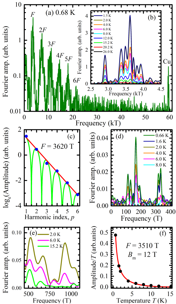
FIG. 2. (a) Fourier spectrum (20 – 38 T window) of the data in Figure 1(a) plotted with a logarithmic amplitude scale. A band of several series of dHvA oscillations (labelled F ) and their higher harmonics (labelled 2F .... 6F ) are clearly visible, along with a peak at 59.5 kT due to the belly orbits in the Cu coil of the susceptometer. (b) [Inset] Fourier transforms (linear amplitude scale) of data from 40 T pulses recorded at a series of higher temperatures T = 1.5 - 26 K. The same field window as in (a) has been applied. The frequency range has been chosen to show just the fundamental frequencies in the band of oscillations labelled F in (a). (c) Logarithmic amplitudes (points) of the harmonics of the F = 3620 T series of dHvA oscillations versus harmonic index p ; the red line is a guide to the eye, showing an approximate linear decrease with p . The green curve is a fit of Equation 2 for gm^* = 2 . (d) Fourier transforms of dHvA oscillations from a series of 10 T pulsed-magnet shots at temperatures T = 0.66 - 8.0 K. (e) Field-axis expansion of Fourier transforms (linear amplitude scale) of data from 40 T pulses for three example temperatures, showing frequencies in the range 490 – 1200 T. The same field window as in (a) has been applied. (f) (Fourier amplitude)/ T versus temperature for the F = 3510 T series of dHvA oscillations. The data window was centred on B_m = 12 T. The red line is a fit of Equation 4 to the data, yielding m^* = 0.58 \pm 0.04m_e .
