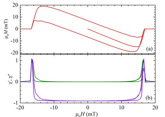
FIG. 7. (a) The dc magnetization M (red) versus field H at a temperature of T = 1.8 K. Sharp transitions and a small supercooling, evident in the hysteresis of the critical field, are apparent in M(H) . (b) The real component \chi' (purple) and the imaginary component \chi'' (green) of the ac magnetic susceptibility versus H , again at T = 1.8 K.
