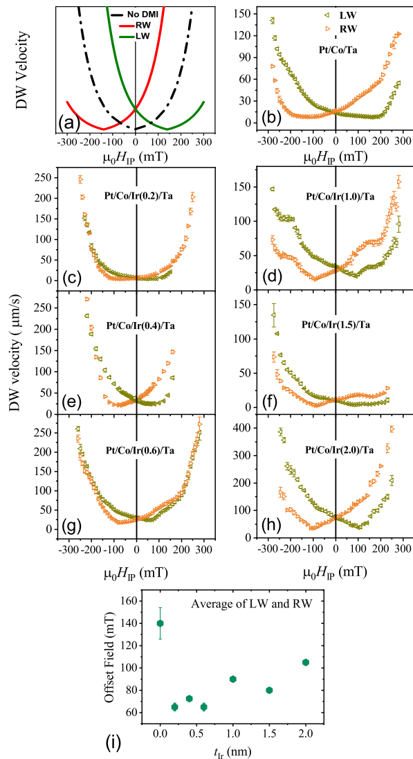
FIG. 5. Variation of DW velocity v with IP field H_{IP} for left- and right-moving DWs, LW and RW, respectively. (a) Simulated from Eq. 3. When there is no DMI, v_{DW} has a minimum at zero in-plane field and rises symmetrically for opposite field directions. When DMI is present the minimum point is shifted to \pm H_{offset} depending on the direction of the DMI vector inside the wall. (b)-(h) Experimental data for left wall (green triangles) and right wall (orange triangles) for multilayers with different t_{Ir} . A lack of symmetry around the minimum points is obvious in most cases. (i) Average H_{offset} as a function of t_{Ir} .
