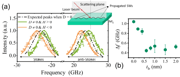
FIG. 7. Brillouin light scattering. (a) Normalized BLS spectra measured for Pt/Co/Ta at two equal and opposite applied fields of \sim 1 T in orange and green. The black dashed line shows what is expected in case that there is no DMI in the sample. Symbols refer to experimental data and solid lines are Lorentzian fits. The panel at the top represents the Damon-Eshbach geometry which was used for measurements presented in this work. (b) Frequency shift \Delta f against Ir thickness t_{Ir} .
