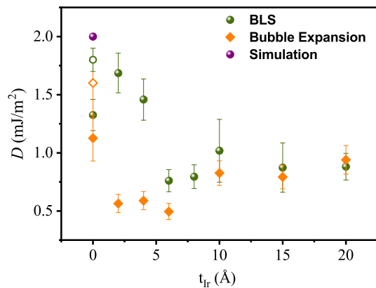
FIG. 10. Comparison of DMI results for the series of samples. Orange diamonds circles are the results obtained from taking the field of minimum asymmetric bubble expansion velocity as H_{DMI} . Green circles are the results from BLS. For t_{Ir} = 0 the open shapes show the D value for BLS and bubble expansion when the measured M_s is substituted with the average value of other samples ( i.e. excluding the dead layer effect)
