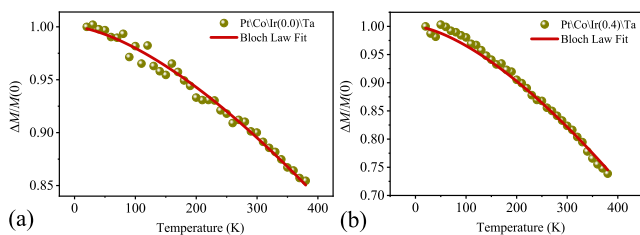
FIG. 11. Temperature dependence of magnetization in (a) Pt/Co/Ta and (b) Pt/Co/Ir(0.4)/Ta multilayers. The red line shows the Bloch law fit in each case.
