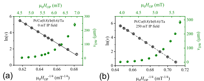
FIG. 12. Investigation of creep propagation of the DWs in a bubble domain for t_{Ir} = 0.6 nm. (a) Without any applied in-plane field and (b) in the presence of a high in-plane field: \mu_0 H_x = 250 mT. In both cases the creep scaling law is well-obeyed.
