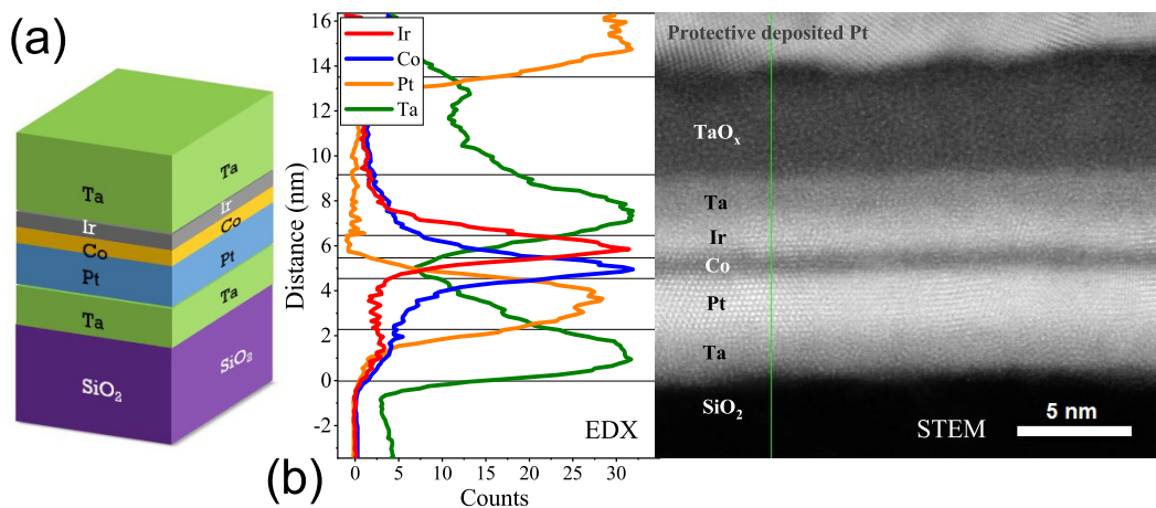
FIG. 1. Magnetic multilayer structure. (a) Schematic of the multilayer stack, nominally Ta(2.0)/Pt(2.2)/Co(0.8)/Ir( t_{\text{Ir}} )/Ta(4.0) (layer thicknesses in nm). (b) EDX elemental line profiles across the multilayer structure with 1.0 nm Ir alongside a HAADF image of the same sample. The different interfaces and a smooth growth of the layers are clearly visible.
