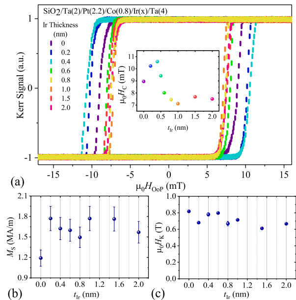
FIG. 2. Magnetic characterization. (a) Polar Kerr measurements show clear square-shaped hysteresis loops confirming strong PMA. The probed area is the size of our unfocussed laser spot, which is of millimeter scale. (b) Saturation magnetization M_S and (c) anisotropy field H_K as a function of Ir thickness t_{Ir} , both are determined from hysteresis loops acquired by SQUID-VSM with an in-plane field.
