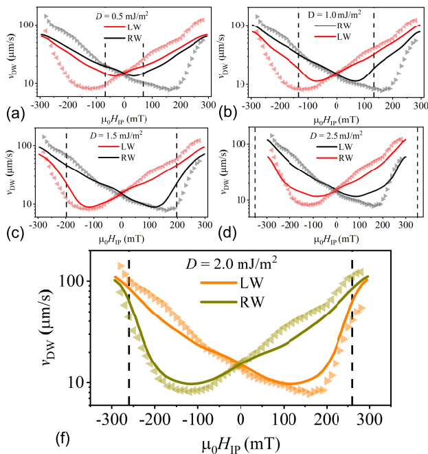
FIG. 9. Domain wall velocity, v , as a function of in-plane applied field, H_{IP} , for four different values of the DMI constant, D : (a) 0.5 \text{ mJ/m}^2 , (b) 1.0 \text{ mJ/m}^2 , (c) 1.5 \text{ mJ/m}^2 , (d) 2.5 \text{ mJ/m}^2 , and (f) 2.0 \text{ mJ/m}^2 . The triangles represent experimental data for the Pt/Co/Ta system (Fig. 5). The dashed vertical lines represent the DMI field extracted from simulation.
