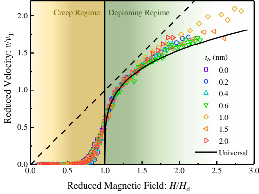
FIG. 4. Reduced velocity vs. reduced field for different Ir thicknesses t_{Ir} , showing a good universal collapse of the curves. The tilted dashed line represents the linear flow regime in which v/v_T = H_{OP}/H_d . The vertical solid line separates the creep and depinning regime. The solid curve marks the universal depinning transition which is conforming to all experimental data in 1 < H_{OP}/H_d < 1.5 range. All the samples leave the universal depinning regime at some point after H_{OP}/H_d \approx 1.5 and begin to approach the flow regime.
