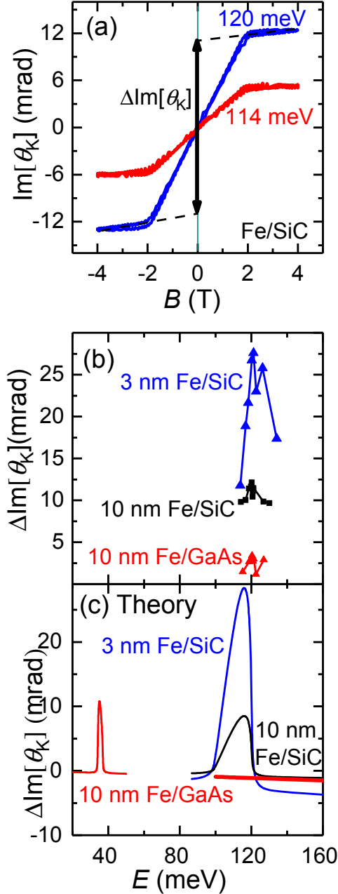
Fig. 2(a) Magnetic field dependence of \text{Im}[\theta_K] for Fe film on SiC, measured at photon energies of 114 and 120 meV. (b) Photon energy dependence of the intercept \Delta\text{Im}[\theta_K] measured for various thickness and substrate. (c) Calculated Kerr angle lineshapes for iron films on SiC and GaAs.
