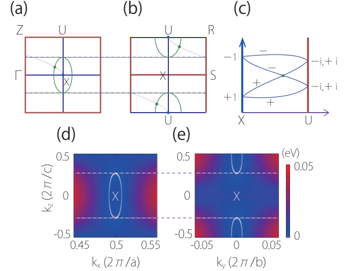
FIG. A2: Schematic figures showing that the neck point in the hourglass dispersion traces out Weyl loops on (a) k_y = 0 plane and (b) k_x = \pi plane. (c) Schematic view of hourglass dispersion along X - U . The labels indicate the eigenvalues of \tilde{\mathcal{M}}_x . (d)(e) Shape of the Weyl loops from the DFT calculations, (d) on the k_y = 0 plane and (e) on the k_x = \pi plane, respectively. The color map indicates the local gap between the two crossing bands.
