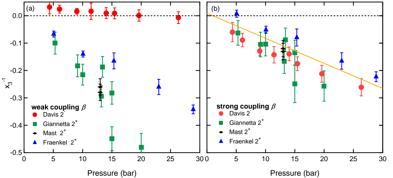
FIG. 2. f -wave interaction strength, x_3^{-1} , calculated using data from Davis et al. 25 , Fraenkel et al. 11 , Giannetta et al. 10 , and Mast et al. 9 . The results in the left panel were calculated from Eqs (7) and (8) using the weak-coupling limits of a_j^c . The right panel incorporates strong-coupling corrections, which brings all four experiments into better agreement. A linear fit (orange solid line) through the entire dataset, weighted by uncertainties, yields a pressure dependence for the f -wave interaction strength reasonably consistent with all experiments.
