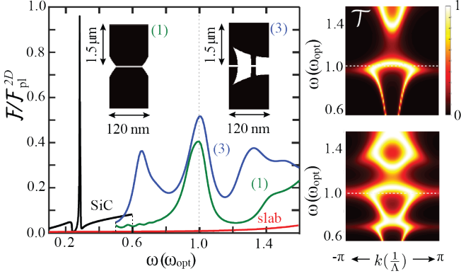
FIG. 1. Inverse design of selective near-field heat transfer between periodic tungsten gratings: Near-field RHT enhancement for inverse-designed tungsten gratings \mathcal{F} , along with that of planar silicon carbide for comparison, relative to the enhancement achieved with ideal (lossless) planar metals, \mathcal{F}_{\text{pl}}^{2D} given in (3), with respect to frequency \omega (left). Profiles of the structures are displayed as insets. Color plots depicting the k -dependent transfer functions \mathcal{T}(\omega, \mathbf{k}) over the chosen frequency range are shown on the right. The depicted optimization proceeds from an unstructured planar system (0) to structured gratings (N) by successively introducing additional ellipsoidal degrees of freedom “N” to the design space. Performance is qualified by the magnitude of RHT at a single design frequency \omega_{\text{opt}} = 2\pi c/3 \mu\text{m} ( \lambda_{\text{opt}} = 3 \mu\text{m} ), where tungsten behaves as a highly lossy metal far from the planar surface plasmon resonance. The gap separation and the period of gratings are d(\Lambda) = 0.02 (0.04) \lambda_{\text{opt}} , respectively. Even in the case of a single ellipsoid, producing a relative simple grating, heat transfer is enhanced by a factor of 40, while the more complicated design (3) is observed to come within 50% of the ideal planar limit.
