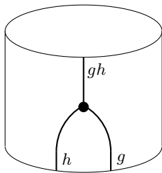
Figure 1: fusion of domain walls
