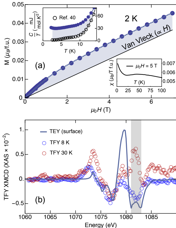
FIG. 3. Bulk properties of nominally pure \text{SmB}_6 sample. (a) The magnetization data is fit by a Van Vleck contribution (solid black line) and a paramagnetic impurity contribution (shaded) of 1% impurities with \mu_{\text{eff}} = 5.2 \mu_{\text{B}} . Insets show susceptibility taken at 5 T and heat capacity with comparison to the previously published heat capacity of a high-purity sample.[40] We attribute shaded portions to impurities. Sample data also appears in the supplementary information of Ref. [19], without fitting. (b) TFY XMCD (bulk). At 8 K, a negative dichroic feature develops from 1081 eV - 1083 eV as for TEY. The temperature dependence counter-indicates solely \text{Sm}^{2+} .
