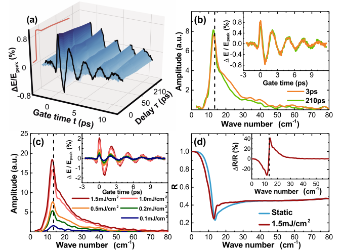
FIG. 2. Photoexcitation-induced changes at 5K. (a) The relative change of the reflected THz electric field \Delta E(t, \tau)/E_{peak} at 5 K at different decay time \tau after excited by 1.28 \mu\text{m} pulses at fluence of 0.5 \text{ mJ/cm}^2 . The red line shows the decay of \Delta E(t=0\text{ps}, \tau)/E_{peak} . The black lines indicate \Delta E(t, \tau = 3\text{ps})/E_{peak} and \Delta E(t, \tau = 210\text{ps})/E_{peak} . (b) Inset: the photoexcitation-induced relative change \Delta E(t, \tau)/E_{peak} in time domain at \tau=3 ps and 210 ps. Main panel: the Fourier transformed spectrum of \Delta E(\omega, \tau) . (c) Inset: fluence dependence of \Delta E(t, \tau)/E_{peak} . Main panel: the Fourier transformed spectrum. (d) R(\omega) before and after excitation by 1.5 \text{ mJ/cm}^2 pulses. Inset shows the ratio of the reflectivity change relative to the static values. The penetration depth mismatch is not considered here.
