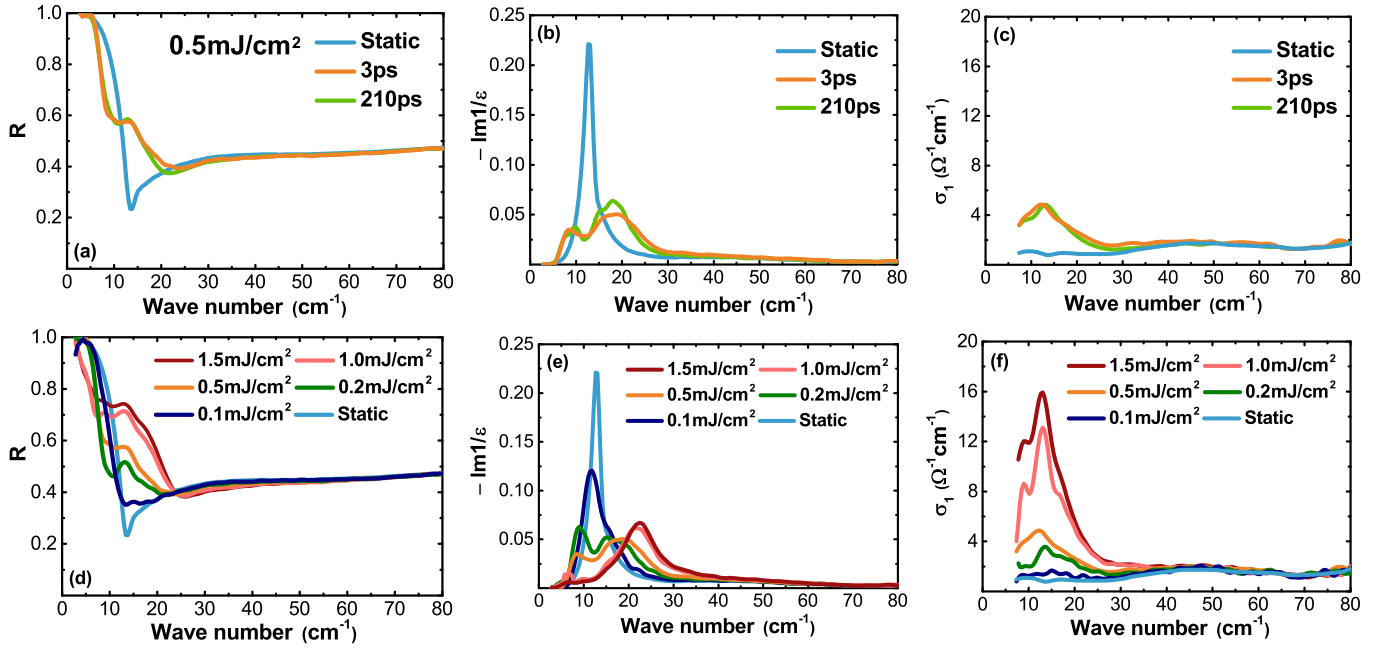
FIG. 3. Calculated optical constants from a multilayer model. (a)-(c) show the temporal evolution of calculated R(\omega) , energy loss function \text{Im}(-1/\varepsilon(\omega)) and real part of conductivity spectra \sigma_1(\omega) after photo-excitations. No significant change can be found in the decay procedure. (d)-(f) show the fluence-dependence of photoexcitation induced values. The photoexcitation induced change gets more and more significant as increasing pump fluence.
