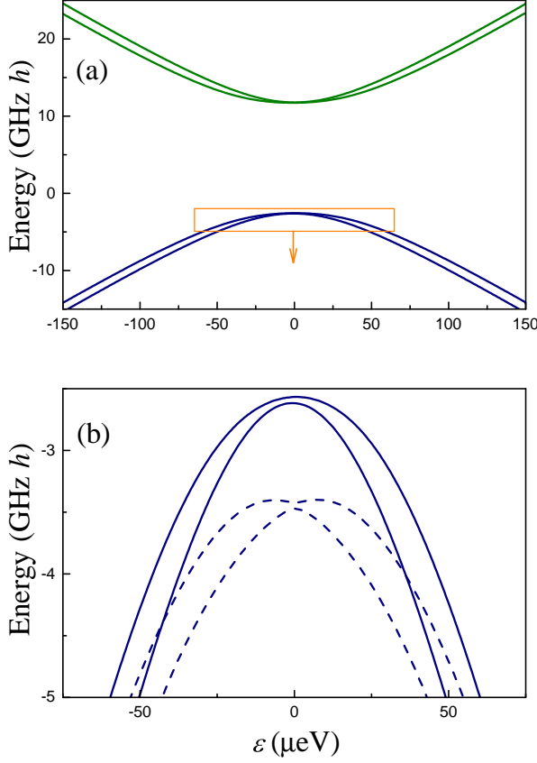
FIG. 6: Energy levels of the dressed DQD. (a) At low driving power, A_d \rightarrow 0 , these are defined by E_i \pm \hbar\omega_d/2 , see Eq. (B3). (b) Close-up of the lowest two dressed energy levels. The solid lines are the same as in (a), for low driving power. This displays the minimal energy-level distance at around \varepsilon_0 = 0 given by \Delta = (E_1 - E_0)_{\min} - \hbar\omega_d . The dashed lines show how the driving changes the dressed energy levels; these are plotted for A_d/\Delta = 2 .
