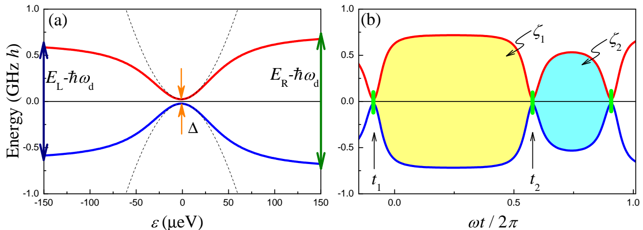
FIG. 2: Dressed energy levels. In (a) the two lowest dressed states are shown by plotting \pm\Delta\tilde{E}/2 versus \varepsilon , where \Delta\tilde{E} = \Delta E - \hbar\omega_d and \Delta E = E_1 - E_0 . The distance between the dressed energy levels shows the avoided-level crossing \Delta at around \varepsilon = 0 and tends to E_{L,R} - \hbar\omega_d to the left and right, respectively. The dashed parabolas correspond to the qubit-like spectrum at small \varepsilon . In (b) the same dressed energy levels are shown versus time for \varepsilon = \varepsilon_0 + A \sin \omega t , with \varepsilon_0 = 50 \mu\text{eV} and A = 100 \mu\text{eV} . Several avoided-level crossings take place at t = t_1, t_2 , and t_2 + 2\pi/\omega . The probabilistic LZ transitions are shown in these points by thick vertical green dashes. Between these avoided-level crossings, the wave-function phases \zeta_{1,2} are accumulated. These phases, equal to the areas under the energy-level curves, result in observable interference fringes.
