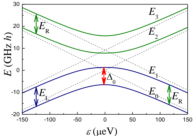
FIG. 1: A four-level system: Energy levels of an orbital-valley DQD. The four energy levels in the absence of tunneling, t_d = t_v = 0 , shown by the dashed lines, experience four crossings. In general case, shown by the solid lines, the degeneracy is lifted, and the four energy levels E_i are plotted for the parameters described in the text.
