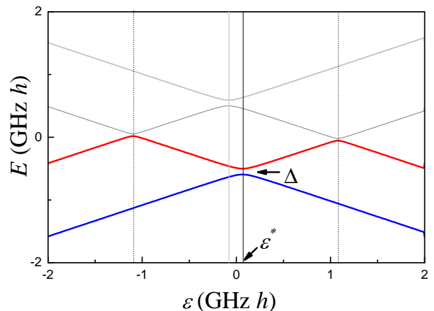
FIG. 5: Energy levels of a two-qubit system. These are shown as an example of the situation where the lower two energy levels have a small avoided level crossing \Delta and the distance between the energy levels increases at around this point and tends to constants at high values of the bias \varepsilon .
