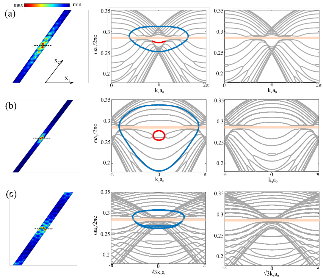
FIG. 9. Optical implementation of PT interfaces in photonic graphene with different cuts at the interfaces (indicated by black dash line): (a) zigzag, (b) bearded, and (c) armchair shaped boundaries. Left panels: Normal electric field |E| profiles for the edge modes localized at different cuts of interfaces between photonic crystals with gain and loss. Middle panels: dispersion (the real part of frequency) for PT-symmetric domain walls. Right panels: dispersion for non-PT domain walls. Branches of PT edge states located at locally parity-symmetric and parity-broken interface are shown in blue and red, respectively, and bands of dissipative bulk modes in grey. Bandgap is indicated by pink shaded region. The crystals are made of dielectric rods of radius r_a = r_b = 0.15a_0 with permittivity \epsilon_1 = 14 and gain/loss parameter \Delta = 5 embedded in air.
