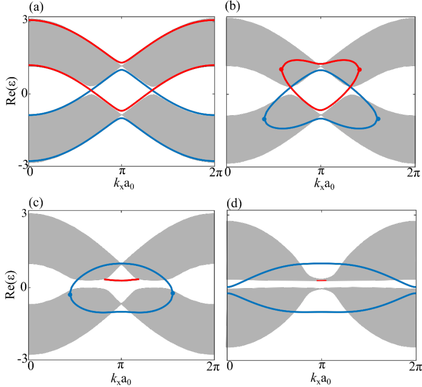
FIG. 2. Energy spectra (grey color) calculated from the TBM and edge states found analytically for locally P-symmetric (blue) and locally P-broken (red) zigzag domain walls. The parameters are (a) m_r = 0.3, m_i = 0.05 . (b) m_r = 0.3; m_i = 0.3 . (c) m_r = 0.3, m_i = 1.2 . (d) m_r = 0.3, m_i = 3 . Number of cells for each domain is N = 50 .
