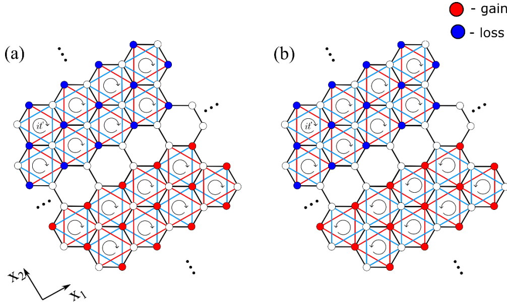
FIG. 7. Schematics of non-Hermitian Haldane model without (a) and with (b) the PT-symmetric interface.
