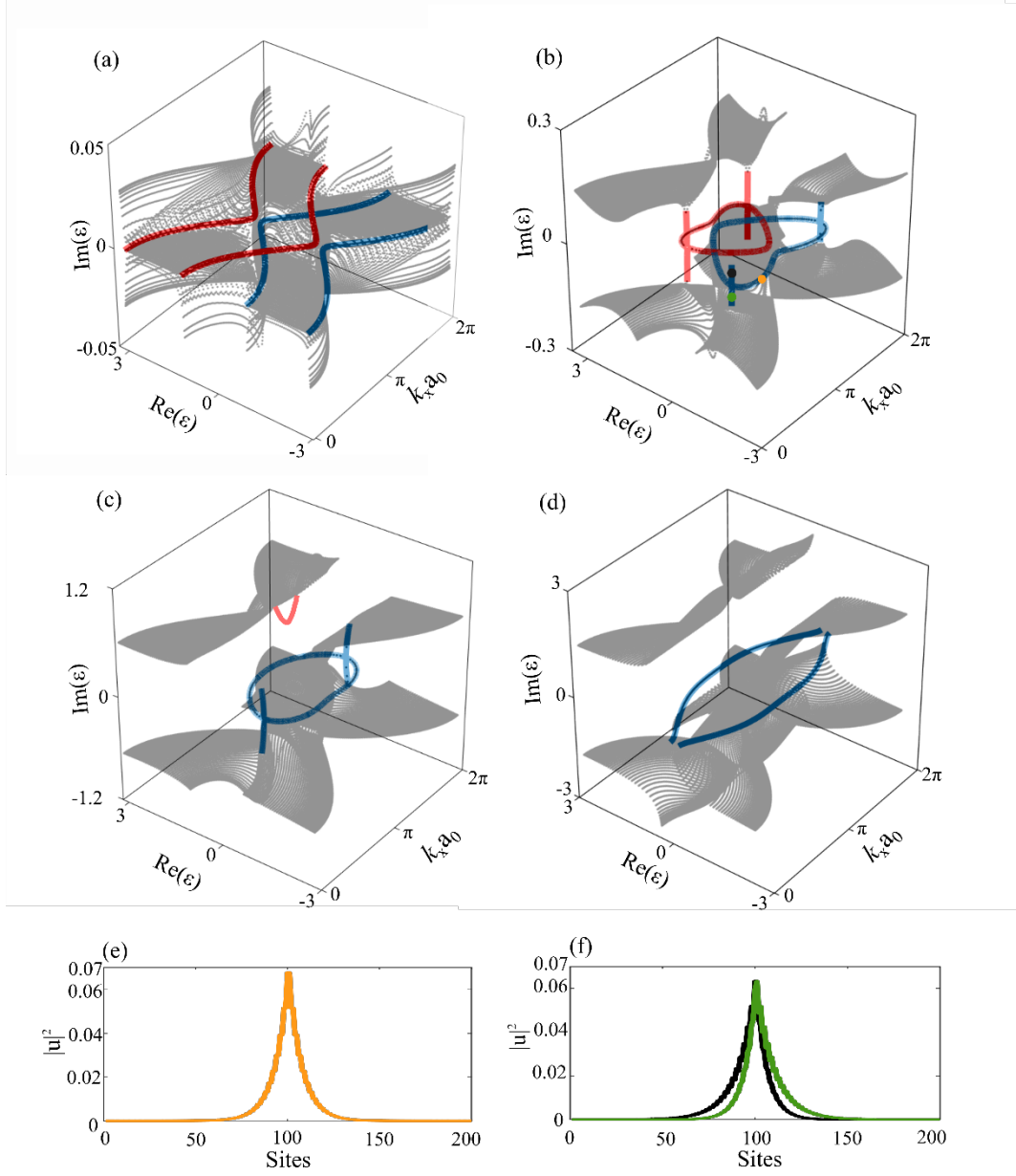
FIG. 3. Complex band structure of the same cases in (a-d) as ones in Fig.2. The wavefunction profiles of (e) PT edge states indicated by orange dot in Fig. 3(b) and complex-valued edge states with complex conjugated pairs indicated by black and green dots in Fig. 3(b) are schemed.
