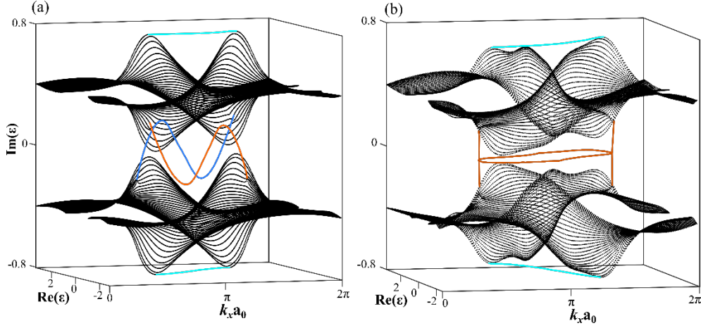
FIG. 8. Complex band structures with m_i = 0.8 , t' = 0.2 , (a) \phi = \frac{\pi}{3} for both domains (b) \phi = \frac{\pi}{3} in the domain I and \phi = -\frac{\pi}{3} in domain II. The cyan curves show the topological edge states located at the ends of the strip, and the red and blue bands in (a) are topological edge states at the domain wall, while the red loop bands in (b) are the topological PT edge states following from topological bulk invariance. Number of unit cells for each domain is N = 60 .
