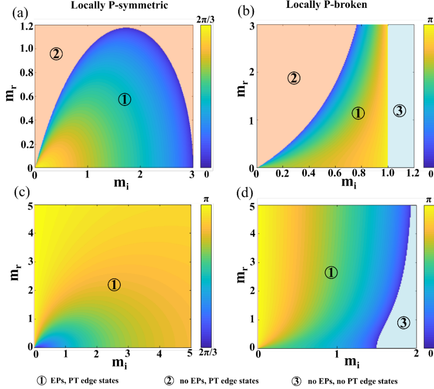
FIG. 6. Variation of the EPs’ position in the Brillouin zone obtained from Eqs. 21,22 depending on m_i and m_r for (a) zigzag cut and locally P-symmetric domain wall, (b) zigzag cut and locally P-broken domain wall, (c) bearded cut and locally P-symmetric and (d) bearded cut and locally P-broken domain wall. EPs don’t exist in light red and blue shaded regions, PT edge states are present in the light red region, but not in the light blue region.
