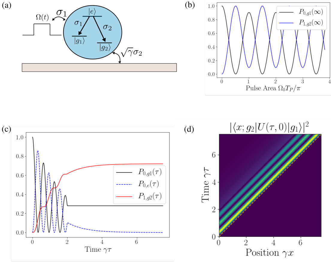
FIG. 5. Emission from a coherently driven three-level lambda system. (a) Schematic of the system being analyzed. (b) Probability of emission of a single photon P_{1,g_2}(\infty) and of no emission P_{0,g_1}(\infty) from the lambda system driven by a short pulse ( \gamma T_P = 0.2 ) as a function of the pulse area. (c) Time dependence of the probabilities P_{0,g_1} , P_{1,g_2} and P_{0,e} for a three-level lambda system driven by a long pulse ( \gamma T_P = 2 and \Omega_0 = 5\gamma ). (d) Space-time dependence of the propagator matrix elements corresponding to a single photon in the waveguide (dotted line is the light line x = \tau ). \delta_{12} = 0 and \delta_e = 0 are assumed in all the simulations.
