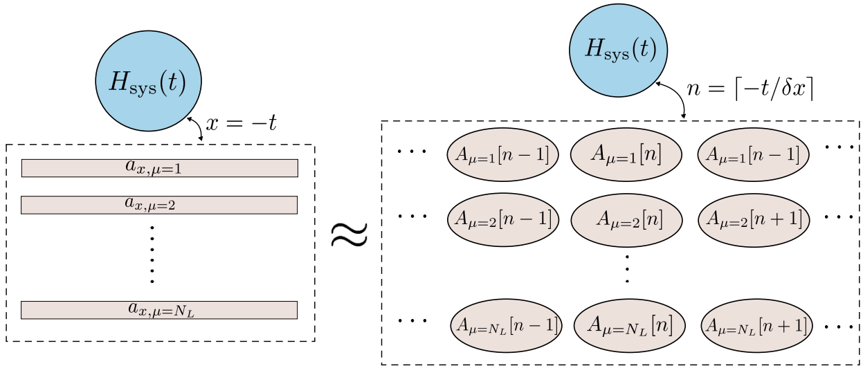
FIG. 2. Diagrammatic representation of approximating the Hilbert space of the bath modes with a discrete Hilbert space. To compute the Green's functions involving operators of the low-dimensional of the system, the spatial discretization is eventually taken in the continuum limit.
