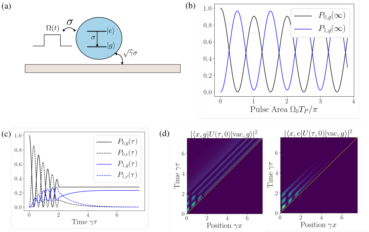
FIG. 3. Emission from a coherently driven two-level system. (a) Schematic of a two-level system driven with a pulse \Omega(t) . (b) Probability of emission of a single photon P_{0,g}(\infty) and of no emission P_{1,g}(\infty) from a two-level system driven by a short pulse ( \gamma T_P = 0.2 ) as a function of the pulse area. (c) Time dependence of the probabilities P_{0,g} , P_{1,g} , P_{0,e} and P_{1,e} for a two-level system driven by a long pulse ( \gamma T_P = 2 and \Omega_0 = 5\gamma ). (d) Space-time dependence of the propagator matrix elements corresponding to a single photon in the waveguide (dotted line is the light line x = \tau ).
