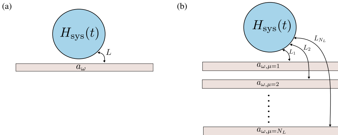
FIG. 1. Schematic of the quantum systems being considered, with a low-dimensional system coupled to (a) a single waveguide (b) multiple waveguides.
