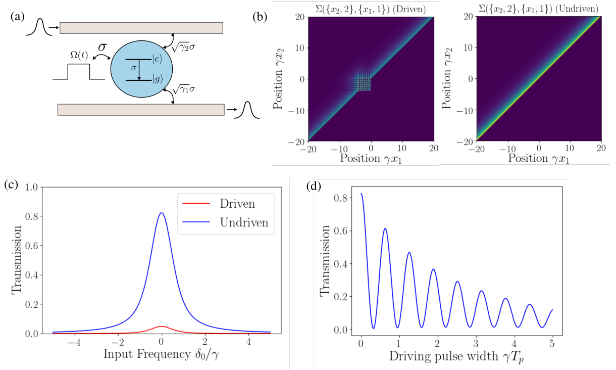
FIG. 4. Scattering of a single-photon wave-packet from a coherently driven two-level system. (a) Schematic of a coherently driven two-level system coupled to an input and output waveguide. (b) Single-photon scattering matrix for the driven and undriven two-level system. (c) Variation of the transmission of the coherently driven two-level system with the central frequency \delta_0 of the input single-photon state. (d) Variation of the transmission of a coherently driven two-level system with the length of the coherent drive for a resonant input single photon state ( \delta = 0 ). For (b) and (c), it is assumed that \gamma T_p = 4 and \Omega_0 = 5\gamma . \gamma_1 = \gamma_2 = \gamma/2 and \Delta x = 2.0/\gamma is assumed in all the calculations.
