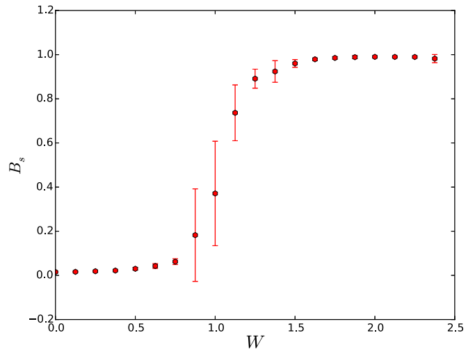
FIG. 4. The spin Bott index as a function of disorder strength W in the disorder Kane-Mele model. The parameters are t = 1 , \lambda_v = 1.65t , \lambda_{SO} = 0.3t and \lambda_R = 0.3t . 38 For each W , 10 samples with 1600 atoms are used to calculate the spin Bott index. A disorder-induced topological phase transition occurs around W = 1.0t . This is consistent with the conductance calculation in previous work. 38
