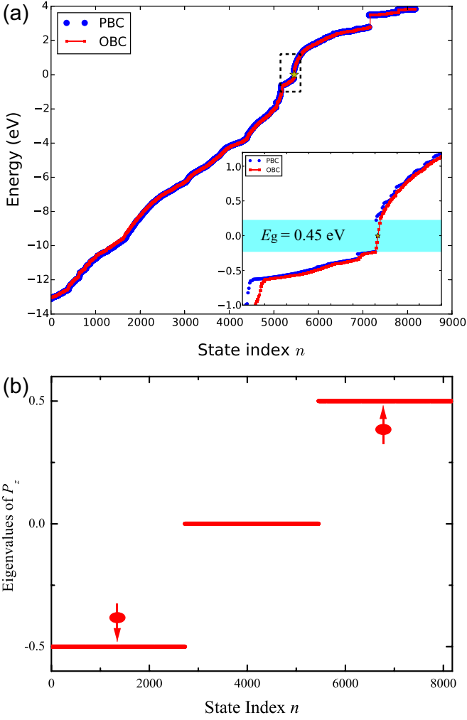
FIG. 6. Calculation of a QL with 1364 atoms. The parameters used here are \epsilon_s = 1.8 , \epsilon_p = -6.5 , \lambda = 0.8 , V_{ss\sigma} = -0.4 , V_{sp\sigma} = 0.9 , V_{pp\sigma} = 1.8 and V_{pp\pi} = 0.05 eV. (a) Energy eigenvalues E_n versus the state index n . The inset shows the spectrum around the Fermi level. The system with periodic boundary condition (PBC) shows a gap of E_g = 0.45 eV, while the one with open boundary condition (OBC) shows mid-gap states. (b) Eigenvalues of Ps_zP (in units of \hbar ) versus state index for the QL.
