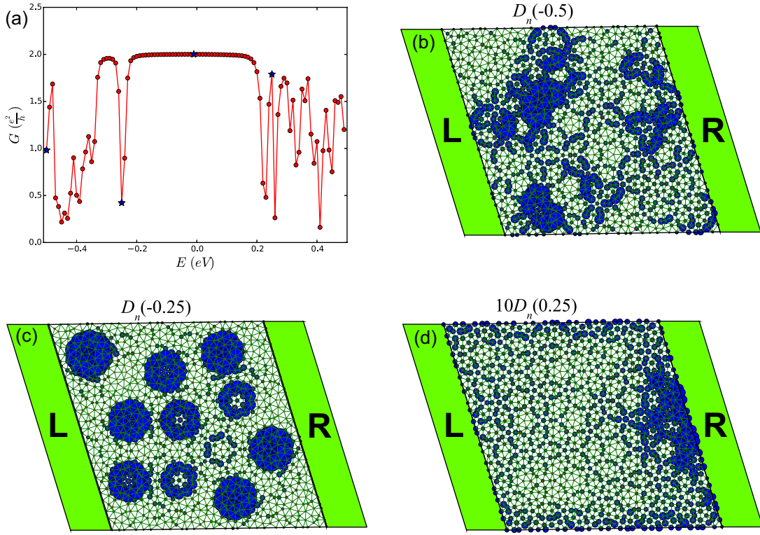
FIG. 12. (a) Two-terminal conductance G as a function of the Fermi energy E of quasicrystal in the QSH insulator phase. The conductance G shows a quantized plateau in the energy gap of QSH insulator shown in Fig.2(a) of the main text. (b) Local density of state D_n(E) at E = -0.5, -0.25 and 0.25 eV [marked as stars in (a)] for the central quasicrystal in the transport simulation. The size of blue dot represents the relative value of local density of state. For a better visualization, the local density of states in (d) is rescaled as 10 \times D_n(0.25) .
