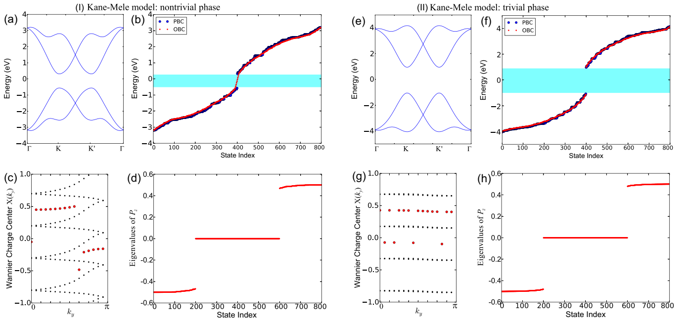
FIG. 2. Calculation of Kane-Mele model. The left panel (I) Kane-Mele model with a nontrivial QSH phase. The parameters are t = 1 , \lambda_{SO} = 0.3 , \lambda_R = 0.25 and \lambda_v = 1.0 . The right panel (II) Kane-Mele model with a trivial QSH phase. The parameters are t = 1 , \lambda_{SO} = 0.3 , \lambda_R = 0.25 and \lambda_v = 2.5 . In each panel we show (a,e) the band structure of unit cell; (b,f) energy eigenvalues versus state index of supercell sample with periodic boundary condition or open boundary condition; (c,g) evolution of the Wannier charge center X(k_y) along 0 \leq k_y \leq \pi (Red points mark the midpoint of the largest gap); (d,h) eigenvalues of P_{s_z}P (in units of \hbar ) versus state index.
