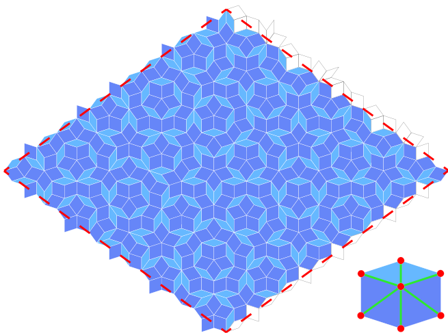
FIG. 5. Penrose tiling containing 521 vertices. The red dashed line defines a unit cell under periodic approximation. The inset shows the atomic orbitals placed on vertices of rhombuses and the first three NN hopping between them.
