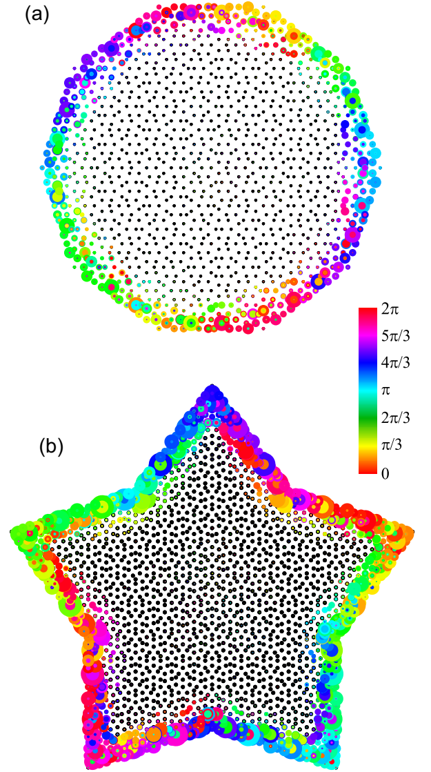
FIG. 7. Topological edge states on (a) decagon-shape and (b) pentagon-shape QLs with 1211 and 1961 atoms, respectively. The computational parameters are the same as those in Fig. 6. The size and the color of the blob indicate the norm |\rho(\mathbf{r})|^2 and phase \phi(\mathbf{r}) of the wavefunction |\psi(\mathbf{r})\rangle = \rho(\mathbf{r})e^{i\phi(\mathbf{r})} , respectively.
