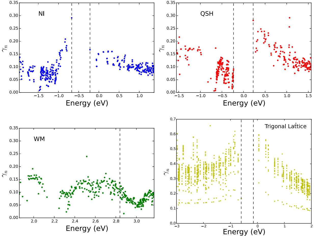
FIG. 10. Participation ratio \gamma_n of QLs at (a) normal insulator ( d_0 = 0.86 ), (b) QSH insulator ( d_0 = 0.95 ) and (c) weak metal phases ( d_0 = 1.34 ). (d) Participation ratio \gamma_n of a periodic trigonal lattice.
