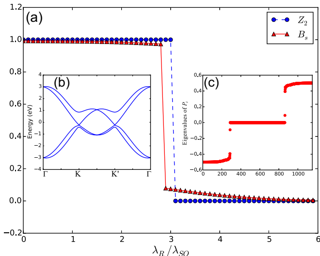
FIG. 3. Topological phase transition in the Kane-Mele model. The parameters are t = 1 , \lambda_v = 0.1t , \lambda_{SO} = 0.06t . 1 (a) The \mathbb{Z}_2 invariant and spin Bott index B_s versus \lambda_R/\lambda_{SO} . The inset shows the (b) band structure and (c) eigenvalues of P_z (in units of \hbar ) upon phase transition with \lambda_R/\lambda_{SO} = 3 , where both the band gap of the Hamiltonian and the spectral gap of P_z almost vanish.
