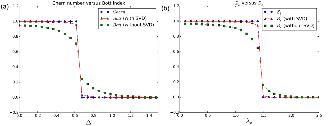
FIG. 1. (a) Topological phase transition in the Haldane model. The parameters are t = -1 and t_2 = 0.15e^{-i\pi/3} . (b) Topological phase transition in the Kane-Mele model. The parameters are t = 1 , \lambda_{SO} = 0.3 and \lambda_R = 0.25 . The Bott B (spin Bott B_s ) index is consistent with the Chern number ( \mathbb{Z}_2 invariant) except around the phase transition point. This is because we use a relatively small supercell to calculate the Bott index. The small divergence would disappear if a larger supercell is used in the calculation of (spin) Bott index. The calculated (spin) Bott index with SVD shows a better performance than the one without SVD.
