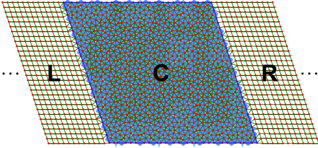
FIG. 11. Schematic illustration of transport simulation setup using the NEGF method. The central part is a finite QL, the left and right parts are two semi-infinite electric leads.
