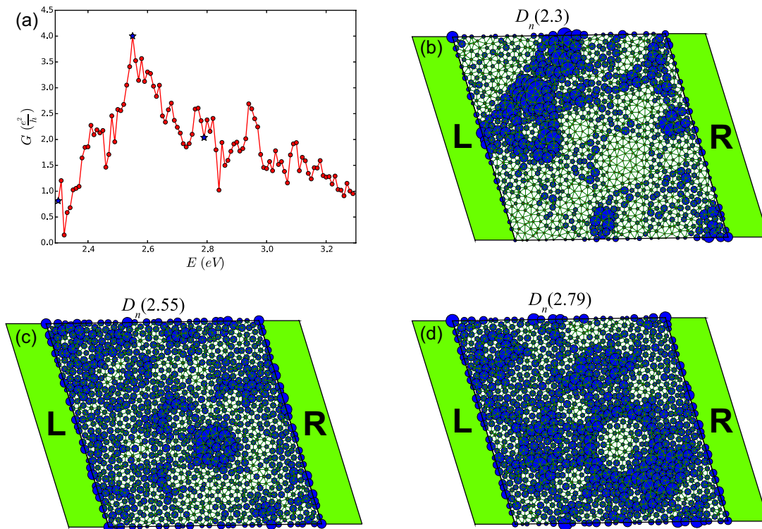
FIG. 14. (a) Two-terminal conductance G as a function of the Fermi energy E of quasicrystal in the weak metal phase. The conductance G is much smaller than that of periodic crystal with the same structure of the leads. (b) Local density of state D_n(E) at E = 2.3, 2.55 and 2.79 eV [marked as stars in (a)] for the central quasicrystal in the transport simulation. The size of blue dot represents the relative value of local density of state.
