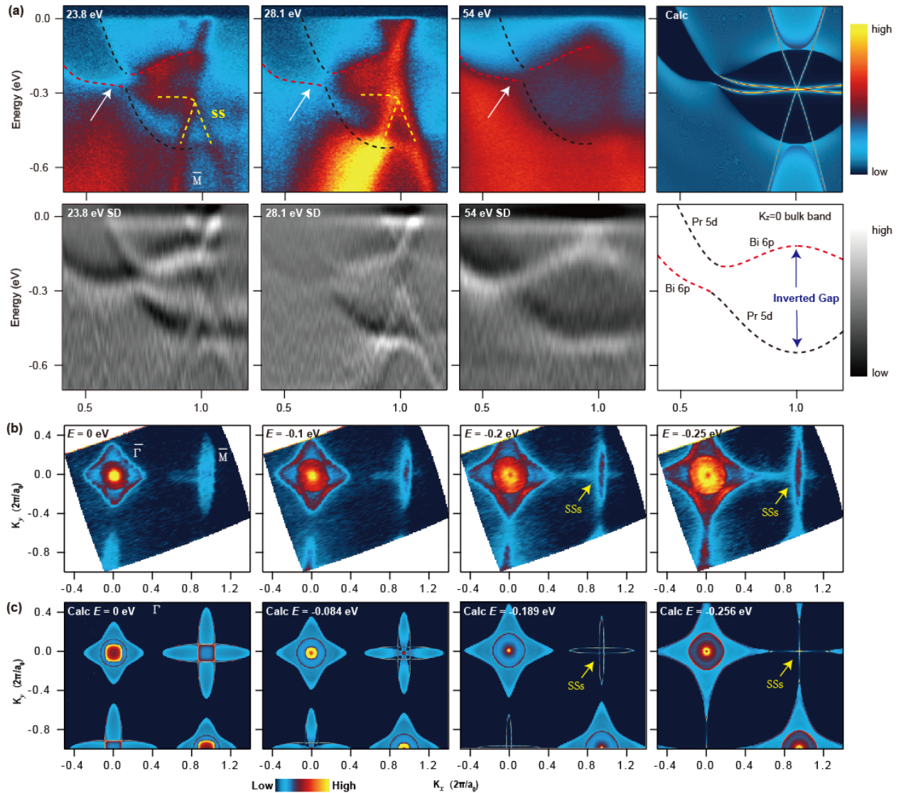
Fig. 3 (Color online). Identifying bulk band inversion and associated SSs, using PrBi data as an example. (a) Upper row: APRES data along \overline{\Gamma M} direction taken with different photon energies, compared with the calculation (the rightmost panel). The yellow, black and red dashed curves indicate extracted SSs, bulk band edge of Pr 5d and Bi 6p, respectively. The white arrows indicate the bulk band inversion point. In the calculation, the blue background indicates the bulk continuum and the SSs are shown as sharp lines lying within the inverted gap. Lower row: the corresponding second derivative of experimental data, together with the plot of bulk band character for k_z=0 cut (the rightmost panel), which is directly relevant for bulk band inversion. (b) Experimental constant energy contours using 23.8 eV photons at E=0 , -0.18 , -0.24 and -0.315 eV, which corresponds to the Fermi energy, the conduction band bottom, the bulk band inversion point and the center point of SSs. (c) Theoretical constant energy contours, to be compared with (b). Thin lines at E=-0.189 and -0.256 eV maps corresponds to SS contours centered at the \overline{M} point. All calculations were performed using the MBJ GF method.
