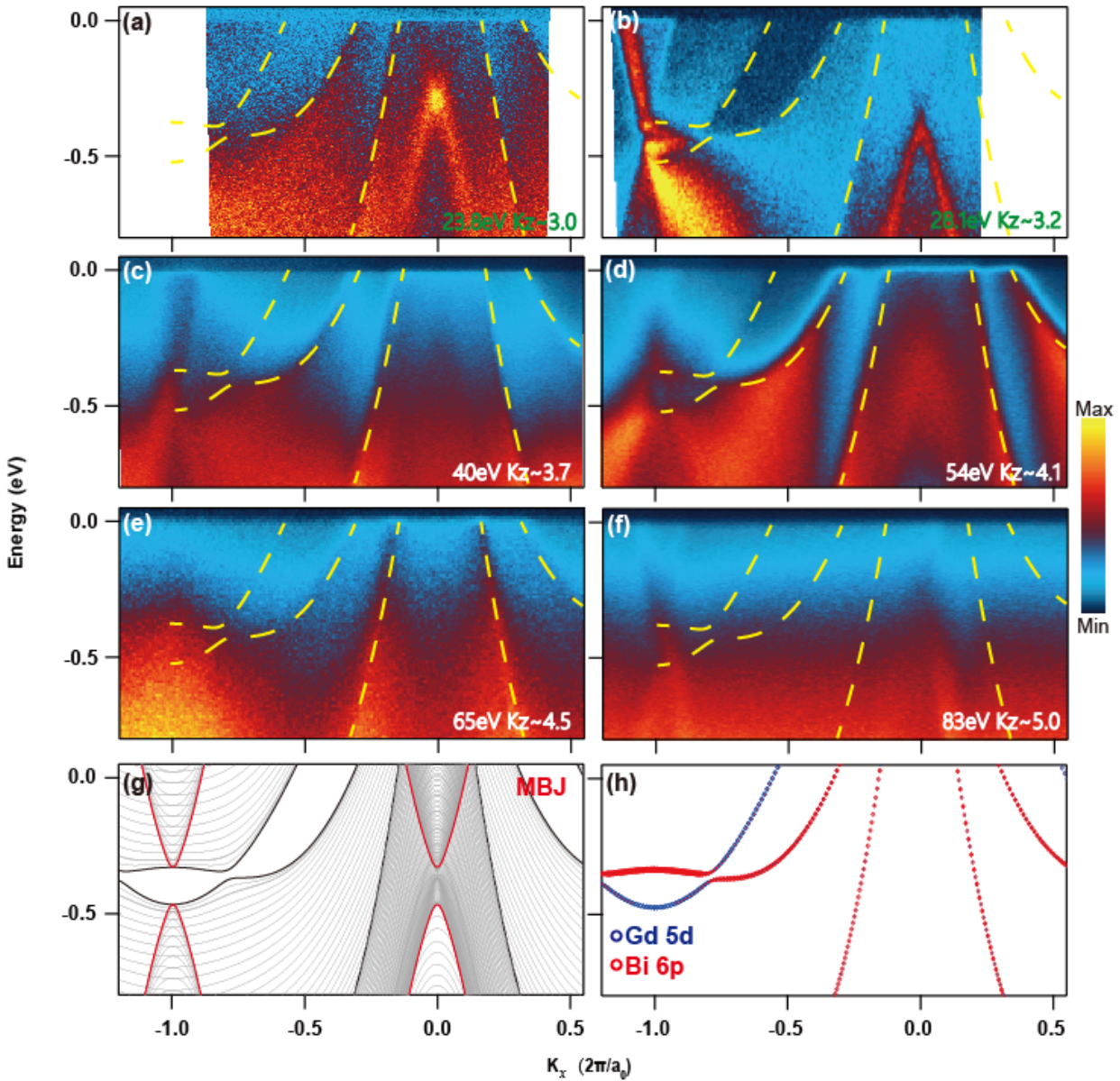
Fig. 2 (Color online). Probing the three-dimensional band structure by photon-energy dependent ARPES, example of GdBi. (a-f) ARPES spectra of GdBi taken along \overline{\Gamma M} direction with various photon energies, in comparison with the projected bulk band calculation using the MBJ potential (g). The k_z values, indicated at the bottom right of the experimental data, are calculated based on the dipole transition model using an estimated inner potential of 14 eV. The dashed yellow curves on top of experimental data are the extracted dispersion relations of the bulk bands at k_z=0 cut. The fact that they do not show continuous change with photon energy indicates large k_z broadening in the photoemission process, which yields emission features dominated by the band edge ( k_z=0 or \pi cuts). The thick black (red) curves in (g) indicates k_z=0 ( k_z=\pi ) cuts. (h) The band character for the k_z=0 cut, highlighting the bulk band inversion between Gd 5d and Bi 6p bands near \overline{M} point.
