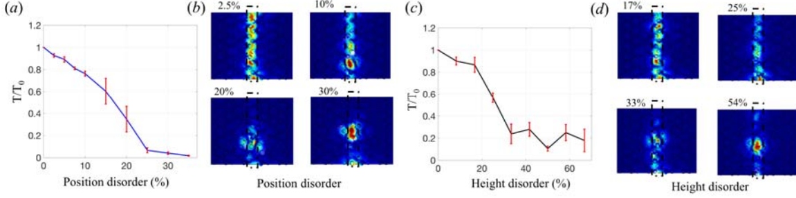
Figure 14: (a) the relation between position disorder degree and T/T_0 at \Omega a = 13.30 ; (b) propagating states abs(u_z) at four position disorders; (c) the relation between height disorder degree and T/T_0 at \Omega a = 13.30 ; (d) propagating states abs(u_z) at four height disorders. The red vertical bars in (a) & (c) stand for the root mean square of fluctuations. Only the phononic crystal part of the whole geometry in Fig.8a is shown in (b) & (c).
