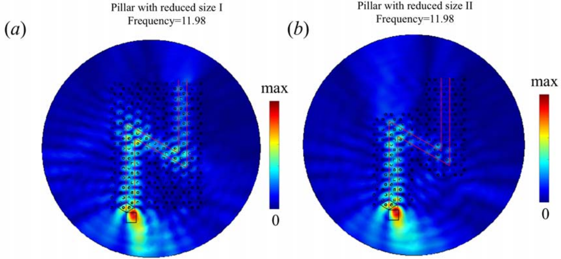
Figure 7: Minimized bulk size with one hexagon unit on one side of the straight interface part (a) or on any side of the zig-zag interface (b). Flexural wave source is excited at \Omega a = 11.98 .
