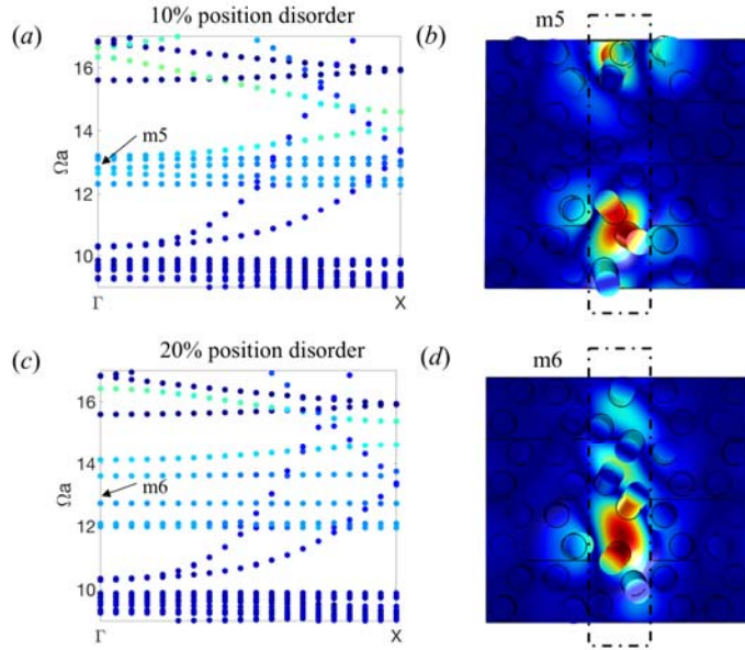
Figure 15: (a) GX dispersion when 10% position disorder is applied to pillars in the dotted rectangle as Fig.11c; (b) eigenmode abs(u_z) of m5 at \Gamma point; (c) GX dispersion when 20% position disorder; (d) eigenmode abs(u_z) of m6 at \Gamma point.
