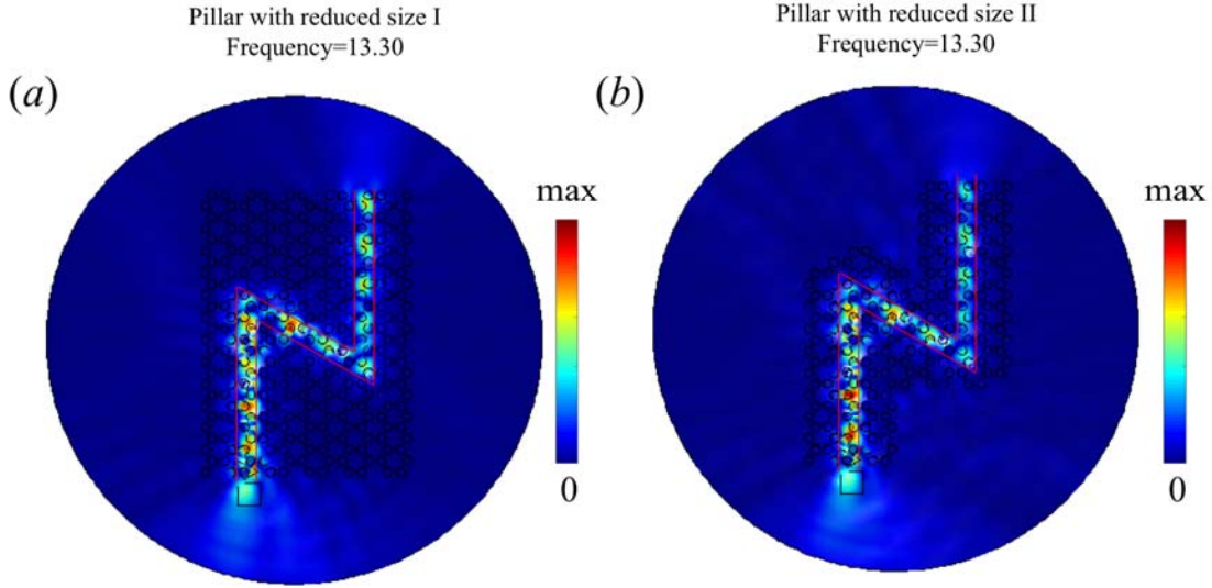
Figure 13: minimized bulk size with one hexagon unit on one side of the straight interface part (a) or on any side of the zig-zag interface (b). Flexural wave source is excited at \Omega a = 13.30 .
