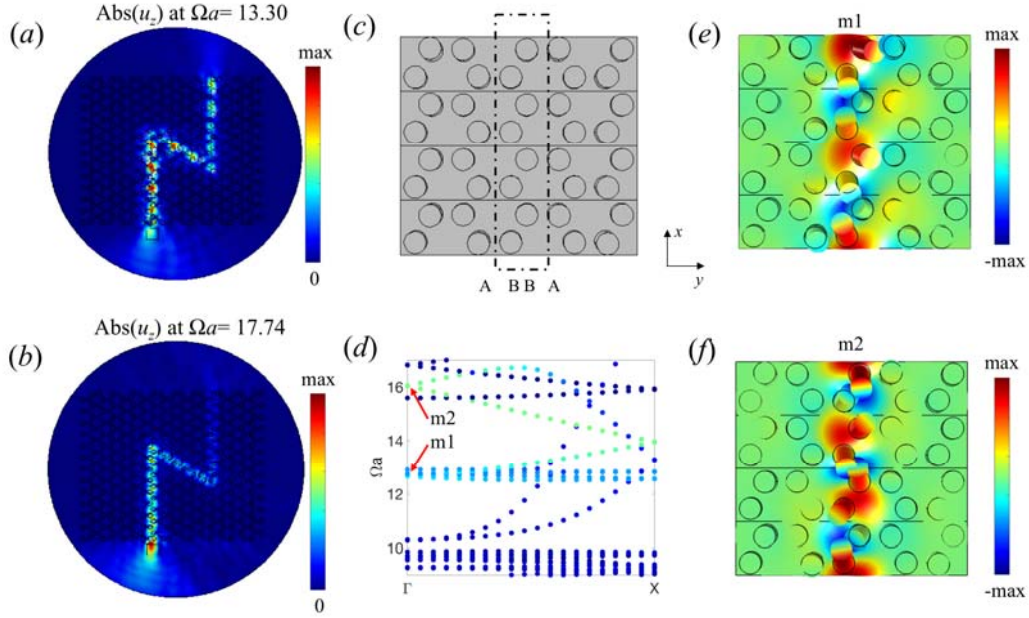
Figure 11: Conventional interface states at \Omega a = 13.30 (a) and \Omega a = 17.74 (b); (c) Geometry of a super-cell model with two lattices as A-B-B-A type interface (dotted rectangle) in the middle to better understand the conventional interface mode. The model has a size of 4a in x and 4.33a in y , with Bloch-periodic conditions applied to the edges in both directions. The dispersion along \Gamma X is calculated and shown in (d) with two points at \Gamma point as m1 and m2; The real part of u_z of eigenmodes m1 and m2 points are shown in (e) and (f), respectively.
