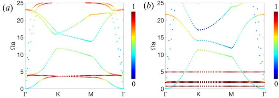
Figure 3: Dispersion of pillared (a) and sphered (b) phononic crystal plate with honeycomb lattice arrangement with asymmetric resonators A and B. Geometric parameters are lattice parameter a , thickness of the plate e=0.1a , radius of the pillar r_p=0.1a , height of the pillar h_A=1.2a and h_B=0.4a , radius of the sphere r_{sA}=0.208a and r_{sB}=0.144a . The color bar in the dispersion indicates a displacement ratio \alpha in Eq.(2).
