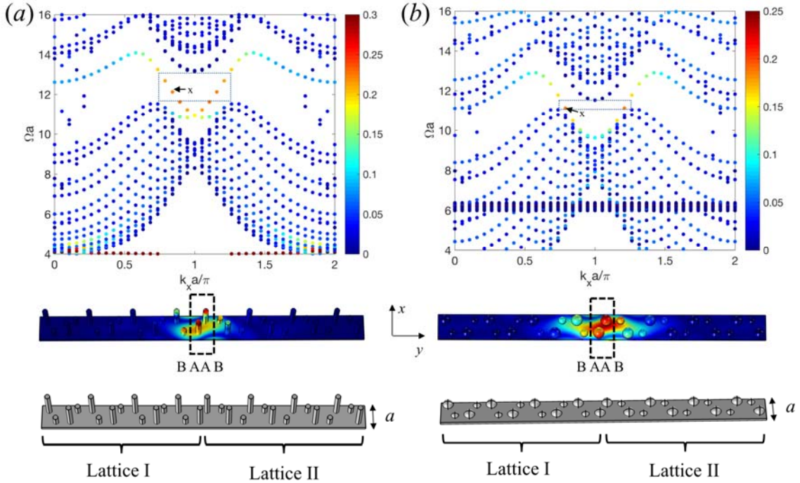
Figure 4: Dispersion of a stripe consisting of the juxtaposition of B-A (lattice I) and A-B (lattice II) honeycomb lattices with the interface as B-A-A-B for pillared (a) and spherical (b) resonators (the geometry of the two lattices stripes are shown at the bottom). The color in the dispersion represents the ratio of total displacement localized in the A-A resonators (black dotted rectangle) over the whole stripe. The total displacement distributions at marked 'x' point in the dispersion are shown below the dispersion curves. Here the wavenumber k_x a/\pi in dispersion is used as the stripe is finite in y axis but infinite in x axis, not relating to the Brillouin zone in Fig.1.
