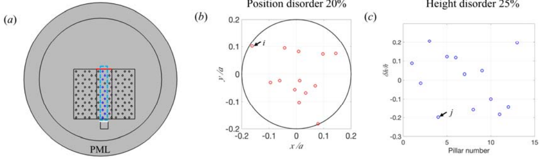
Figure 8: (a) is the geometric model used in random simulation. The A_0 Lamb mode wave is excited by the finite white line source and transmitted wave is detected by the finite red line. Example of position disorder 20% (b) and height disorder 25% (c) for all pillars in the interface (limited in the blue dotted box) in (a); The dots in (b) and (c) show one example of the random profiles.
