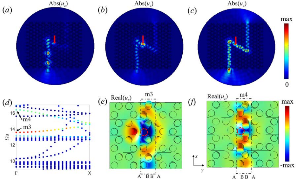
Figure 12: Abs(u_z) of conventional interface states at \Omega a = 13.30 (a), \Omega a = 13.75 (b) and \Omega a = 16.41 (c) when moving a pillar in the central of zig-zag path pointed with red arrow (the same as in the insert of Fig.6); (d) dispersion along \Gamma X when moving one pillar in the interface with the color standing for the displacement concentration rate on the two pillars in the neighborhood of the absent pillar position over the whole supercell; The Real(u_z) of eigenmode m_3 at \Omega a = 13.75 (e) and m_4 at \Omega a = 16.41 (f) at \Gamma point are shown, with the absent pillar indicated as the red dotted circle.
