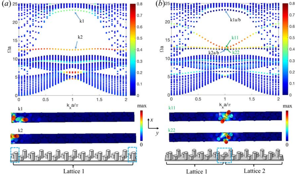
Figure 10: (a) Dispersion of a stripe consisting unit cell with one honeycomb lattice as h_A=0.8a and h_B=0.4a with the color stands for the displacement concentration rate of the four pillars (in the two dotted boxes) at the two edges in y . The amplitudes of total displacement distributions at k_1 and k_2 points shown at the bottom. (b) Dispersion of a stripe consisting unit cell with two lattices as an interface type ABBA in the middle with the color stands for the displacement concentration rate of the four pillars (in the dotted box) at middle interface. The amplitudes of total displacement distributions at k_{11} and k_{22} points (green color) shown at the bottom. Thickness of the plate e=0.1a , radius of the pillar r_p=0.2a .
