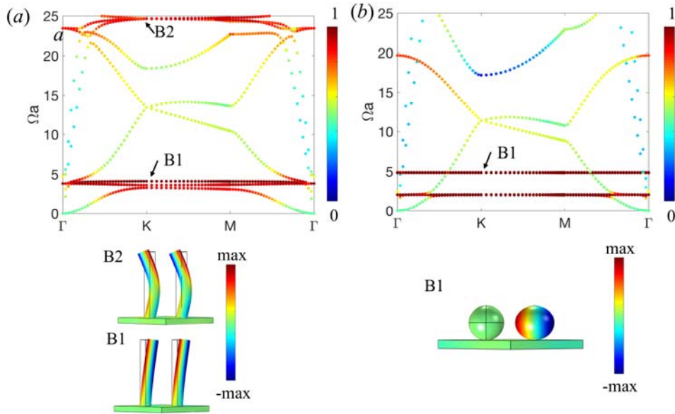
Figure 2: Dispersion of pillared (a) and sphered (b) phononic crystal plate with honeycomb lattice arrangement with identical scatters A and B. Geometric parameters are lattice parameter a , thickness of the plate e=0.1a , radius of the pillar r_p=0.1a , height of the pillar h=1.2a , radius of the sphere r_s=0.208a . The pillar and the sphere have a same
