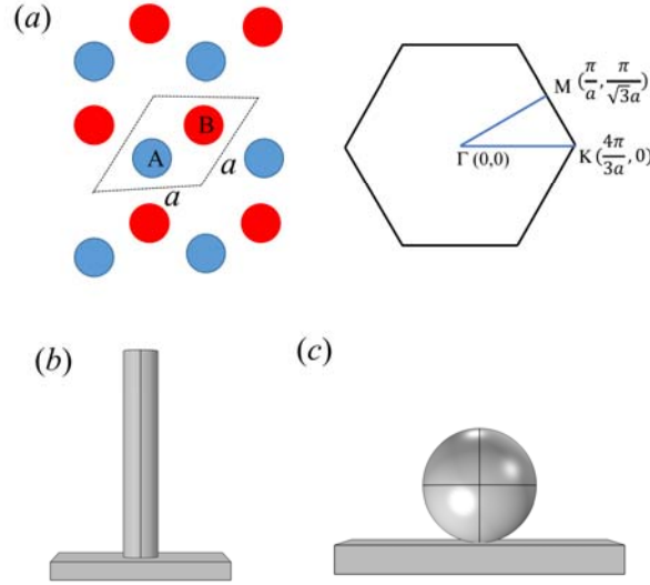
Figure 1: (a) Phononic crystal plate with honeycomb lattice and the corresponding Brillouin zone; cylinder (b) and sphere (c) resonators are deposited on a thin plate.
