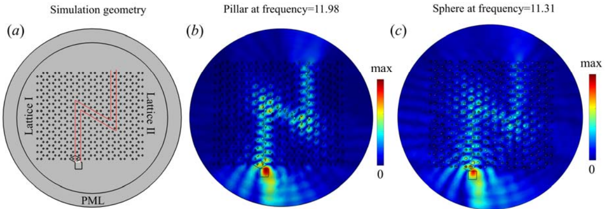
Figure 5: (a): schematic view of the numerical model: the phononic crystal plates consist of two lattices (as in Fig.4) with a zig-zag interface path (limited by the red lines); a finite antisymmetric Lamb wave source is excited along the white line segment (at the bottom exit of zig-zag path); Perfect Matched Layer (PML) is applied to surround the phononic crystal plates to avoid any wave reflection. Topologically protected edge state is excited by anti-symmetric Lamb wave at \Omega a = 11.98 for pillar-resonator (b) and at \Omega a = 11.31 for sphere-resonator (c) with backscattering-immune property. The color bars show the amplitude of the displacement u_z .
