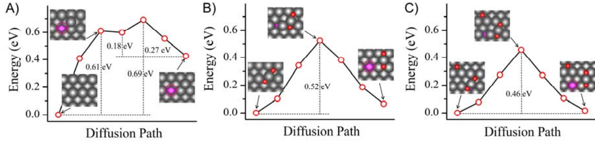
Fig. 15. Energetics of atom extraction from the Ag(110) surface: A) in the absence of O atoms, B) in presence of 0.16 ML of O adatoms, C) in presence of 0.25 ML of O adatoms. Also shown are the activation energy barriers. The grey, pink and red balls represent the Ag atoms of the top layer, the Ag atom of the third layer and the O adatoms, respectively.
