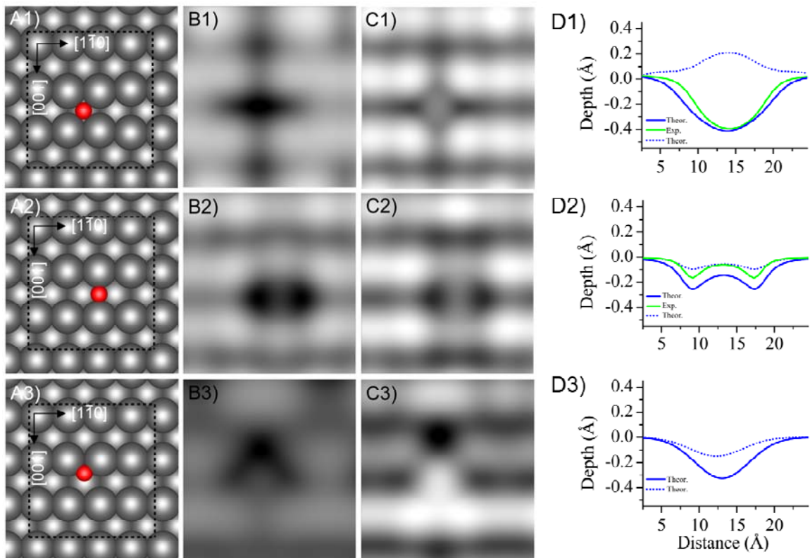
Fig. 8. (A1-A3) DFT-optimized geometries of O adatoms at A1) FFH A2) LB and A3) TFH sites; (B1-B3 and C1-C3) corresponding simulated STM images at B1-B3) V=70 \text{ mV} and C1-C2) V=700
