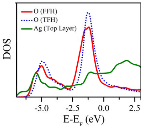
Fig. 13. Electron density of states projected on the 2s and 2p orbitals of an isolated O adatom at FFH site (red solid trace) and of an O adatom at TFH site embedded in the -O-Ag-O-Ag-O- zig-zag chain (blue dotted trace) formed on Ag(110), and the 5s orbital of Ag atoms on the topmost layer (green trace) of the bare Ag(110). The energy is expressed relative to the Fermi energy (0 eV as reference level).
