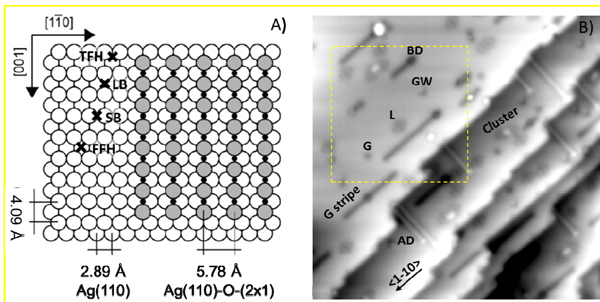
Fig. 1. A) Geometry of the Ag(110) surface. The four-fold hollow (FFH), long bridge (LB), short bridge (SB) and three-fold hollow (TFH) sites, relevant for the data presentation are marked on the left part of the drawing. The structure of the Ag(110)-O-(2x1) added row reconstruction is shown in the right part. B): STM image of the Ag(110) surface exposed to 19 L of O 2 at 175 K (image size: 25x25 nm 2 , V=0.07 V, I=1.3 nA, virgin area). Black dot (BD) decorated by grey stripes, isolated grey dot (G d ), lozenge (L), added row (AD), grey and white dot oriented along [100] (GW) and isolated cluster structures are apparent on the terraces. The dashed box indicates the area subject to the manipulation experiment reported in Fig. 4. Added rows stretch along the [001] direction while G stripes have the axis aligned along [1 0].
