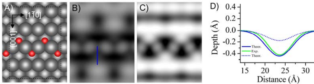
Fig. 9. A) Optimized geometry of O adatoms at TFH sites and organized in an -O-Ag-O-Ag- zig-zag chain; (B-C) Simulated STM images at V=70 mV and V=700 mV, respectively; D) Line profiles cut along the [001] direction (blue path in panel B). The blue solid and dashed traces derive from the simulated images at V=70 mV and V=700 mV, respectively. The experimental curve recorded at 70 mV is plotted in green. No experimental trace is available for V=700 mV since at this bias voltage the grey stripes are disrupted.
