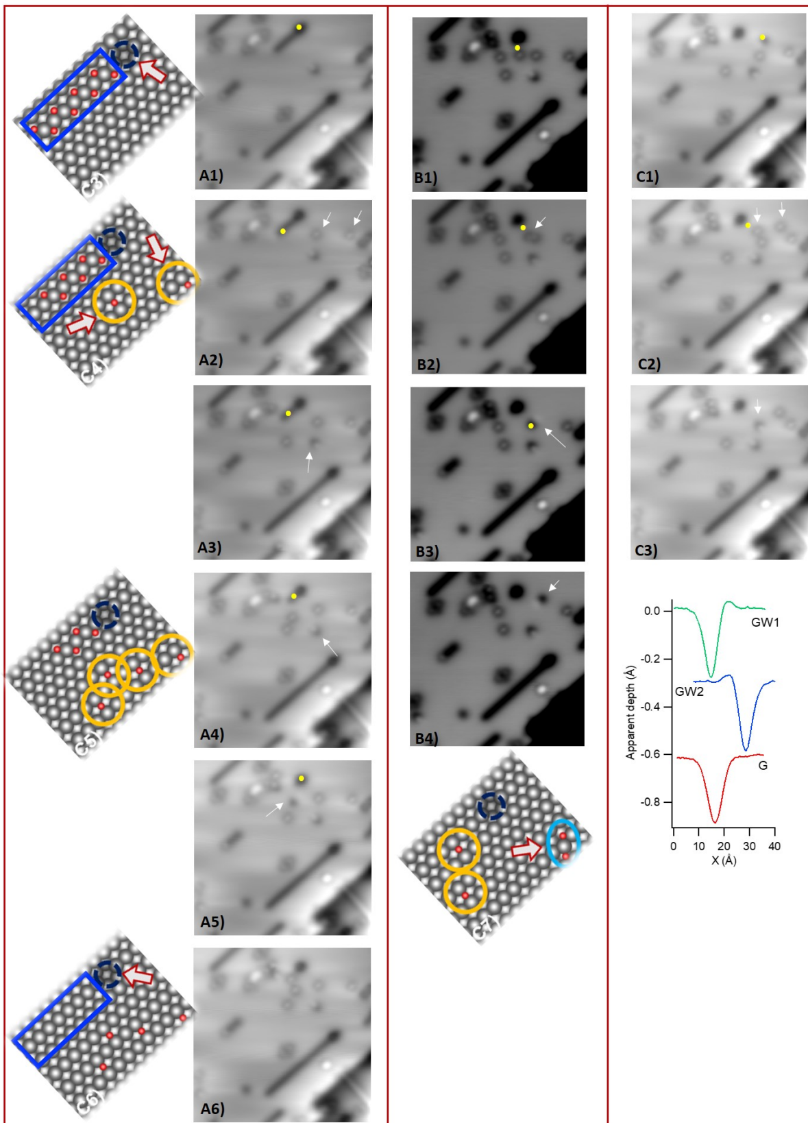
Fig. 4. STM images showing three manipulation sequences performed on different objects present in the same area. In sequence A sombreros are generated from the grey tail of a black dot by
