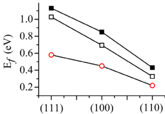
Fig.14. Calculated vacancy formation energy per surface unit cell on the (111), (100), and (110) surfaces of Ag. DFT results are shown by solid squares, effective medium theory results [52] by empty squares, and results from the inserted-atom method [53] by empty circles.
