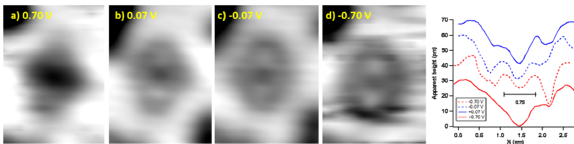
Fig. 6. STM images showing lozenges recorded at different tip bias ( I = 1.0 nA, T = 6 K, image size = 2.2 \times 3.0 nm 2 ) and corresponding line profiles cut along the [1-10] direction, i.e. along the major axis of the lozenge. The distance between the center of the lobes in this direction is 7.5 Å.
