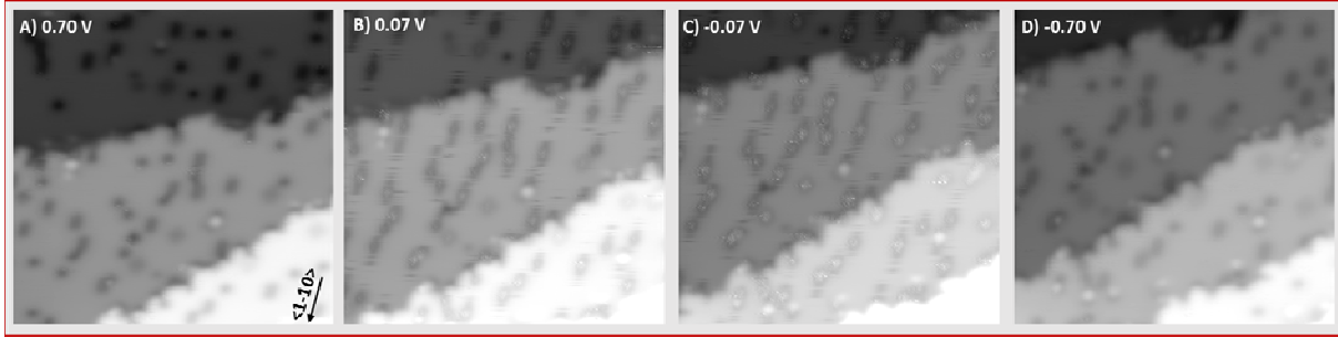
Fig. 3. Sequence of STM images of the Ag(110) surface exposed to 18 L of O_2 at 180 K recorded at different V ( I= 1.0 nA, image size: 22.5 \times 22.5 nm 2 ) and at T=77 K. At low bias voltage (panels B and C) short stripes are present in the scanning direction (horizontal) due to the movement of weakly bonded oxygen adatoms under the tip while the image is recorded. Such effect is absent in the images collected at V= \pm 0.7 V (panels A and D) since the apparent depth of sombreros is then smaller (see Fig. 8 below).
