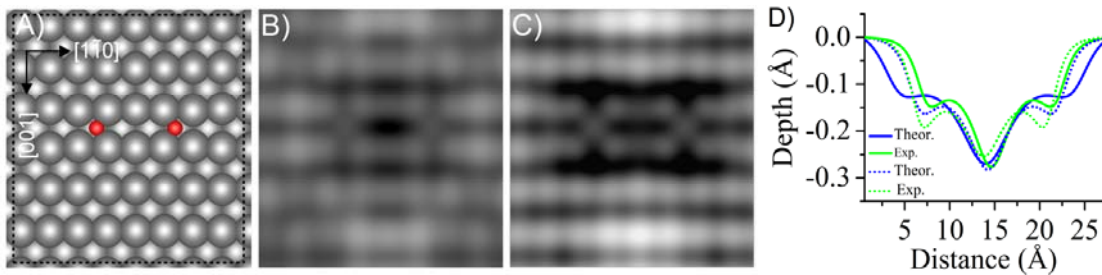
Fig. 12. A) Optimized geometry of a configuration with two O adatoms positioned in the troughs of the Ag rows, slightly off the FFH sites, forming the lozenge (L) shaped objects. (B-C) Simulated STM images at V=70\text{ mV} and V=700\text{ mV} , respectively; (D) Line profiles in the valley along [1\ 0] (solid trace for 70\text{ mV} ; dashed trace for V=700\text{ mV} ).
