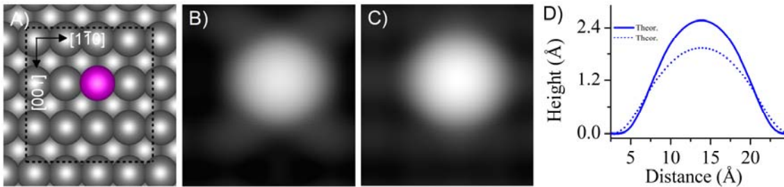
Fig. 11. A) Optimized geometry of O residing at the octahedral subsurface site. The Ag atom (pink ball) is located just on top of a subsurface O atom; (B-C) Simulated STM images at V=70 mV and V=700 mV, respectively; and (D) Line profiles (solid trace for 70 mV; dashed trace for V=700 mV).
