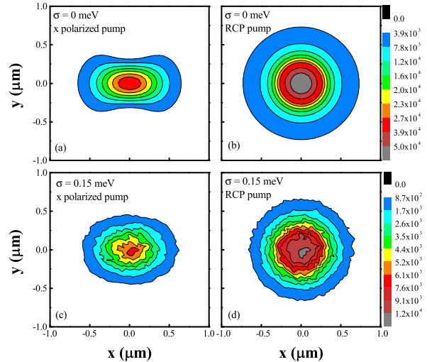
FIG. 4. Exciton transport when pumped with x polarized pump (a,c) and right circularly polarized (RCP) pump (b,d). (a,b) correspond to the case without disorder, (c,d) for the case with disorder with correlation amplitude \sigma = 0.15 meV.
