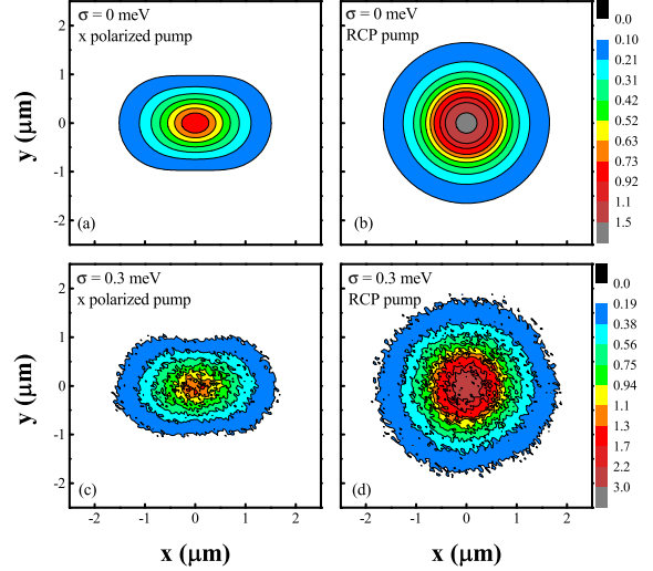
FIG. 5. EP transport when pumped with x polarized pump (a,c) and right circularly polarized (RCP) pump (b,d). (a,b) correspond to the case without disorder, (c,d) for the case with disorder with correlation amplitude \sigma = 0.3 \text{ meV} . The detuning of EPs in the calculations is \Delta = 60 \text{ meV} .
