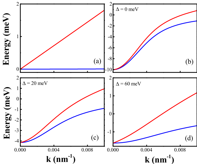
FIG. 2. The dependence of two exciton branches resulting from (1) (a) and lower two EP branches from (2) for detunings \Delta = 0 meV (b), \Delta = 20 meV (c), \Delta = 60 meV (d) on absolute value of in plane momentum |\mathbf{k}| .
