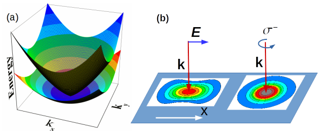
FIG. 1. (a) Schematic drawing of the band structure of excitons in TMDs and (b) depiction of exciton transport when the system is pumped with linearly polarized light (left) and right circularly polarized light (right).
