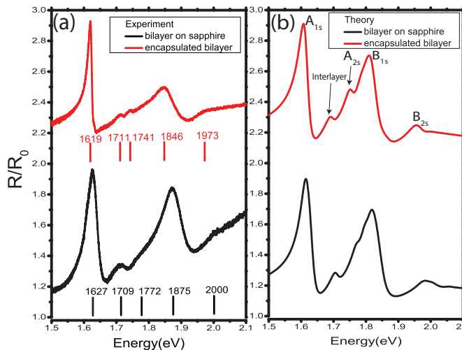
FIG. 4: (a) Comparison between optical spectra of MoSe 2 bilayer with hBN encapsulation (red curve) and without hBN encapsulation (black curve). The MoSe 2 bilayer with hBN encapsulation shows a significant linewidth narrowing in both intralayer and interlayer excitonic transitions due to symmetric dielectric screening and a clean environment. (b) Corresponding simulated optical spectra showing the theory is able to capture the dielectric screening effects on different exciton species.
