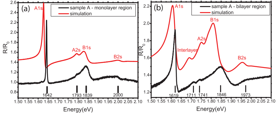
FIG. 2: Measured (black curve) and simulated (red curve) reflection contrast spectra( R/R_0(E) ) from encapsulated monolayer(in (a)) and bilayer(in(b)) region of sample A, where R(E) and R_0(E) are reflection spectrum from sample and substrate area. Comparing experiment and theory, we assign the peaks from low to high energy as A_{1s} , A_{2s} , B_{1s} , B_{2s} for the intra-layer excitons and identify the new peak at 1711 meV in the bilayer as the inter-layer A_{1s}^{\text{inter}} exciton. All simulated spectra have been shifted for better visibility.
