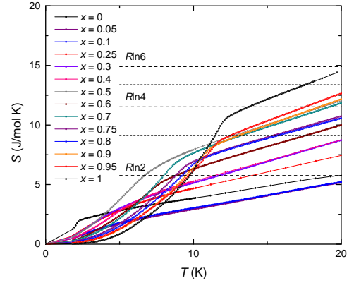
FIG. 12. (Color online) Electronic entropy, S(T) , calculated as described in the text, plotted vs. temperature, T . Dashed lines showing R \ln(2J+1) at various values of total angular momentum J are provided for comparison.
