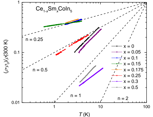
FIG. 13. (Color online) Plot of \log[(\rho - \rho_0)/\rho(300 \text{ K})] vs. \log T for \text{Ce}_{1-x}\text{Sm}_x\text{CoIn}_5 ( 0 \leq x \leq 0.5 ) up to T \approx 15 \text{ K} . Linear behavior indicates power-law behavior given by Eq. 5. Dashed lines are provided at exponents of n = 0.5, 1, and 2 as guides to the eye.
