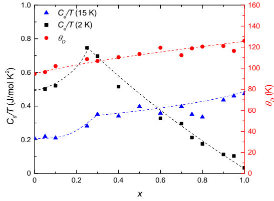
FIG. 11. (Color online) Electronic contribution to the specific heat divided by temperature, C_e/T , at 2 K (black squares), temperature-independent contribution to C_e/T at 15 K, above the magnetic ordering temperature (blue triangles), and Debye temperature \Theta_D (red circles), all plotted as a function of Sm concentration x , in \text{Ce}_{1-x}\text{Sm}_x\text{CoIn}_5 . Dashed curves are guides to the eye. The procedures for determining the values of C_e/T at 2 K and 15 K are described in the text.
