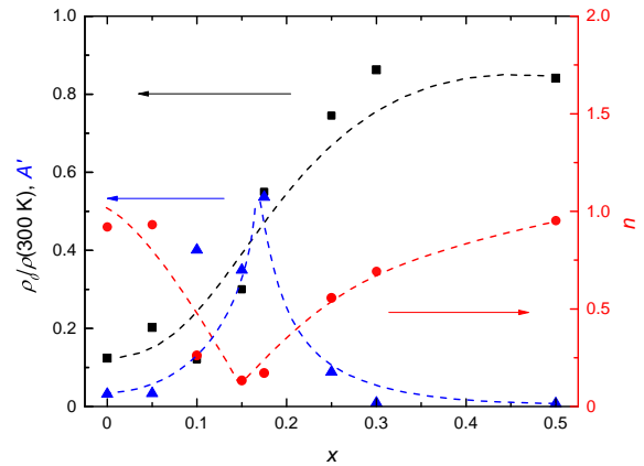
FIG. 14. (Color online) Normalized residual resistivity \rho_0/\rho(300 \text{ K}) (black), normalized coefficient A' (blue), and exponent n (red) vs. Sm concentration x for \text{Ce}_{1-x}\text{Sm}_x\text{CoIn}_5 . The values of \rho_0/\rho(300 \text{ K}) , A' , and n were extracted from fits of Eq. 5 to the \rho(x, T) data in Fig. 13.
