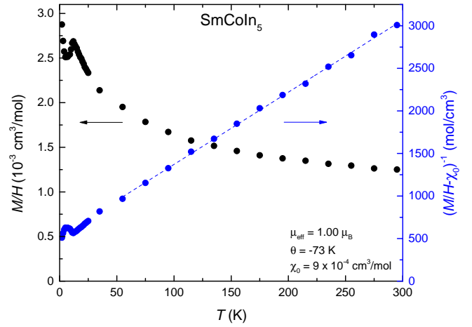
FIG. 6. (Color online) Magnetization, M/H , and (M/H - \chi_0)^{-1} , where \chi_0 is a constant, vs. temperature, T , for \text{SmCoIn}_5 . Best-fit values for the effective magnetic moment, \mu_{eff} , Curie-Weiss temperature, \theta , and \chi_0 were extracted from a fit of the Curie-Weiss law to the data and are given in the panel. Features corresponding to magnetic transitions are observed at low temperatures.
