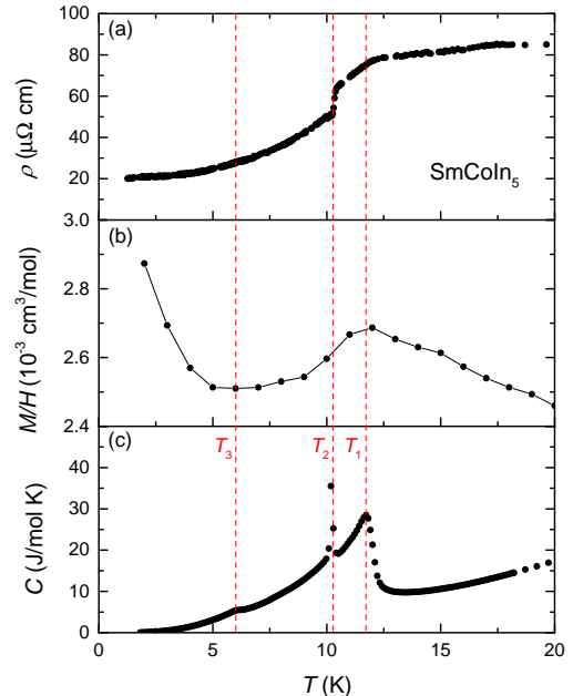
FIG. 8. (Color online) (a) Electrical resistivity, \rho , (b) magnetization divided by magnetic field, M/H , and (c) specific heat, C , vs. temperature, T , in the range 0 \leq T \leq 20 K. Corresponding magnetic transitions can be observed in the different measurements with the vertical red dashed lines drawn through T_1 , T_2 , and T_3 which serve as guides to the eye.
