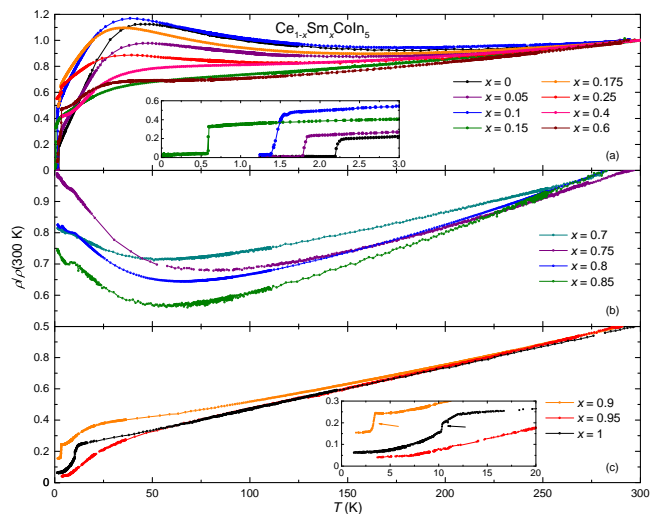
FIG. 3. (Color online) Electrical resistivity, \rho , normalized by its value at 300 K, plotted vs. temperature, T , for \text{Ce}_{1-x}\text{Sm}_x\text{CoIn}_5 . (a) Samples with low Sm concentration display both a coherence peak associated with the formation of a coherent Kondo lattice and superconductivity (see inset) that is suppressed with increasing x . (b) As x increases above 0.6, we observe a crossover into a single-ion-like Kondo effect in which Ce ions behave as a magnetic impurity in \text{SmCoIn}_5 . (c) On the Sm-rich side of the phase diagram, the only salient feature observed is a sharp, “knee-like” feature consistent with AFM order of the Sm sublattice, as observed previously (see inset). 12
