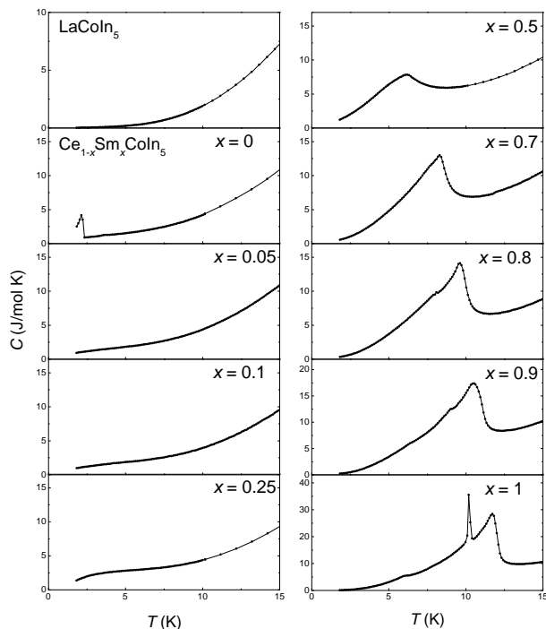
FIG. 9. Specific heat, C , plotted vs. temperature, T , for \text{LaCoIn}_5 and \text{Ce}_{1-x}\text{Sm}_x\text{CoIn}_5 ( x = 0, 0.05, 0.25, 0.5, 0.7, 0.8, 0.9 , and 1 ) to demonstrate the evolution of behavior; we move from superconductivity on the Ce-rich side to antiferromagnetic order on the Sm-rich side.
