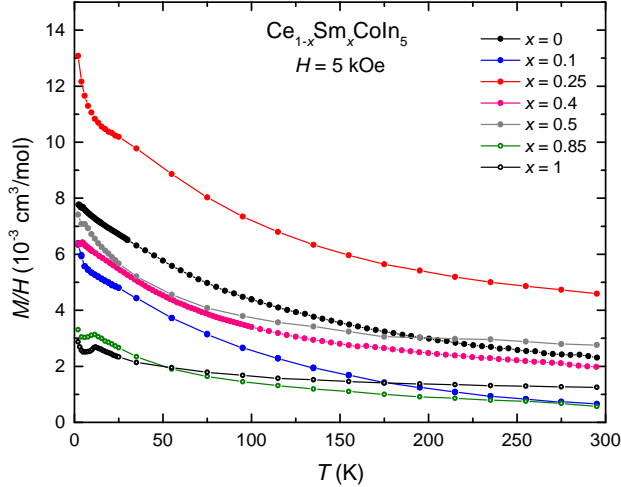
FIG. 5. (Color online) Magnetization, M/H , vs. temperature, T , measured in an applied magnetic field H = 5 kOe. The magnetic field was oriented parallel to the ab -plane.
