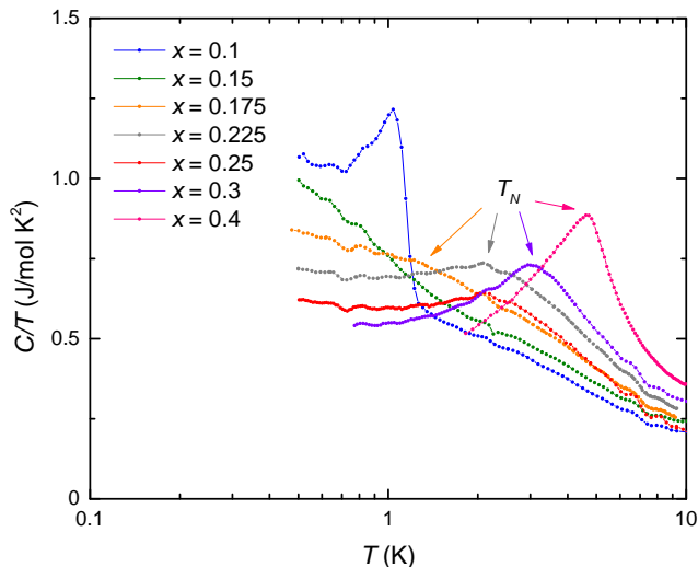
FIG. 10. (Color online) Specific heat, C , divided by temperature, T , C/T , vs. \log(T) for selected Sm concentrations x near a potential AFM QCP. C(T)/T exhibits a logarithmic divergence in T for x = 0.15 , behavior that is consistent with quantum criticality. For other concentrations ( x = 0.1, 0.175, 0.225, 0.25, 0.3 , and 0.4 ), this behavior is not as apparent due to the proximity to their respective phase transitions, distance from the QCP, and the limited temperature range over which logarithmic behavior in T can be identified.
