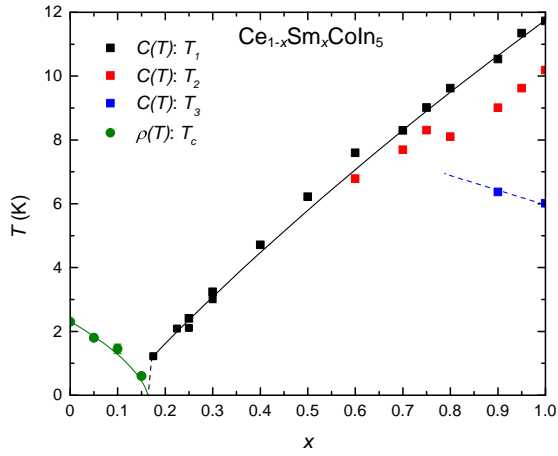
FIG. 4. (Color online) Superconducting critical temperature, T_c , and Sm ordering temperatures T_1 , T_2 , and T_3 (where T_1 is the Néel temperature, T_N ) vs. Sm concentration, x . Lines are guides to the eye.
