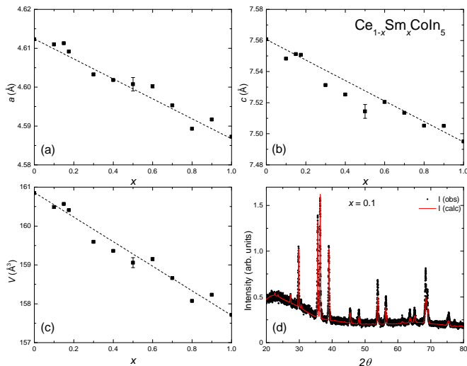
FIG. 2. (Color online) (a), (b) Lattice constants, a and c , plotted as a function of x , respectively. (c) Volume of the unit cell, V , plotted as a function of x . (d) Representative powder x-ray diffraction pattern for an x = 0.1 sample (black circles) and calculated fit from the Rietveld refinement (red line) used to determine the lattice constants a and c . In panels (a)-(c), dashed lines are guides to the eye. Error bars for all concentrations and most are less than or of the order of 10^{-4} Å; however, the x = 0.5 sample has a larger error bar of the order of 10^{-3} Å.
