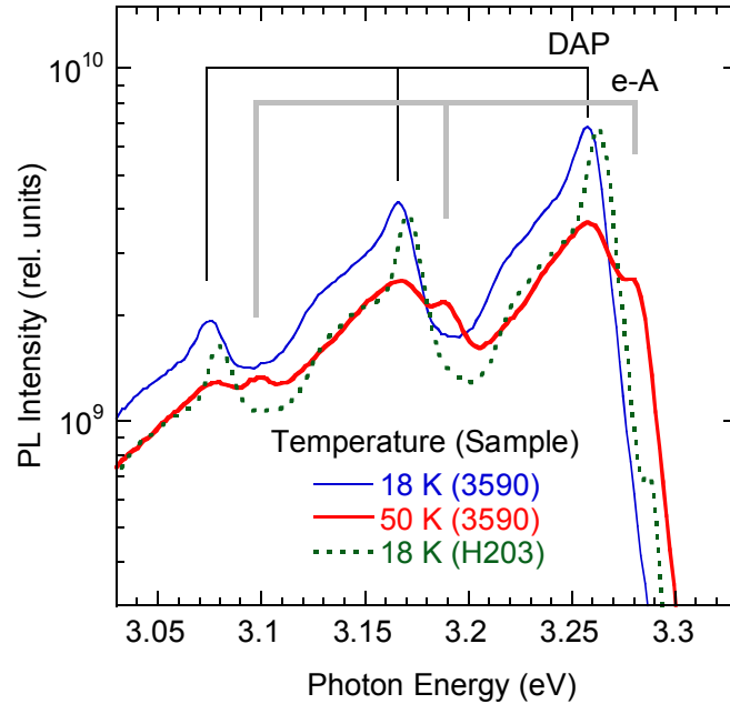
Figure 2 (color online). The UVL band in GaN:Mg (sample 3590) at 18 and 50 K and from undoped GaN sample (H203) at 18 K, all excited with P_{exc} = 0.008 \text{ W/cm}^2 . The UVL band at T = 18 \text{ K} includes the ZPL at 3.253 eV (attributed to DAP-type transitions involving a shallow donor and the shallow \text{Mg}_{\text{Ga}} acceptor) and a set of LO phonon replicas at distances multiple of 91.5 meV from the main peak. At 50 K, a series of (e-A)-type transitions appears, which corresponds to electron transitions from the conduction band to the same shallow acceptor. The spectrum from sample H203 is shifted by 5 meV to lower energies to compensate strain-related blue shift in a relatively thin GaN layer on sapphire substrate, and its intensity is multiplied by a factor of 10 to match the peak intensity of sample 3590.
