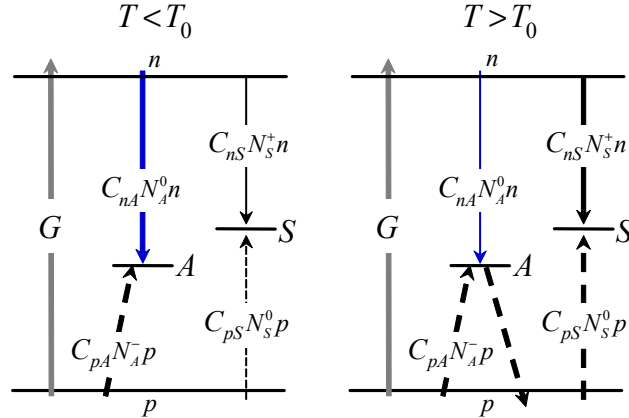
Fig. 9. (Color online) Schematics of transitions explaining abrupt and tunable quenching of PL. Radiative recombination channel A competes with nonradiative recombination channel S for nonequilibrium electrons and holes generated with rate G by a laser. The thick and thin lines indicate high and low transition rates, respectively. The solid and dashed lines show the electron and hole transitions, respectively. The C_{ij} are capture coefficients described in the text. The nonradiative recombination channel is partially blocked at T < T_0 , because deep donors S are saturated with electrons (small N_S^+ ) due to large C_{nS} . The acceptor A is not saturated with holes, because it is partially compensated by shallow donors. The PL efficiency is very high. At T > T_0 , thermal emission of holes from acceptor A to the valence band becomes very efficient. These holes unblock the nonradiative channel, and PL is abruptly quenched in a narrow range of temperatures. The T_0 increases with G , because higher temperature is needed to satisfy parity of thermally emitted and photogenerated holes in the valence band.
