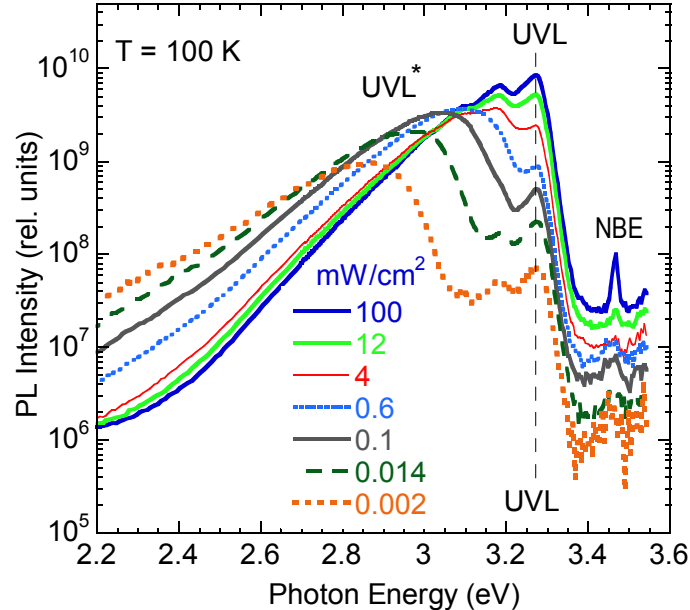
Fig. 6. (color online) PL spectra from GaN:Mg, sample 3589, at T = 100 K and different excitation power densities (indicated with numbers in \text{mW}/\text{cm}^2 ). The PL intensity is divided by the excitation intensity for convenience of comparison. The UVL band does not shift, while the UVL* band shifts monotonously to higher energies with increasing excitation intensity.
