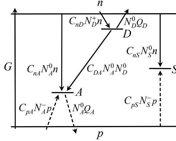
Fig. 15 (color online). Band diagram of GaN:Mg. The solid arrows show transitions of electrons, and the dashed arrows show transitions of holes. A is the Mg Ga acceptor, D is a shallow donor, and S is a nonradiative deep acceptor. Model parameters are defined in the text.
