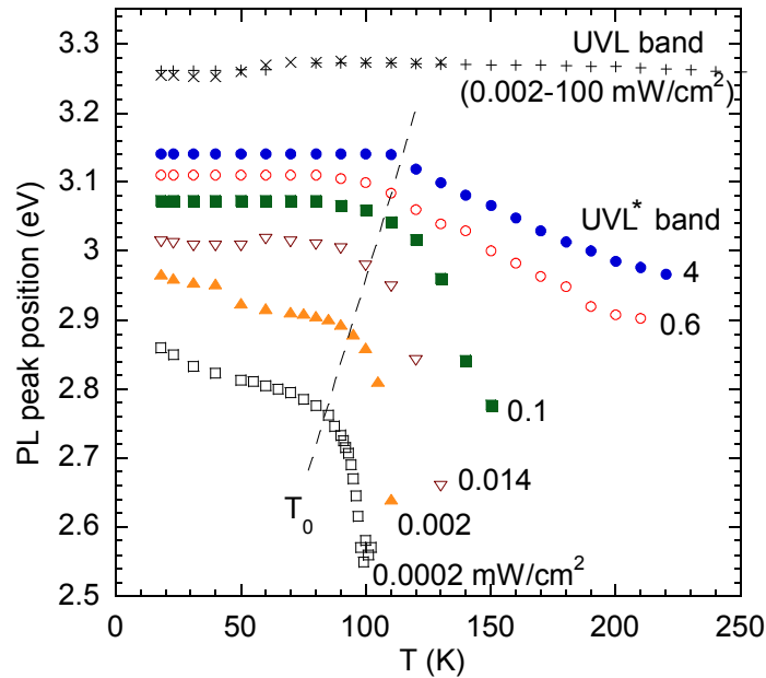
Fig. 7 (color online). Peak position of the UVL and UVL* bands in GaN:Mg (sample 3589) as a function of temperature at different P_{exc} (indicated with numbers in mW/cm 2 ). T_0 is the characteristic temperature at which the rate of the shift abruptly changes.
