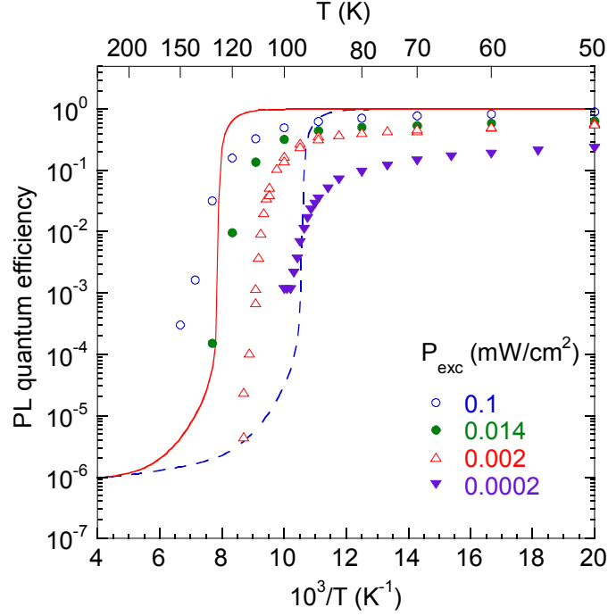
Fig. 8. (Color online) Temperature dependence of the UVL* quantum efficiency at different excitation intensities for sample 3589. The symbols are experimental data (multiplied by a factor of 5 for convenience of comparison). The lines are from numerical solution of Eqs. (A1)-(A9) in Appendix with the following parameters: N_A = 1.5 \times 10^{18} , N_S = 8 \times 10^{17} , N_D = 5 \times 10^{17} (all in \text{cm}^{-3} ); C_{pA} = 5 \times 10^{-7} , C_{pS} = 1 \times 10^{-10} , C_{nA} = 3.2 \times 10^{-12} , C_{DA} = 1 \times 10^{-13} , C_{nD} = 1 \times 10^{-8} , C_{nS} = 1 \times 10^{-6} (all in \text{cm}^3/\text{s} ); E_D = 20 meV, E_A = 185 meV; P_{exc} = 0.1 mW/cm 2 (solid line), and 0.0002 mW/cm 2 (dashed line).
