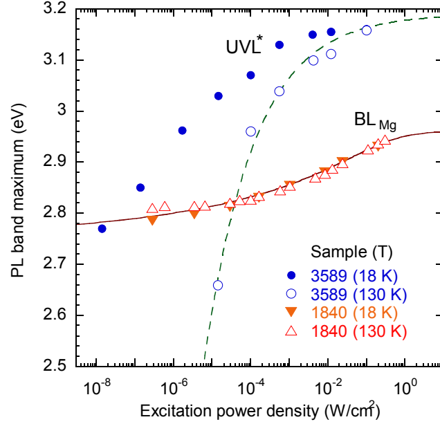
Fig. 13 (color online). Shift of PL band maxima with excitation intensity at T = 18 and 130 K. The BL_{Mg} band in sample 1840 and the UVL^* band in sample 3589. The solid line is calculated using Eq. (6) with D = 100 \text{ W}/(\text{eV cm}^2)^2 , E_B = 0.48 \text{ eV} , and \hbar\omega_\infty = 2.72 \text{ eV} . The dashed line is calculated using Eq. (9) with the following parameters: \hbar\omega_{max} = 3.19 \text{ eV} , N_A = 1.5 \times 10^{18} \text{ cm}^{-3} , and p = 3 \times 10^{19} P_{exc}[\text{W}/\text{cm}^2] \text{ cm}^{-3} .
