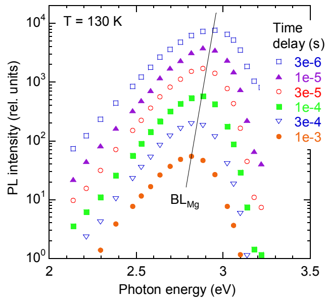
Fig. 12 (color online). Evolution of PL spectrum with time after a laser pulse at 130 K for HVPE GaN:Mg sample 1840.
