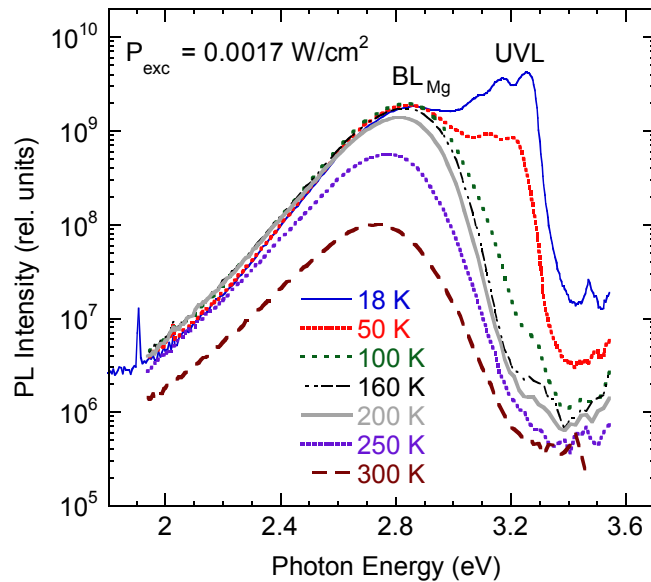
Fig. 10. (color online) Evolution of the PL spectrum with temperature for HVPE GaN:Mg, sample 1840.
