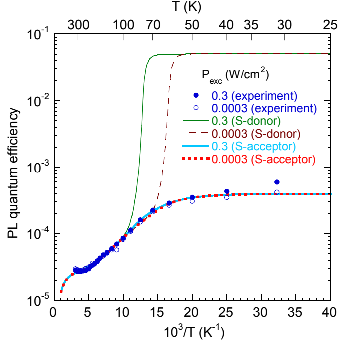
Fig. 17 (color online). Temperature dependence of the quantum efficiency of the UVL band in p -type GaN:Mg. The symbols are experimental data for sample 9600A at P_{exc} = 0.0003 and 0.3 \text{ W/cm}^2 . The lines are calculated using Eqs. (A1)-(A9) with parameters listed in Table II. Thick dotted and solid lines are calculated for the case of S center as a deep acceptor, and thin dashed and solid lines are calculated for the case of S center as a deep donor.
