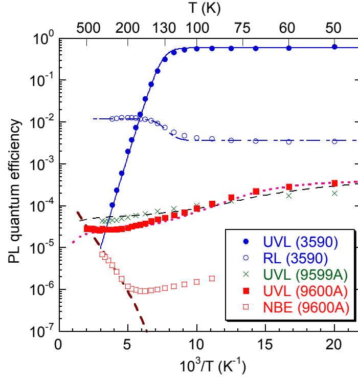
Fig. 3 (color online). Temperature dependence of PL quantum efficiency for selected PL bands in GaN:Mg samples. The solid line for sample 3590 is calculated using Eqs. (1) and (2) with the following parameters: \eta_0 = 0.6 , \tau_0 = 20 \mu\text{s} , C_{pA} = 0.5 \times 10^{-6} \text{ cm}^3/\text{s} , N_v = 3.2 \times 10^{15} T^{3/2} \text{ cm}^{-3} , E_A = 185 \text{ meV} . Other lines are from numerical solutions of Eqs (A1)-(A9) in Appendix with parameters given in Table II.
