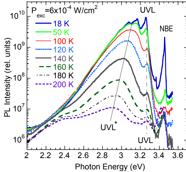
Fig. 5 (color online). Evolution of the PL spectrum with temperature for HVPE GaN:Mg, sample 3589. The UVL band does not shift, while the UVL* band monotonously shifts to lower energies with increasing temperature.
