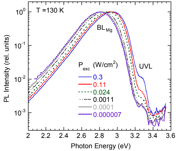
Fig. 11 (color online). Normalized PL spectra at 130 K and different excitation intensities for HVPE GaN:Mg sample 1840.
