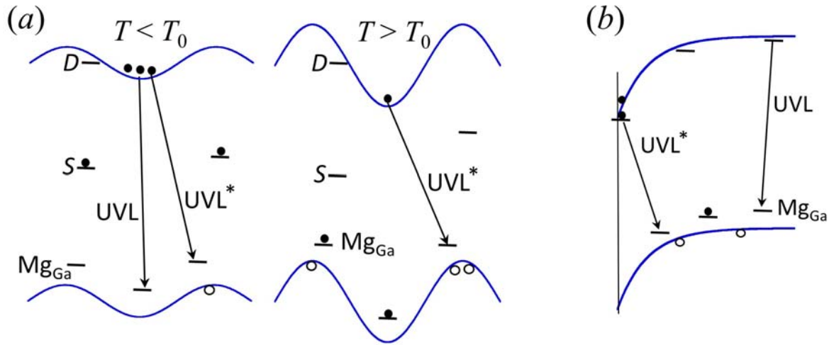
Fig. 14 (color online). Schematics of GaN bandgap and electron transitions resulting in the UVL and UVL^* bands. (a) The potential fluctuations cause diagonal transitions. At T < T_0 , nonradiative deep donors S are saturated with photogenerated electrons, and the Mg_{Ga} acceptors are saturated with holes. Under illumination, electrons accumulate in the conduction band because the nonradiative recombination channel is blocked and radiative transitions are very slow. Potential fluctuations are screened by accumulated electrons, and radiative transitions are almost vertical. At T > T_0 , holes are emitted from the Mg_{Ga} to the valence band, the concentration of charged donors and acceptors sharply increases, while the concentration of photogenerated free electrons abruptly drops. This results in large unscreened potential fluctuations and diagonal radiative transitions. (b) The downward band bending near the sample surface causes diagonal transitions. Transitions of electrons from the conduction band (or shallow donors) at the surface to the Mg_{Ga} acceptors in the depletion region are responsible for the UVL^* band, whereas such transitions in the bulk are responsible for the UVL band.
