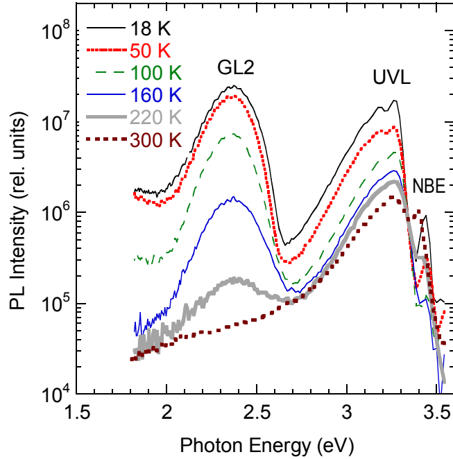
Fig. 4 (color online). Evolution of the PL spectrum with temperature for MBE GaN:Mg sample 9599A. P_{exc} = 0.001 \text{ W/cm}^2 .
