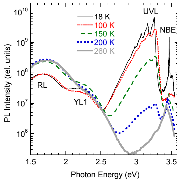
Fig. 1. (color online) Evolution of the PL spectrum with temperature for HVPE GaN:Mg sample 3590.
