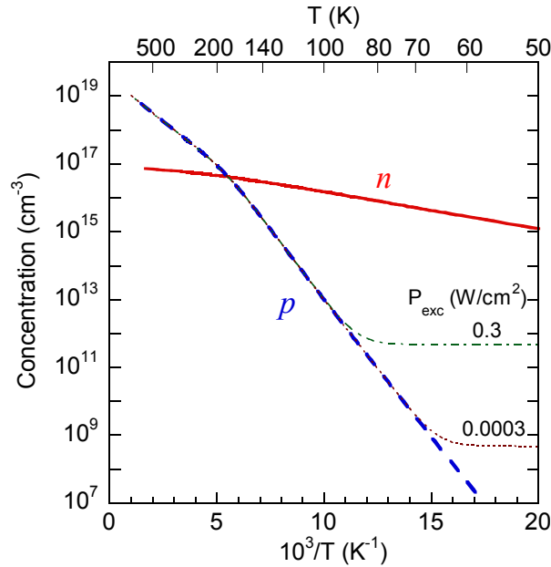
Fig. 16 (color online). Temperature dependences of the concentrations of free electrons in n -type GaN:Mg (sample 3590) and free holes in p -type GaN:Mg (sample 9600A). The thick solid curve for n is calculated using Eq. (A10). The thick dashed curve for p is calculated using Eq. (A11). The thin dash-dotted and dotted curves for p are from numerical solutions of Eqs. (A1)-(A9) for P_{\text{exc}} = 0.3 and 0.0003 \text{W}/\text{cm}^2 , respectively. The parameters are given in Table II.
