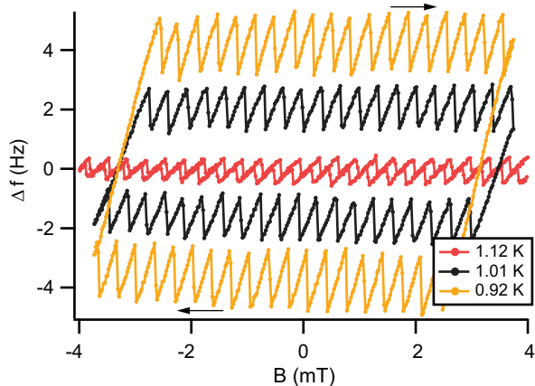
FIG. 9. Field sweeps of obtained for Ring 1, with the magnetic tip positioned 600 nm above the center of the ring. The arrows indicate the direction of the field sweep.
