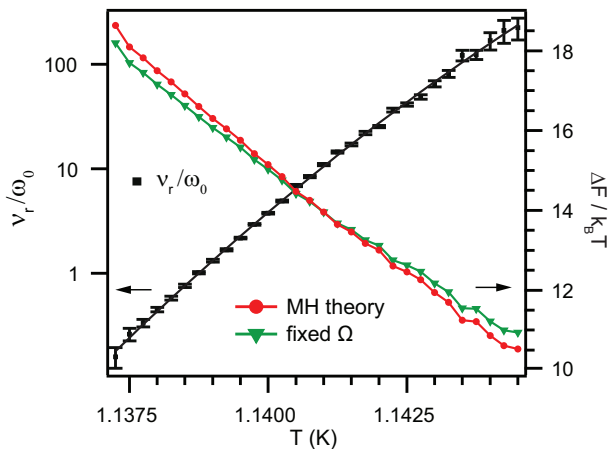
FIG. 5. (Left axis) \nu_r/\omega_0 determined from the data shown in Fig. 3(b). (Right axis) Phase slip energy barrier \Delta F derived from \nu_r . Solid circles correspond to \Delta F derived using McCumber-Halperin expression for attempt frequency \Omega , solid triangles correspond to constant \Omega = 3 \times 10^{11} \text{ s}^{-1} .
