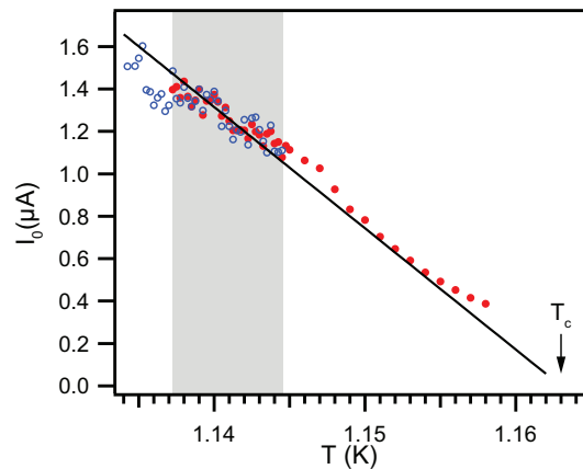
FIG. 12. Plot of I_0(T) derived from \Delta\gamma (empty circles) and \Delta\omega (solid circles). Solid line corresponds to the fit of I_0 to the expected temperature dependence I_0(T) \propto 1 - T/T_c . Shaded region marks the temperature range where \nu_r(T) was extracted from data; points at other temperatures were calculated with extrapolated \nu_r and were not used for the fit.
