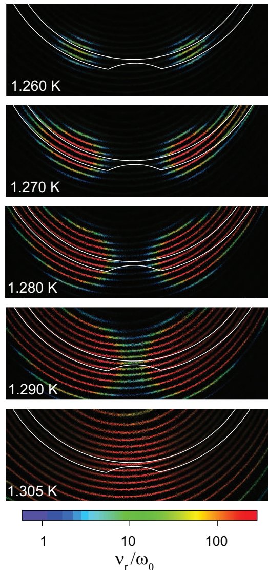
FIG. 7. (Color online) Temperature evolution of \nu_r taken for the rectangular region indicated in Fig. 6(d). Measurements were performed at a tip-surface separation of 550 \text{ nm} .
