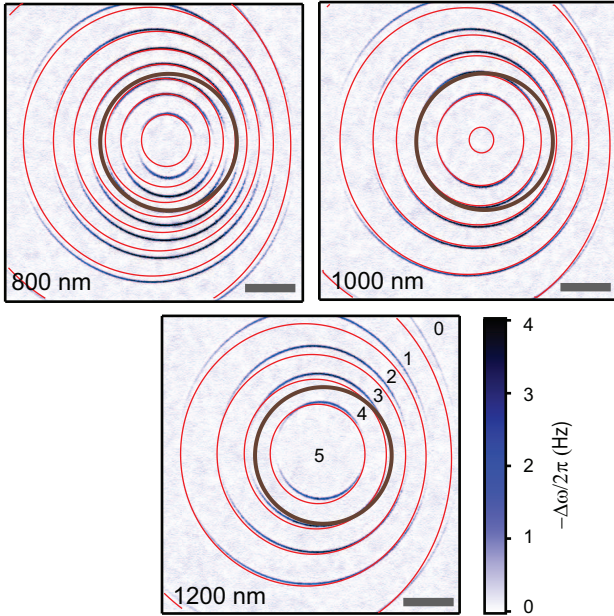
FIG. 11. Comparison of the fluxoid transitions calculated from the 3D model of the tip (red) to the experimental data. The textcolor[rgb]0,0,1brown circle represent the location of the ring. Calculated fluxoid states are labeled with the phase winding numbers on the image taken at tip-surface separation of 1200 \text{ nm} . All scale bars correspond to 1 \mu\text{m} .
