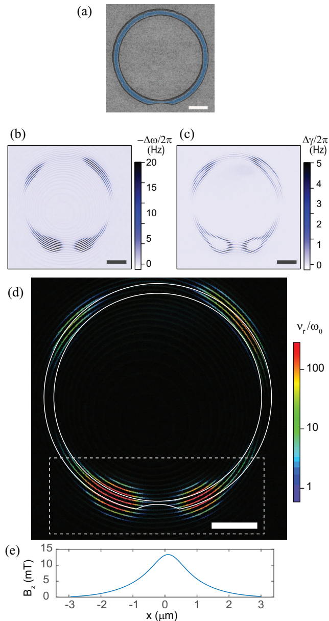
FIG. 6. (Color online) Stochastic resonance imaging of a thin ring containing a constriction. The stripes in the images correspond to individual fluxoid transitions. (a) An SEM image of Ring 2. The ring has a radius R = 2.38 \mu\text{m} , a width w = 200 \text{ nm} and a 1.22\text{-}\mu\text{m} long constriction, having a minimum width of 60 \text{ nm} . (b) Frequency shift \Delta\omega . (c) Dissipation shift \Delta\gamma (d) Phase slip rate \nu_r . The solid white lines indicate the outline of Ring 2. The dashed line marks the rectangular region shown in Fig. 7. (e) Cross section of the magnetic field distribution on the surface. Measurements were performed at 1.280 \text{ K} for a tip-surface separation of 650 \text{ nm} . All scale bars are 1 \mu\text{m} .
