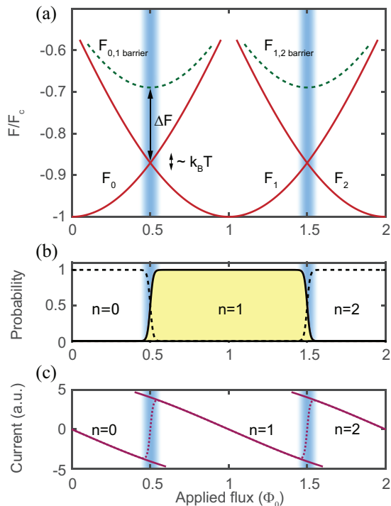
FIG. 2. Energy, occupation probability and supercurrent corresponding to the n = 0 to n = 2 fluxoid states. (a) Schematic of fluxoid state energies: solid lines represent energies of the fluxoid states. The dashed lines represent the energy barriers between adjacent fluxoid states. (b) Equilibrium occupation probability for different fluxoid states. (c) The solid lines represent the piecewise-continuous circulating current corresponding to a particular fluxoid state. The dashed line represents the thermal average of the current. Vertical blue bands on all panels mark the regions, where the energy separation between the states is of the order \leq k_B T .
