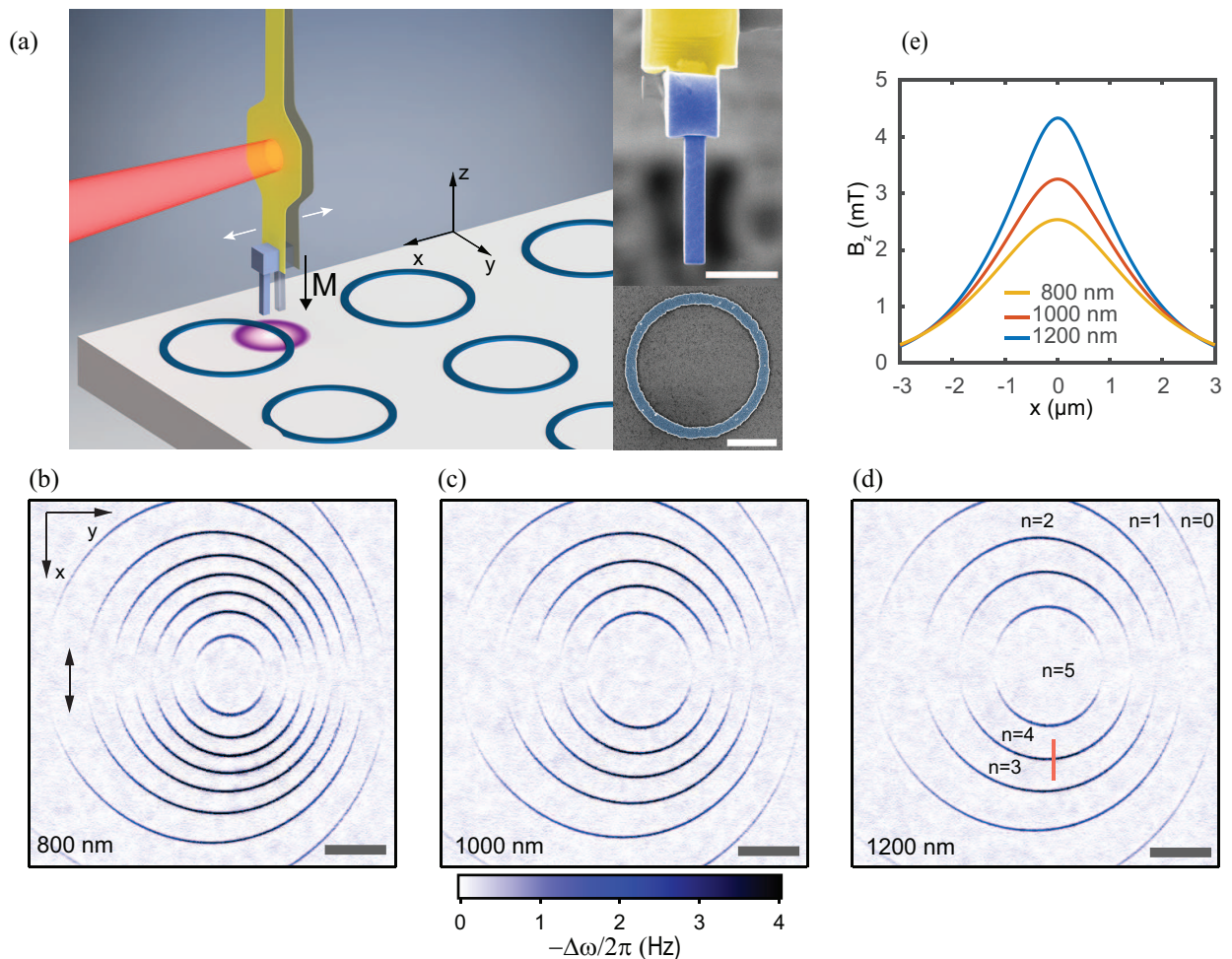
FIG. 1. (a) Schematic of the experimental setup showing the cantilever positioned over an Al ring. Top inset shows an SEM micrograph of the FIB-shaped \text{SmCo}_5 magnetic particle attached to the tip of the cantilever. The magnetic moment of the particle is oriented perpendicular to the surface, in the z -direction, and produces a highly inhomogeneous magnetic field in its vicinity (illustrated as the disk shaped region near the tip.) The bottom inset displays an SEM micrograph of Ring 1; (b-d) The \Phi_0 -MFM images show the frequency shift of the cantilever. Dark circular contours correspond to transitions between fluxoid states. In the regions between successive transitions, the winding number n of the ring changes by 1. The images were obtained with a fixed tip-surface separation distance, indicated in the bottom-left-hand corner of each panel. The double arrows in (b) indicate the oscillation direction of the cantilever. Change in the frequency and dissipation of the cantilever across the n = 3 to n = 4 transition, indicated by the red line segment in (d), are presented in detail in Fig. 3. (e) Cross section of the magnetic field distribution on the sample surface for various tip-surface heights. The field distributions are estimated from the pattern of fluxoid transitions observed in (b-d). All scale bars correspond to 1 \mu\text{m} .
