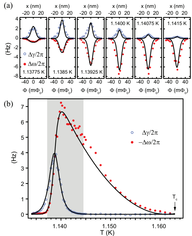
FIG. 3. Temperature dependence of the signal for the n = 3 to n = 4 transition at the location indicated in Fig. 1(d). (a) Line scans across the transition region were obtained at the temperatures indicated on each panel. (b) Plot of the peak frequency (solid circles) and dissipation shift (open circles) as a function of temperature. Solid lines on (a) and (b) represent the curves calculated using the stochastic resonance model for TAPS (see Section III C). Shaded region on (b) marks the temperature range for which the relaxation rate \nu_r was determined.
