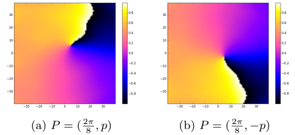
FIG. 11: \arg \nu_P^E(\mathbf{r}) for canted PDW in unit of \pi .
