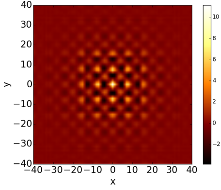
(a) Real space pattern of magnetic moment M(\mathbf{r}) in unit of 10^{-3}\mu_B .
