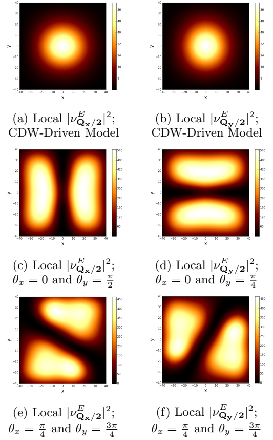
FIG. 7: |\nu_{\mathbf{Q}_a/2}^E|^2 from CDW-Driven and PDW-Driven Models. (a) and (b) are from a CDW-Driven model; Others are from PDW-Driven models. E = 30 meV.
