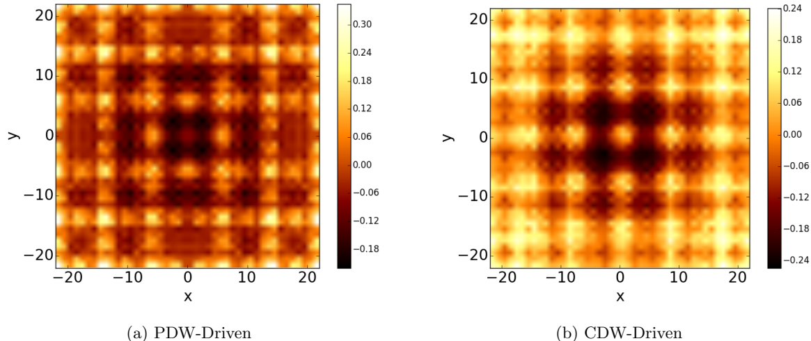
FIG. 3: Real Space Plot of on site LDoS \nu^E(\mathbf{r}) at E = 30\text{meV} for PDW-Driven and CDW-Driven model.
