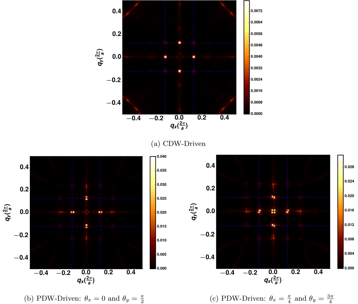
FIG. 4: |\tilde{\nu}^E(q)| with E = 30 meV for PDW-Driven and CDW-Driven Models.
