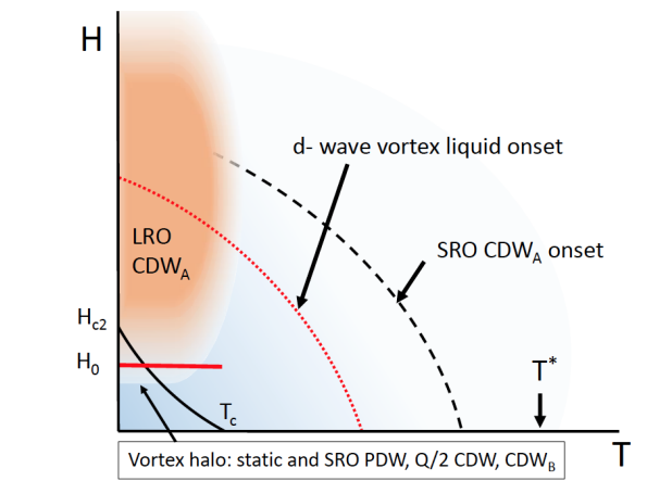
FIG. 13: H - T Phase Diagram for an underdoped Cuprate. The light blue shading indicates that a fluctuating PDW is pervasive over a large segment of the H - T plane for underdoped Cuprates. Dashed line indicates the onset of short range ordered CDW at wave-vector Q . It is a subsidiary order of the PDW which we refer to as CDW_A . Solid red line marks the magnetic field H_0 as defined in Eq.(14) in terms of the coherence length \xi_P of the PDW which marks the size of the vortex halo. It is closely related to the field H_{c2} which marks the onset of a vortex solid phase and LRO superconductivity. Within this phase and inside the vortex halo we expect the pinned static PDW, Q/2 CDW as well as its harmonic, a wave-vector Q CDW which we refer to as CDW_B . The CDW_B short range order state may extend to higher magnetic field much beyond H_{c2} . The dotted red line indicates the onset of a vortex liquid phase. The brown area indicates the appearance of long range ordered type A CDW with wave-vector Q .
