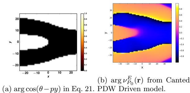
FIG. 12: Visualization of \arg \nu_{P_0}^E(\mathbf{r}) for canted PDW Driven model. P_0 = (\frac{2\pi}{8}, 0) and shifted-momentum is p = 0.03 * 2\pi .
