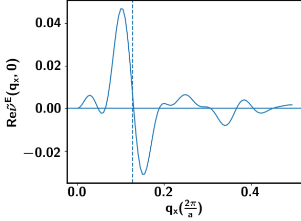
FIG. 5: Re\tilde{\nu}^E(q_x, 0) for PDW-Driven model with \theta_x = 0 and \theta_y = \frac{\pi}{2} ; There is a clear sign change at q_x = \frac{1}{8}\frac{2\pi}{a} .
