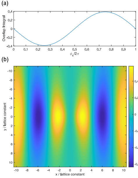
FIG. 2: (a) Overlap integral \int \Delta_d^*(\mathbf{r})\Delta_{\text{PDW}}(\mathbf{r})d^2\mathbf{r} as a function of \phi_x , for \theta_x = 0 . We have set their maximum amplitude to 1 for both \Delta_d(\mathbf{r}) and \Delta_{\text{PDW}}(\mathbf{r}) , and we normalize the integral by the overlap of PDW with itself inside the vortex core of radius 3a . \phi_x is pinned to 3\pi/2 . The large overlap implies the real-space pattern of PDW matches the pattern of d wave vortex core almost perfectly at \phi_x = 3\pi/2 — its amplitude is reduced only because d wave amplitude is reduced in the vortex core. (b) The integrand \Delta_d^*(\mathbf{r})\Delta_{\text{PDW}}(\mathbf{r}) as a function of \mathbf{r} near vortex core, for \phi_x = 3\pi/2 , \theta_x = 0 .
