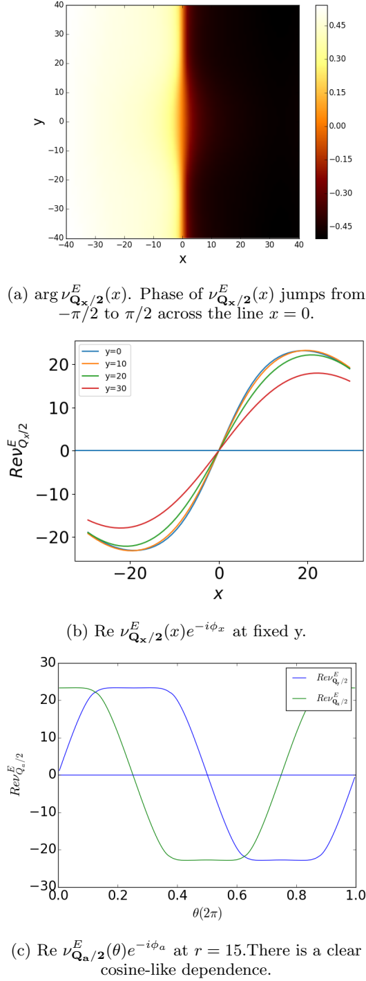
FIG. 6: \nu_{\mathbf{Q}_a/2}^E for PDW-Driven model with \theta_x = 0 and \theta_y = \frac{\pi}{2} .
