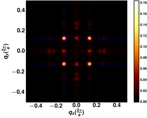
(b) Magnetic moment M(q) in momentum space.
