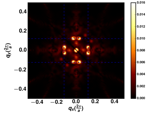
FIG. 10: |\tilde{\nu}^E(\mathbf{q})| for canted PDW with shifted momentum p = 0.03 * 2\pi/a . Phase of PDW is \theta_x = 0 and \theta_y = \frac{\pi}{2} .
