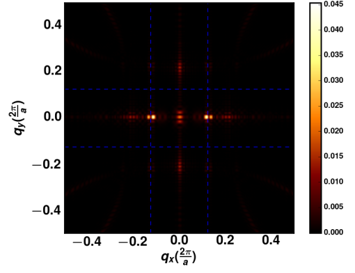
FIG. 9: |\tilde{\nu}^E(q)| for unidirectional PDW with phase \theta_x = 0 .
