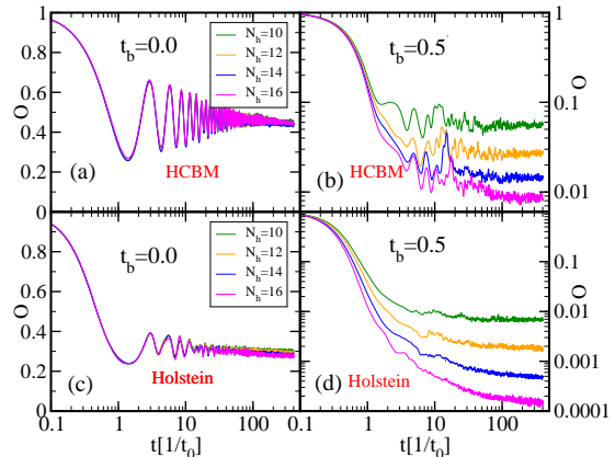
Figure 6. \mathcal{O}(t) as given in Eq. (5) of the main text using different system sizes as given by N_h , for the HCBM in (a) and (b) and the Holstein model in (c) and (d). In all cases we have used \omega = g = 1 , W = 12 .
