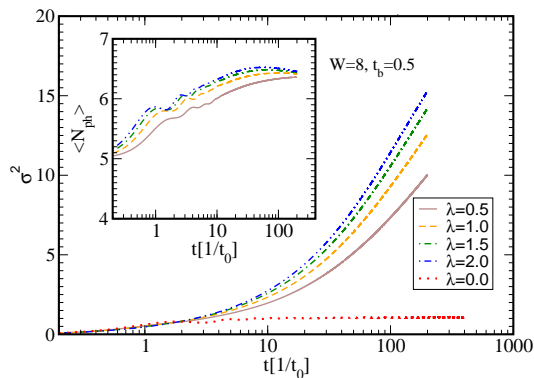
Figure 5. \sigma^2 vs. t for the Holstein model for different coupling strengths \lambda . Inset represents \langle N_{\text{ph}} \rangle(t) . In both cases we have used \omega = 1 , t_b = 0.5 , and W = 8 .
