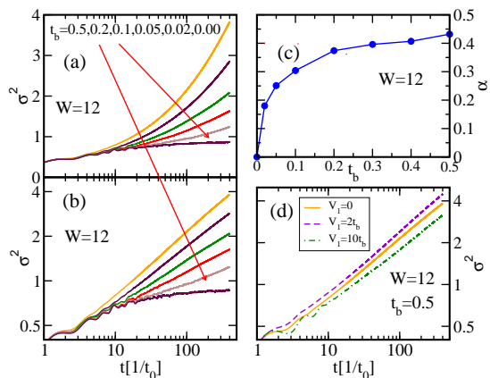
Figure 1. The mean square deviation \sigma^2(t) for different values of t_b for the case when the particle is coupled to HCB's using a) semi-log plot and b) log-log plot; c) fitting exponents \alpha vs. t_b extracted from \sigma^2(t) = At^\alpha . Fitting was performed in the long-time-limit; d) log-log plot of \sigma^2(t) of the HCB model using different values of nearest and next nearest interaction V_1 and V_2 , respectively. In all cases we have used \omega = g = 1 , W = 12 , and N_h = 20 .
