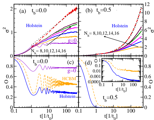
Figure 3. a) and b) \sigma^2(t) of the Holstein model for different sizes of the Hilbert spaces generated by N_h and W = 12 . The cases with no dispersion, t_b = 0 , are presented in a) while results for t_b = 0.5 are shown in b). Dashed (red) lines represent results after finite-size scaling analysis. Dotted line in a) represents a fit to the form \sigma^2(t) = A + B \log(t) . Dotted line in b) represent fit to the form \sigma^2(t) = At^\alpha . Overlaps \mathcal{O} are shown in c) ( t_b = 0 ) and d) ( t_b = 0.5 ) for the Holstein model with full lines and the HCBM with dashed lines. Thin lines (violet in colour) in a) and c) represent evolution of \sigma^2(t) and \mathcal{O} , respectively, for a free particle, i.e. at g = 0 , that undergoes Anderson’s localization. The inset in d) shows the same data as in d) but using log-log scale. Other parameters of the model were in all cases \omega = g = 1 , W = 12 , and V_1 = V_2 = 0 .
