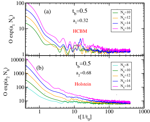
Figure 7. Scaled survival probability \mathcal{O}(t) \exp(a_i N_h) for the case when t_b = 0.5 for the two models as indicated in the figure. In both cases we have used \omega = g = 1 , W = 12 .
