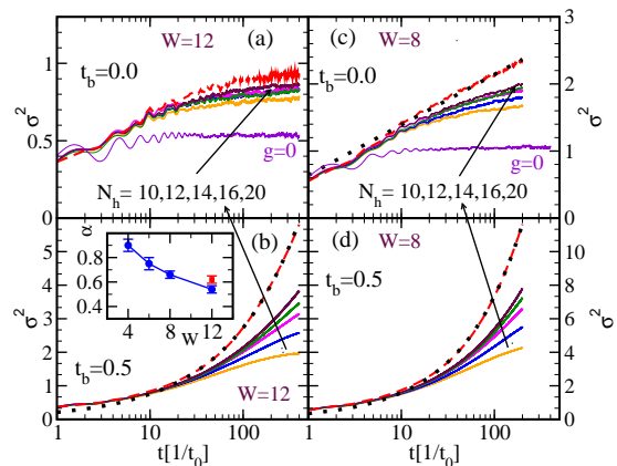
Figure 2. Semi-log plots of \sigma^2(t) of the HCB model for different sizes of the Hilbert spaces generated by N_h . Cases with no dispersion, t_b = 0 , are presented in a) and c) for two distinct values of disorder W = 12 and 8 , respectively. Results for t_b = 0.5 are shown as well for two distinct values of W in b) and d). Note also substantially different scales used to present results with or without dispersion. Dashed (red) lines represent results after finite-size scaling analysis. Dotted line in c) represents a fit to the form \sigma^2(t) = A + B \log(t) . Dotted lines in b) and d) represent fit to the form \sigma^2(t) = At^\alpha . Thin (violet in colour) line in a) and c) represents evolution of \sigma^2(t) for a free particle, i.e. g = 0 , that is subject to Anderson's localization. Inset in b) displays exponents \alpha (circles) extracted from finite-size scaled results at different values of disorder W . A singular square represents result for the Holstein model with identical parameters as the HCB one. Other parameters of the model were \omega = g = 1 and V_1 = V_2 = 0 .
