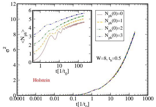
Figure 4. \sigma^2 vs. t for the Holstein model. N_{\text{ph}}(0) the number of phonon excitations at t = 0 . Inset represents \langle N_{\text{ph}} \rangle(t) . In both cases we have used \omega = g = 1 , t_b = 0.5 , and W = 8 .
