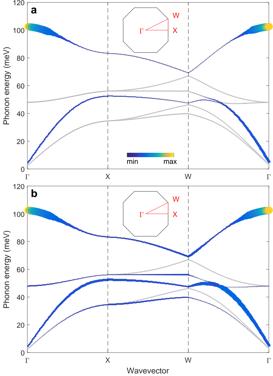
FIG. 8: Contribution of phonon modes to electron energy loss probability P(\hbar\omega) of Eq. (10). The Brillouin zone and the path of the selected wavevectors are shown in the insets. We plot the contributions |\mathcal{F}_\lambda(\mathbf{q})|^2 to P(\hbar\omega_{\mathbf{q}\lambda}) , see Eq. (10), using impact parameters of (a) 0.5\times and (b) 0.25\times AC. For better visibility, the sizes of the largest dots have been set to a maximum value.
