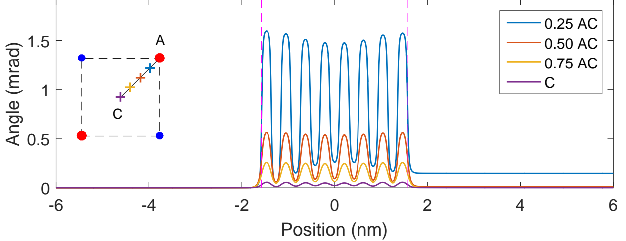
FIG. 3: Deflection angle of the electron velocity with respect to the forward direction while passing through a n = 8 MgO nanocube. We show the deflection angles in mrad for different impact parameters, corresponding to position C, as well as 75%, 50% and 25% of direction AC shown in the inset. The vertical dashed lines indicate the cube boundaries.
