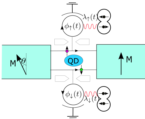
FIG. 2. (Color online) Schematic plot of spin-resolved waiting time clock. A quantum spin Hall QD is embedded between two ferromagnetic electrodes. Spin- \sigma (spin-up in the plot) electrons can tunnel into the capacitor through a quantum point contact and then interacts with a two-level system. Spin- \sigma electron waiting times can be obtained from monitoring the two-level system by changing interaction strength \lambda_\sigma(t) .
