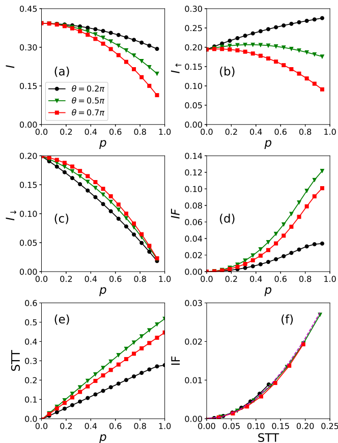
FIG. 7. (Color online) Charge current [panel (a)], spin up current I_{R\uparrow} [panel (b)], spin down current I_{R\downarrow} [panel (c)], influence degree [panel (d)], and STT [panel (e)] versus spin polarization p with different noncollinear angles \theta are plotted. Influence degree versus STT are plotted in panel (f) with the quadratic fitting IF = 0.51 * (STT)^2 shown in dashed lines.
