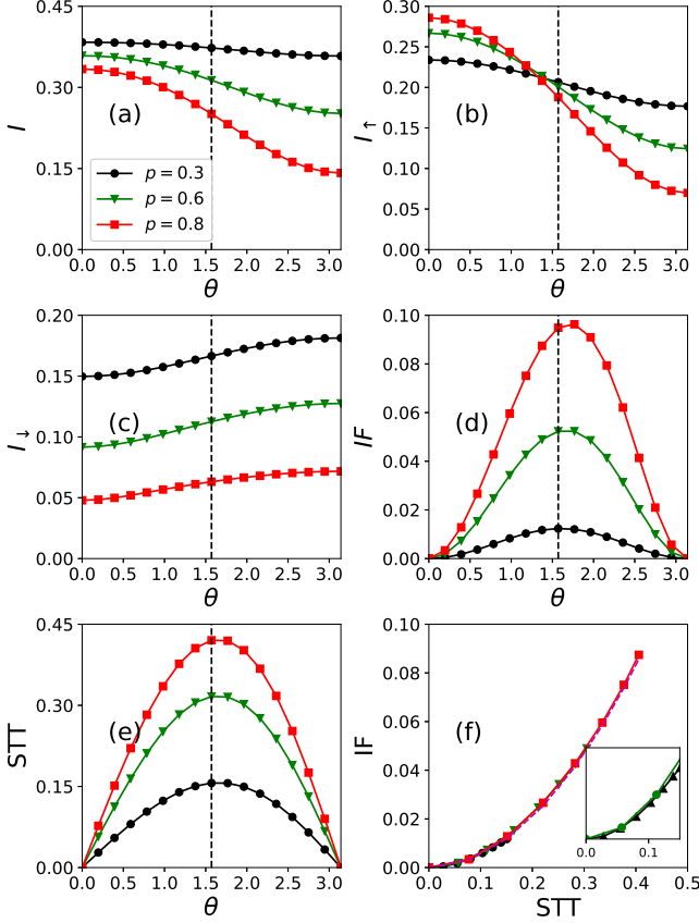
FIG. 4. (Color online) Charge current [panel (a)], spin up current I_{R\uparrow} [panel (b)], spin down current I_{R\downarrow} [panel (c)], influence degree [panel (d)], and STT [panel (e)] versus non-collinear angle \theta with different spin polarization p are plotted. Influence degree versus STT are plotted in panel (f) with the quadratic fitting IF = 0.51 * (STT)^2 shown in dashed lines.
